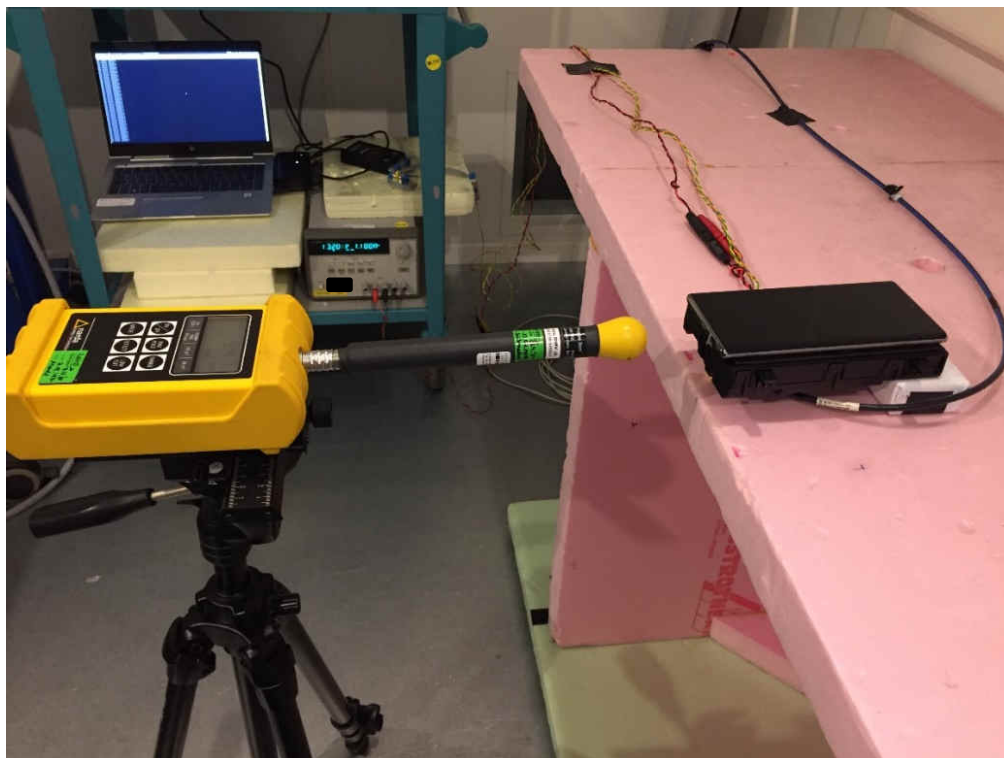
Worst case position H-field probe (Coil 2, Pos. B, 6 cm)
