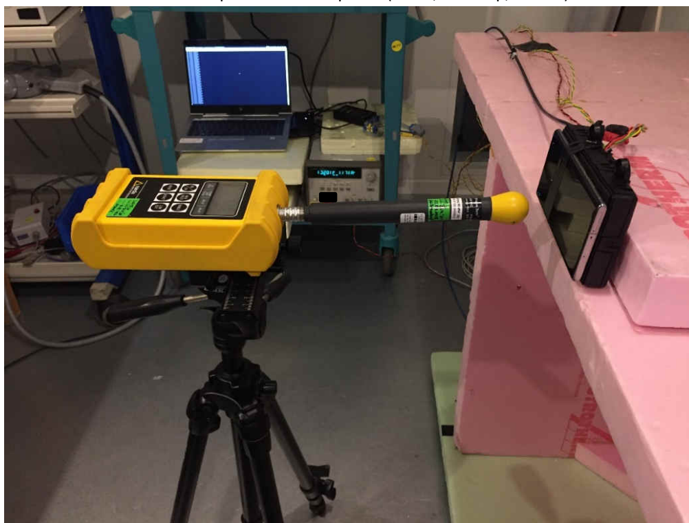
Worst case position H-field probe (Coil 1, Pos. Top, 5.3 cm)
