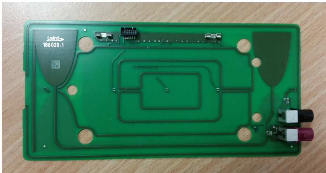
Top view of antenna board with additional connector for external NFC antenna:
