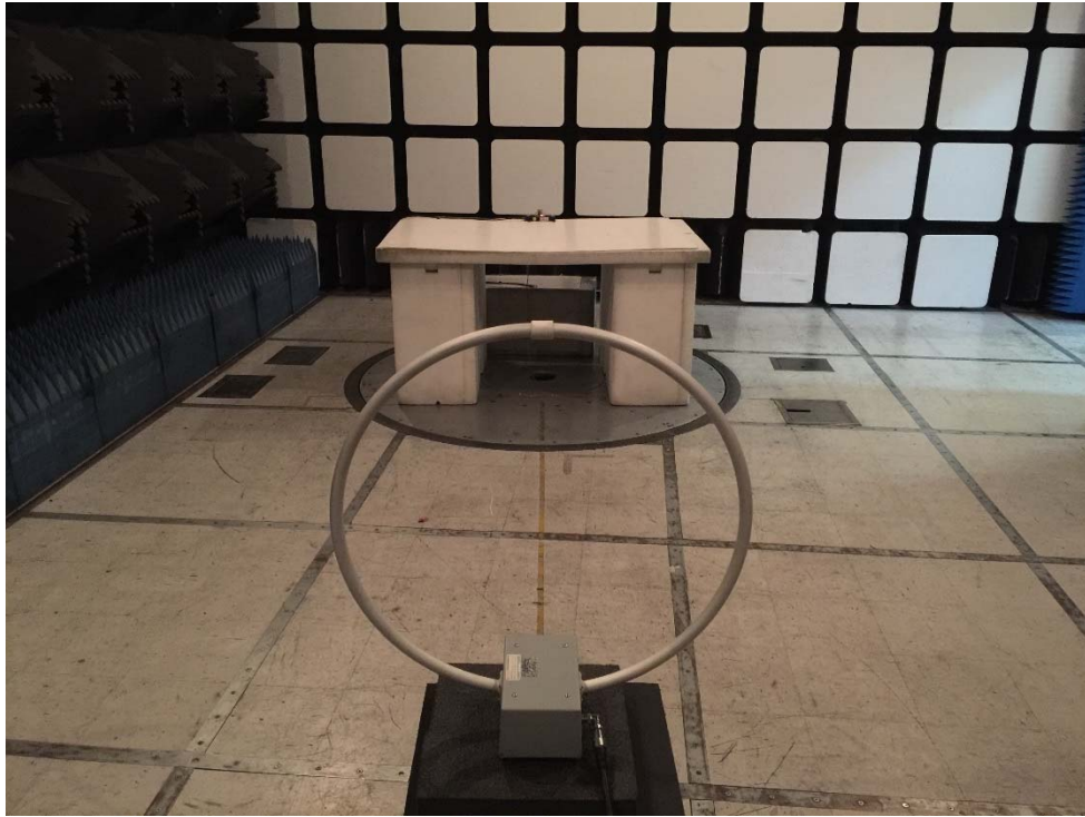
RSS 216 Setup
