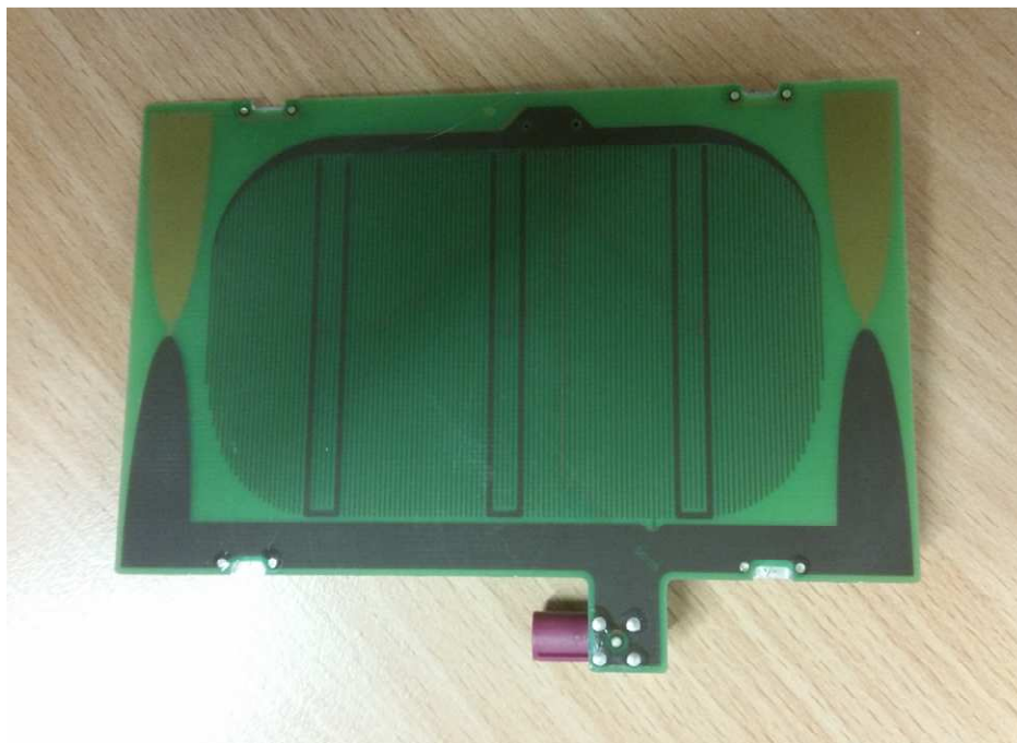
Antenna Board bottom view
