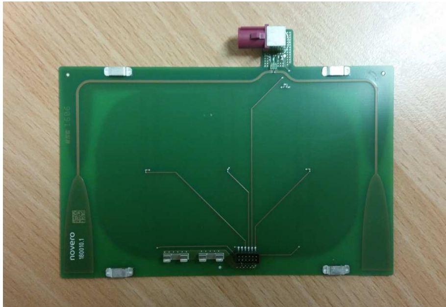
Top view antenna board with Fakra antenna connector
