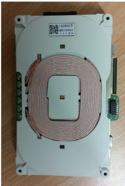
Top view antenna board with Fakra antenna connector
