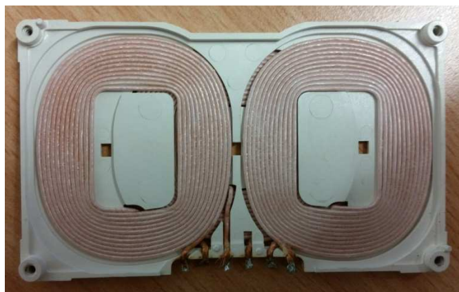
Bottom view coil module
