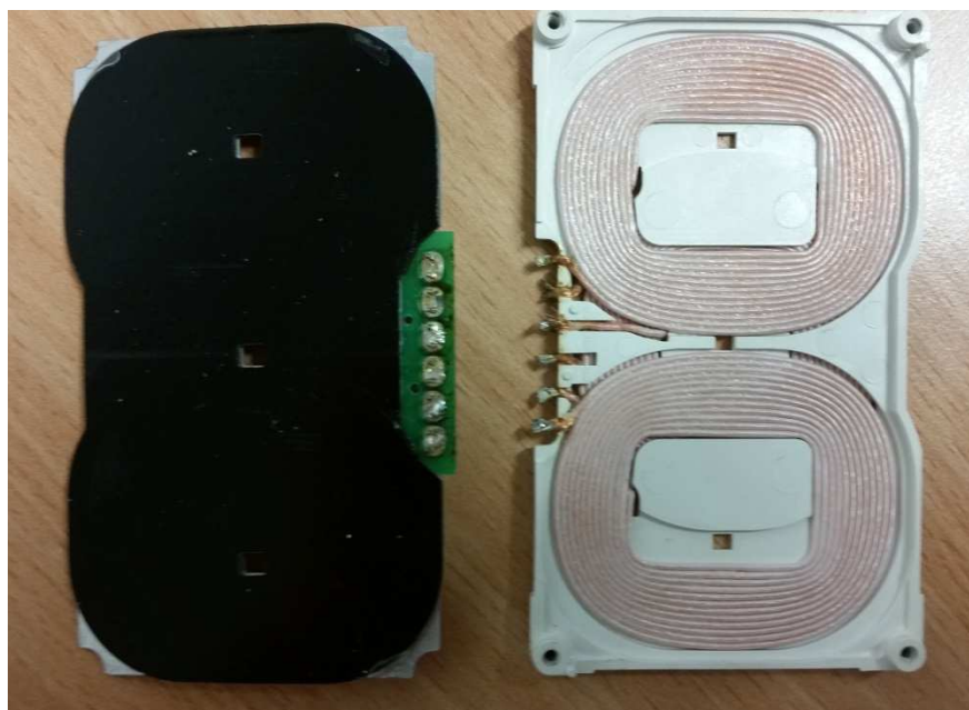
Inner view coil module with 2 coils
