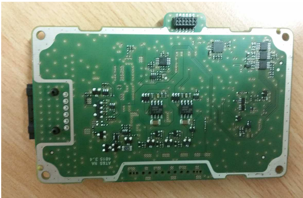
Bottom View Main Board
