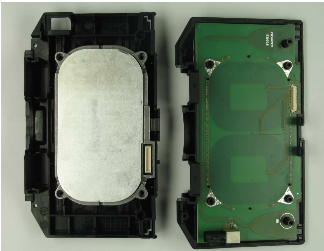
Inside view with PWB Coil Board
