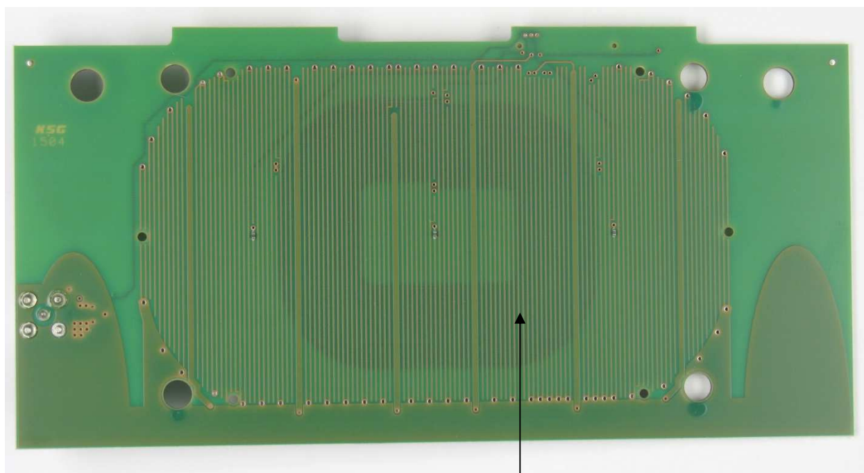
Bottom view PWB coil board with first primary coil
