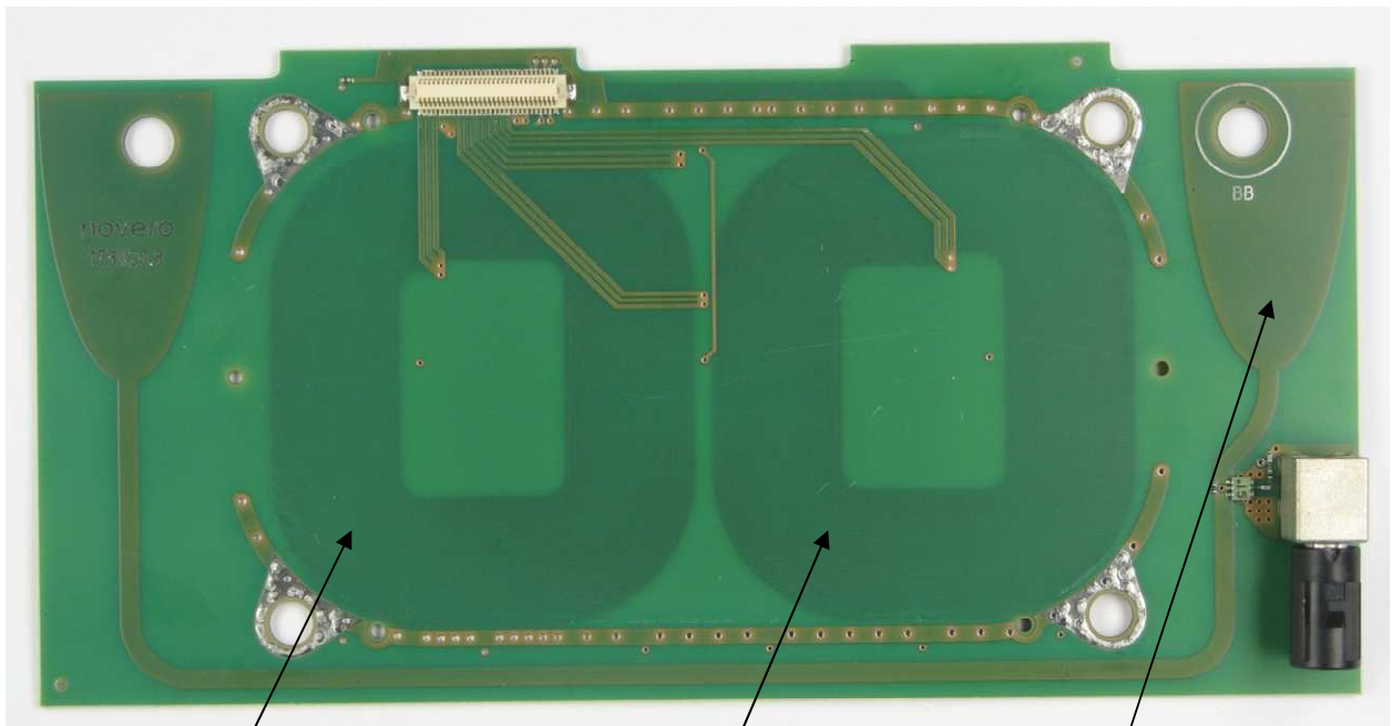
Top view of PWB coil board with second primary coil and third primary coil and passive antenna coupling
