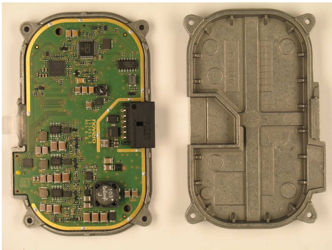
Top view of PWB main
