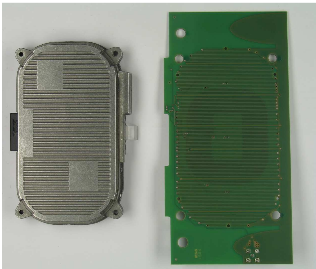
Cooling element and PWB coil board
