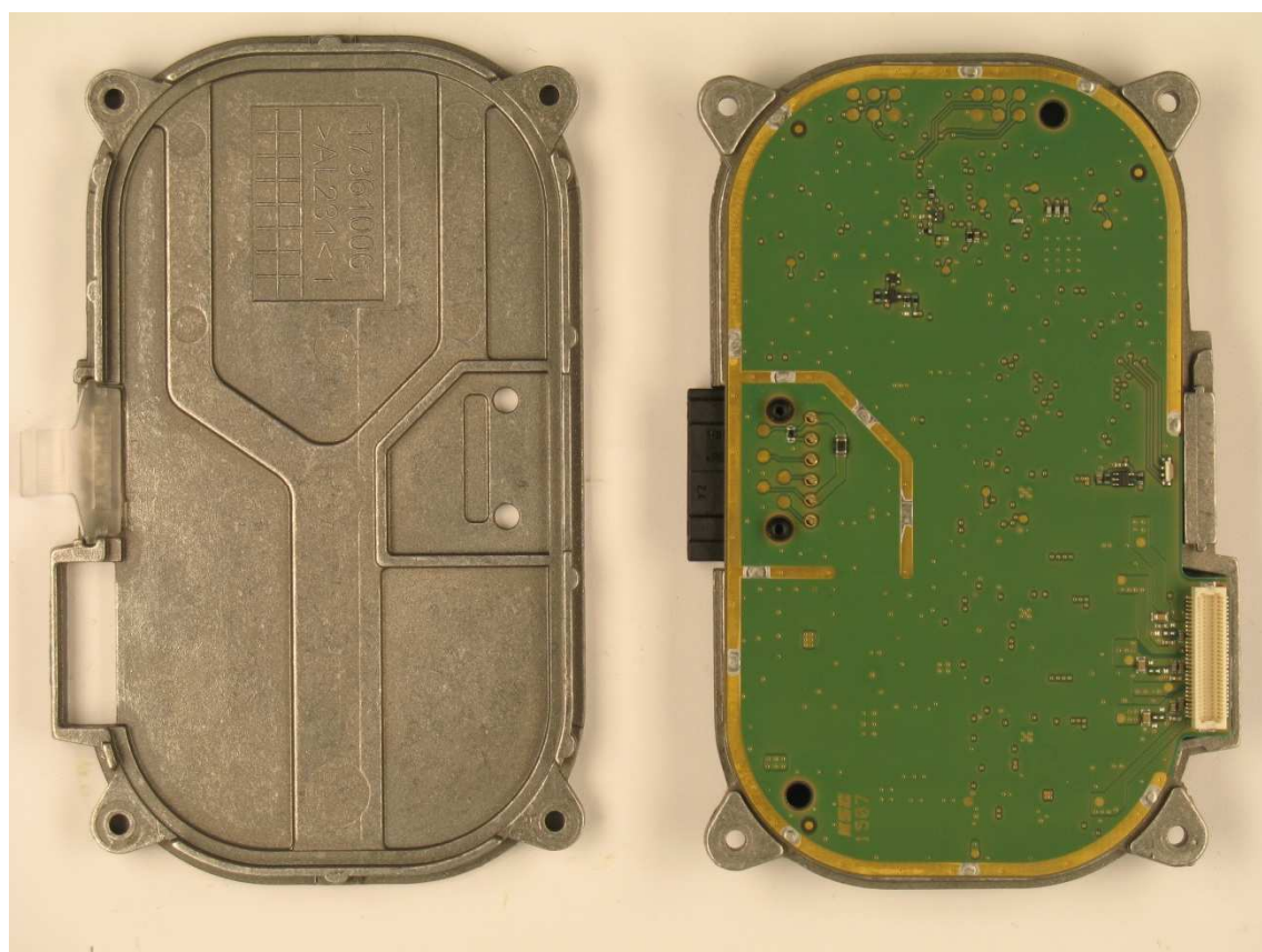
Bottom view of PCB main
