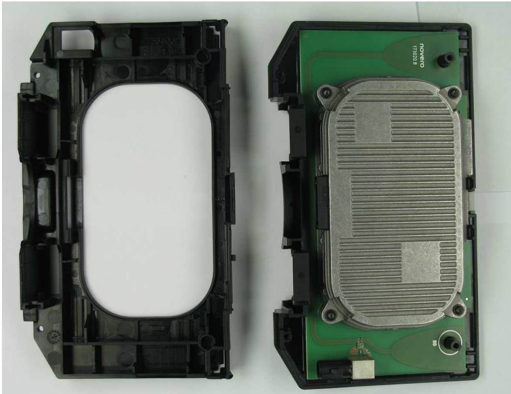
Inside view with cooling element
