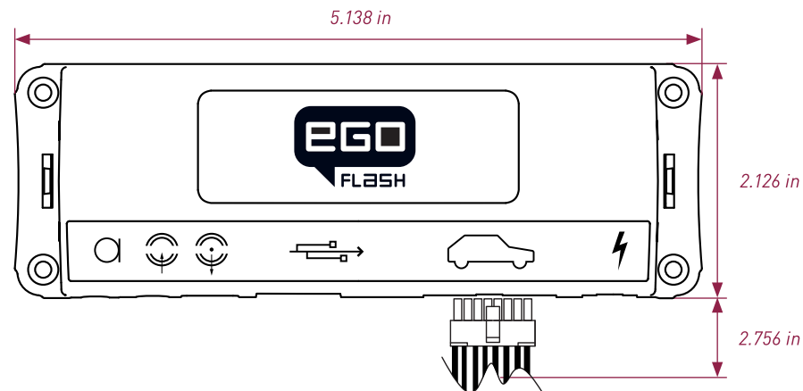
Fig. 05: Electronics box dimensions
