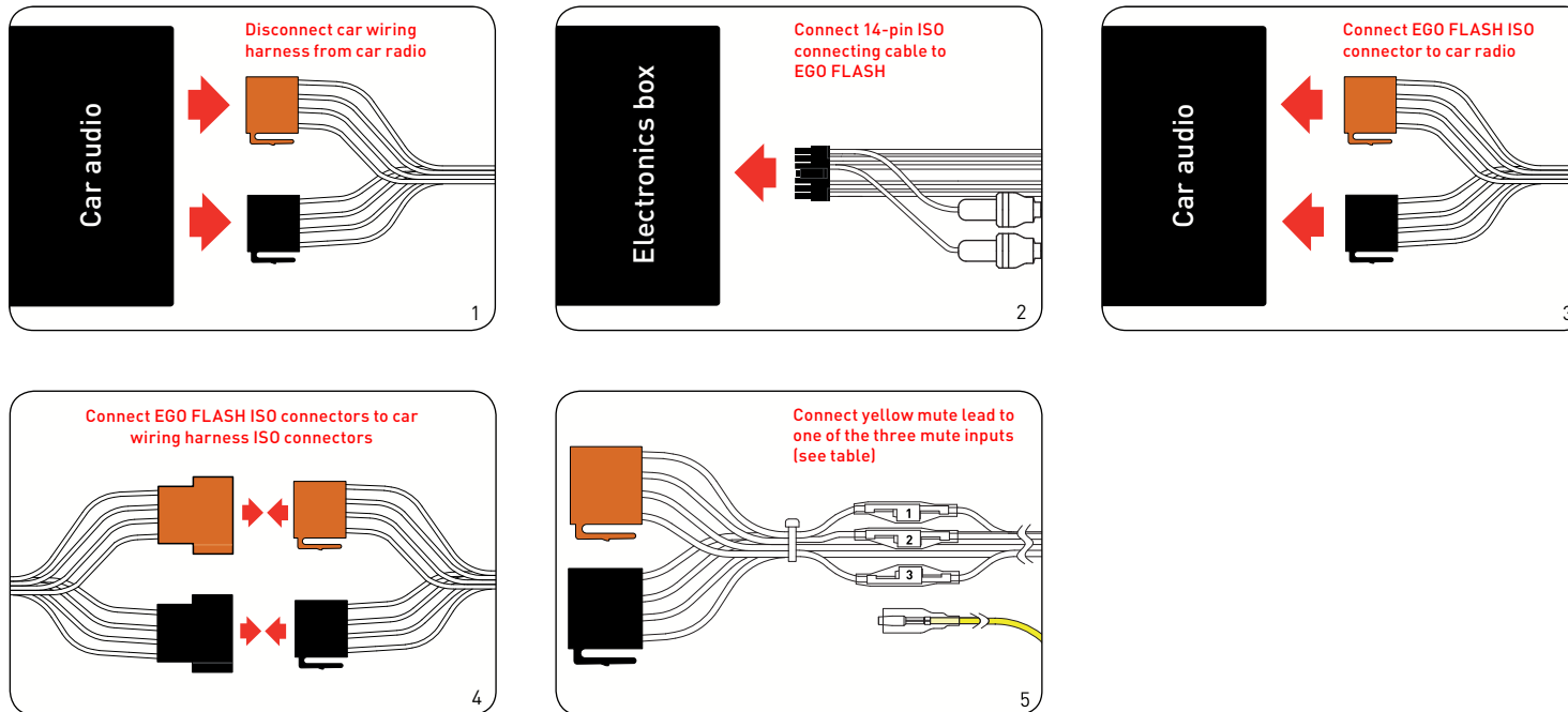
Fig. 07: Installation procedure
