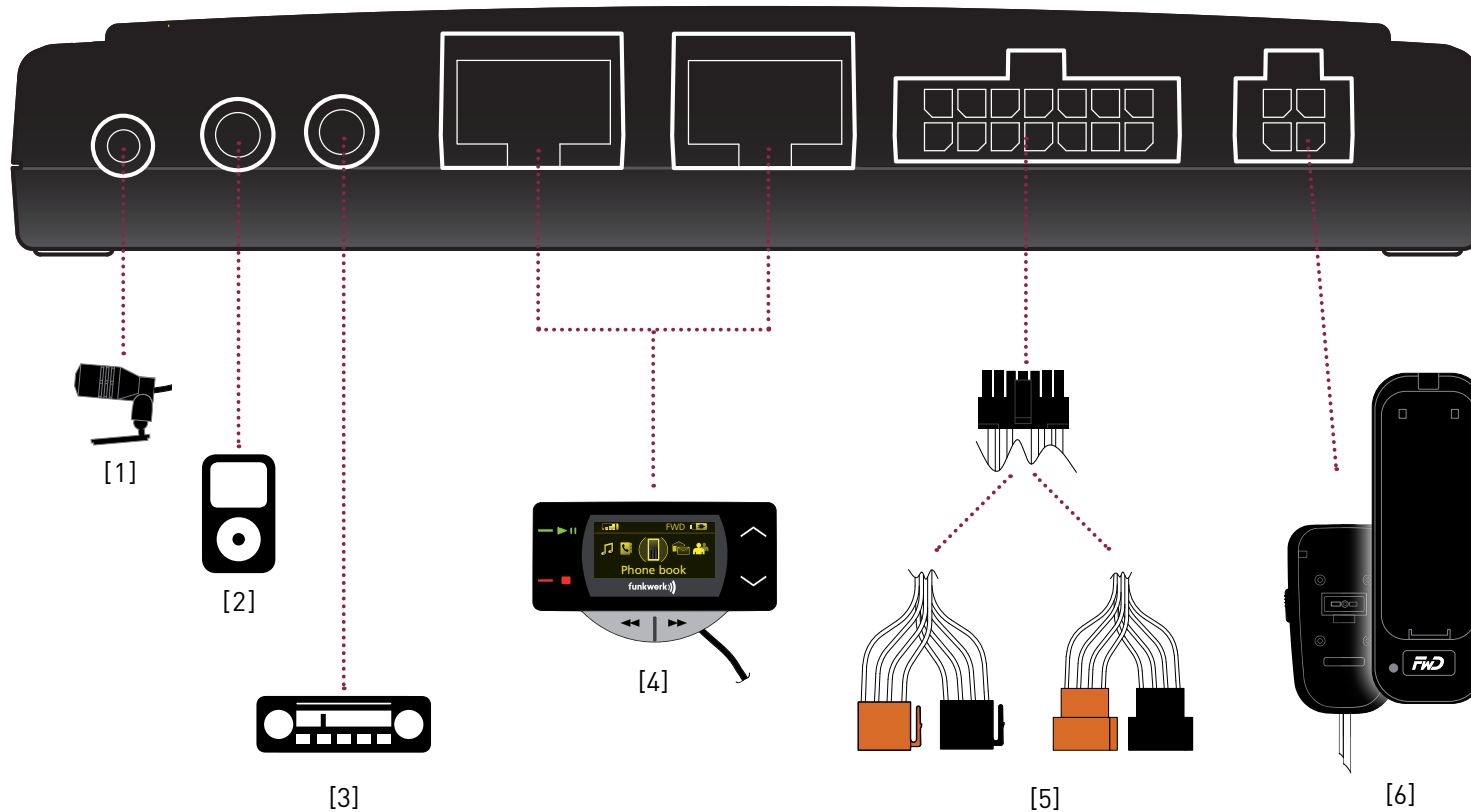
Fig. 13: Electronics box connection
