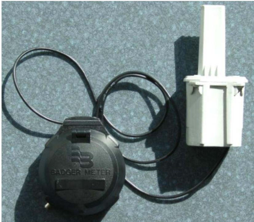
Figure 1 : Water Trak
