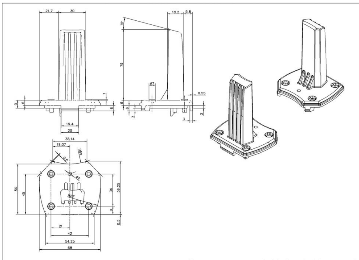
Figure 4 : Soleplate
