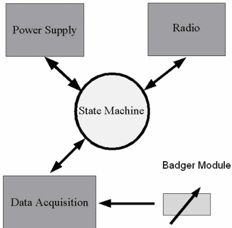
Figure 5 : Software bloc
