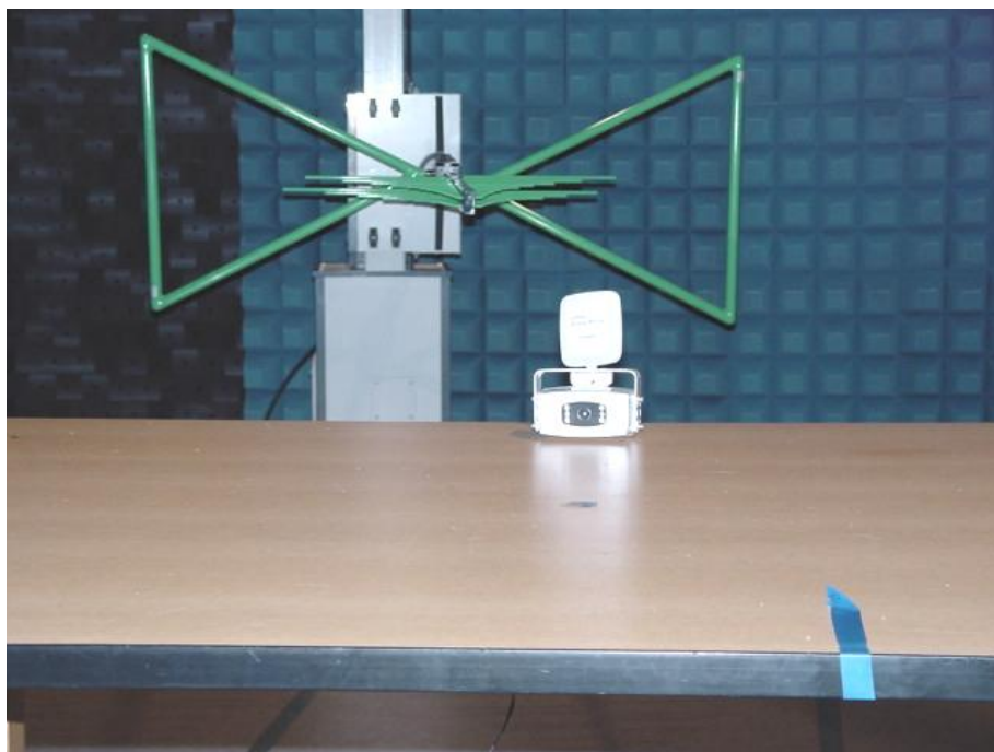
Photo 2 Test Setup for Radiated Disturbance Test
