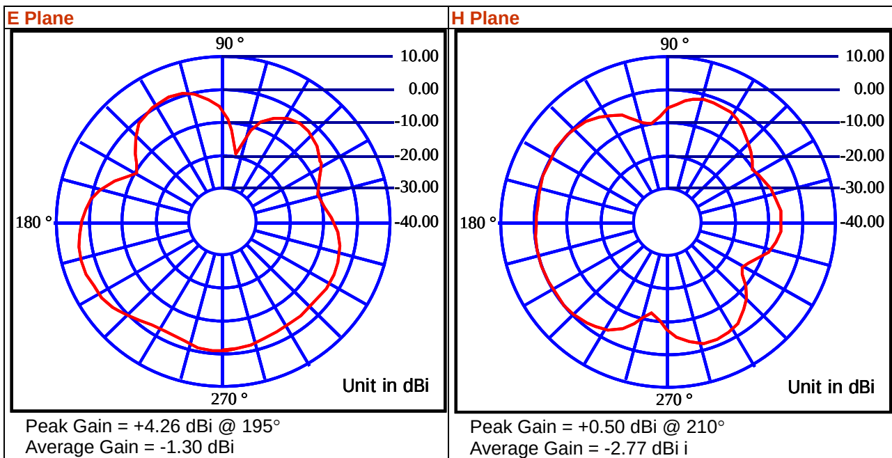
Antenna – 2:
