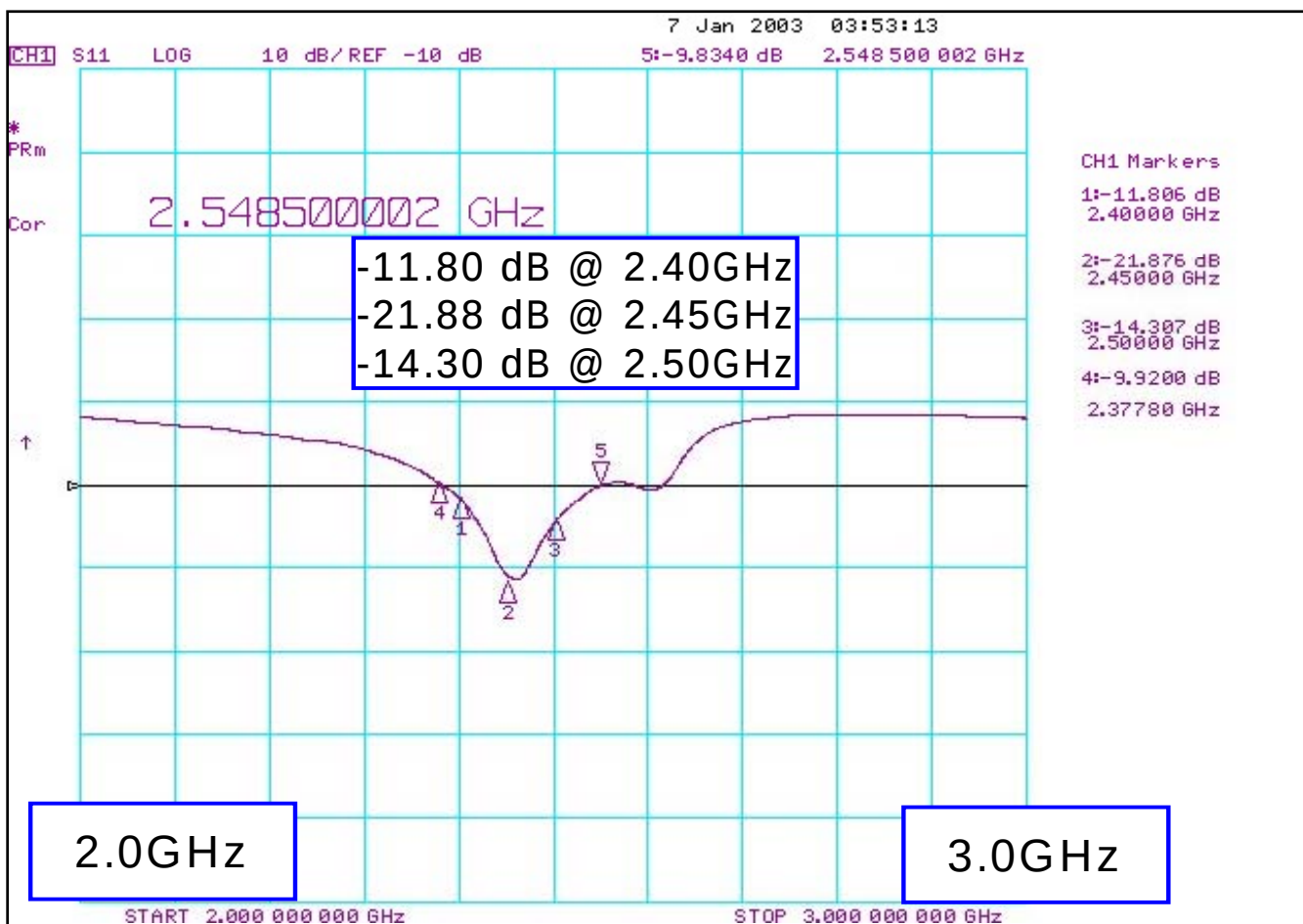
S11 for Antenna - 1:
