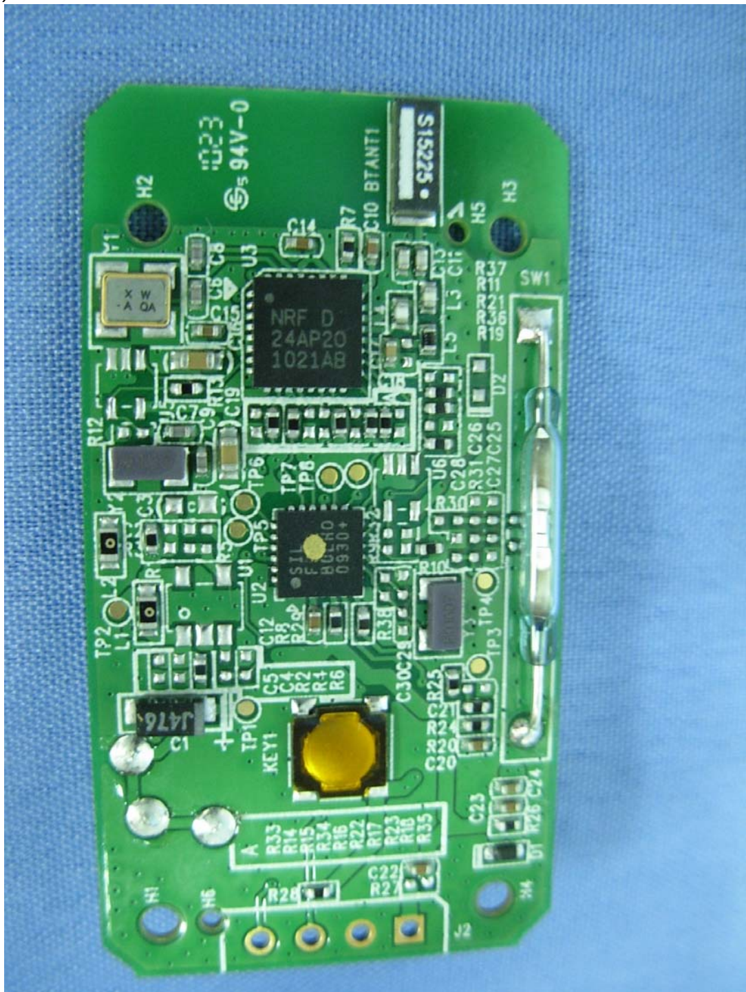
(7) EUT Photo
