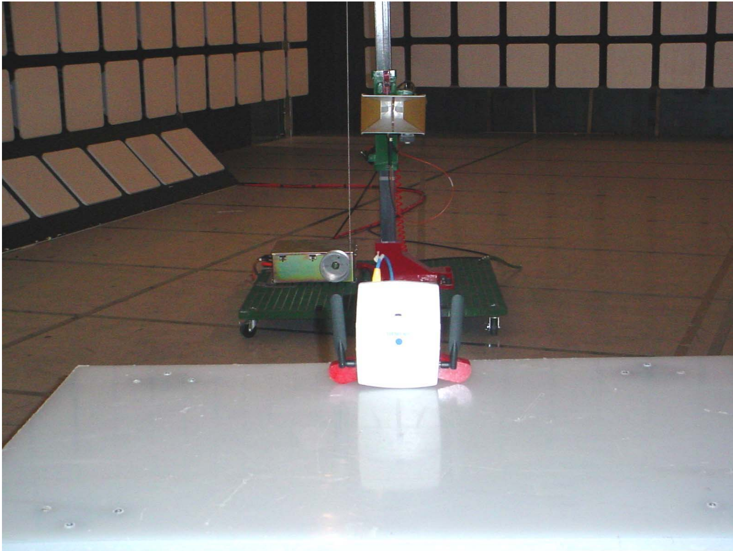
Photo #8: Altitude 350-2 Access Point with external antennas – Test Orthogonal Position #3
