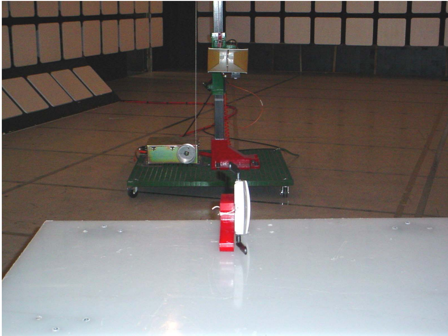
Photo #7: Altitude 350-2 Access Point with external antennas – Test Orthogonal Position #2
