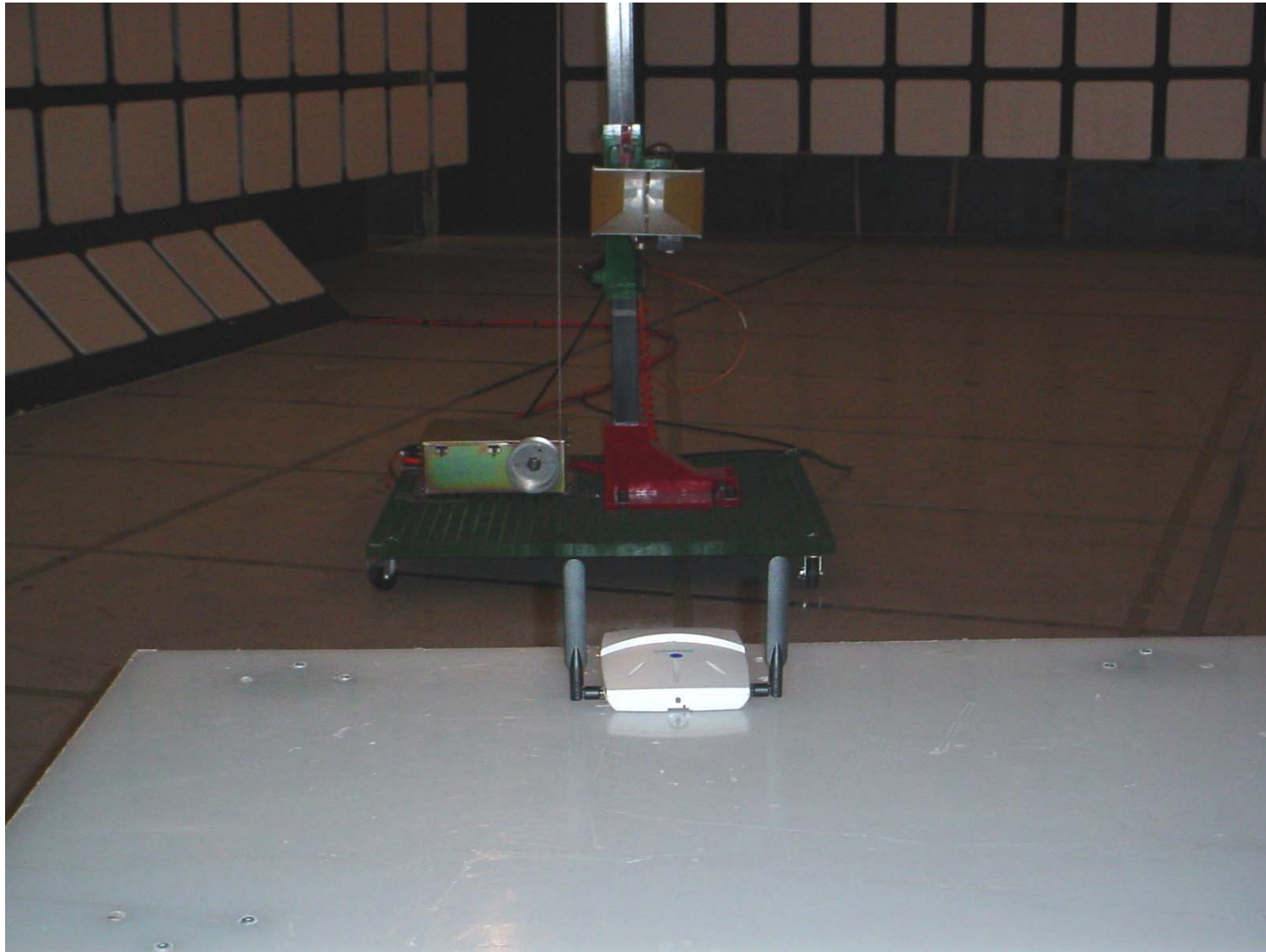
Photo #6: Altitude 350-2 Access Point with external antennas – Test Orthogonal Position #1
