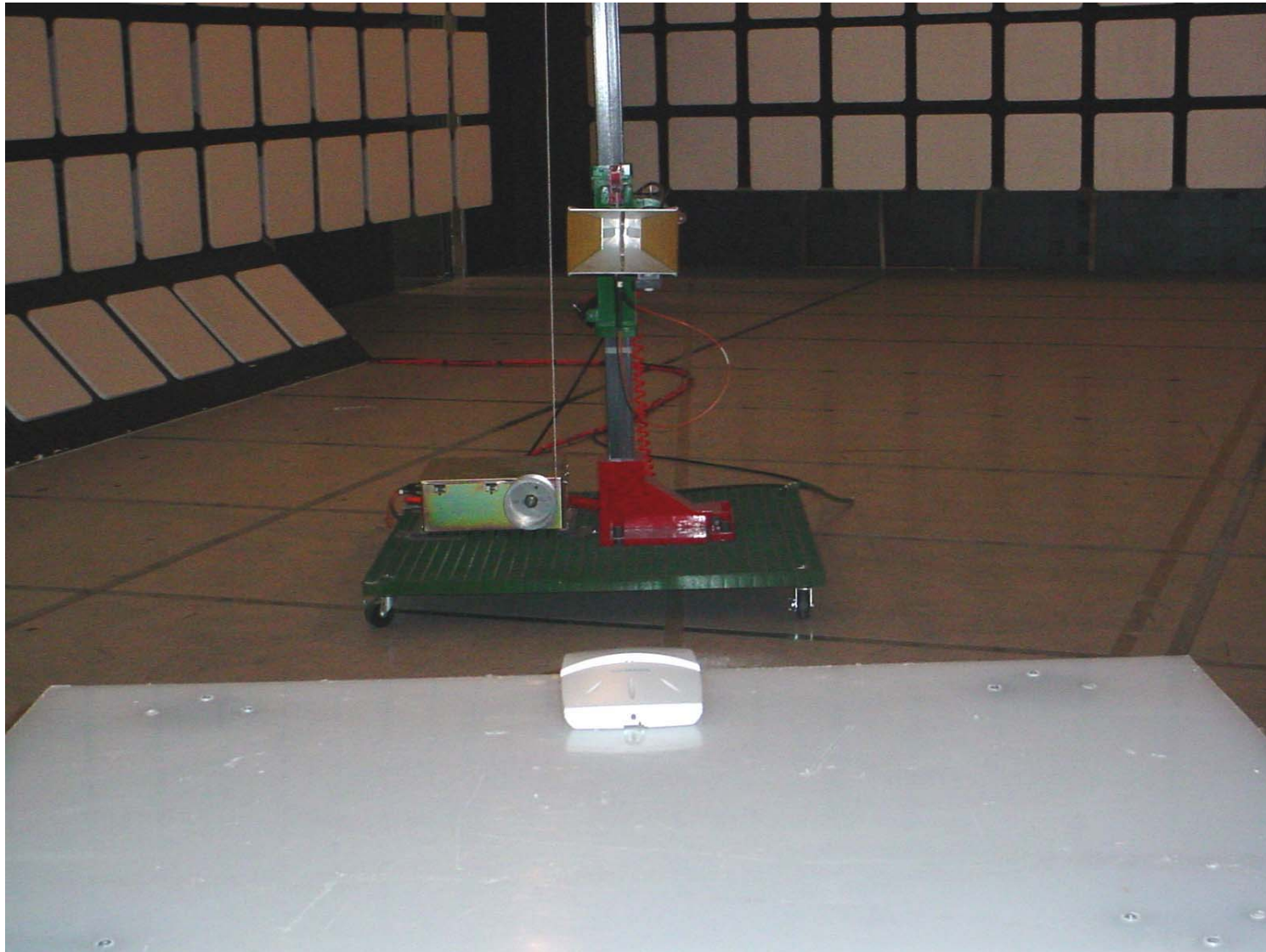
Photo #3: Altitude 350-2 Access Point with internal antennas – Test Orthogonal Position #1
