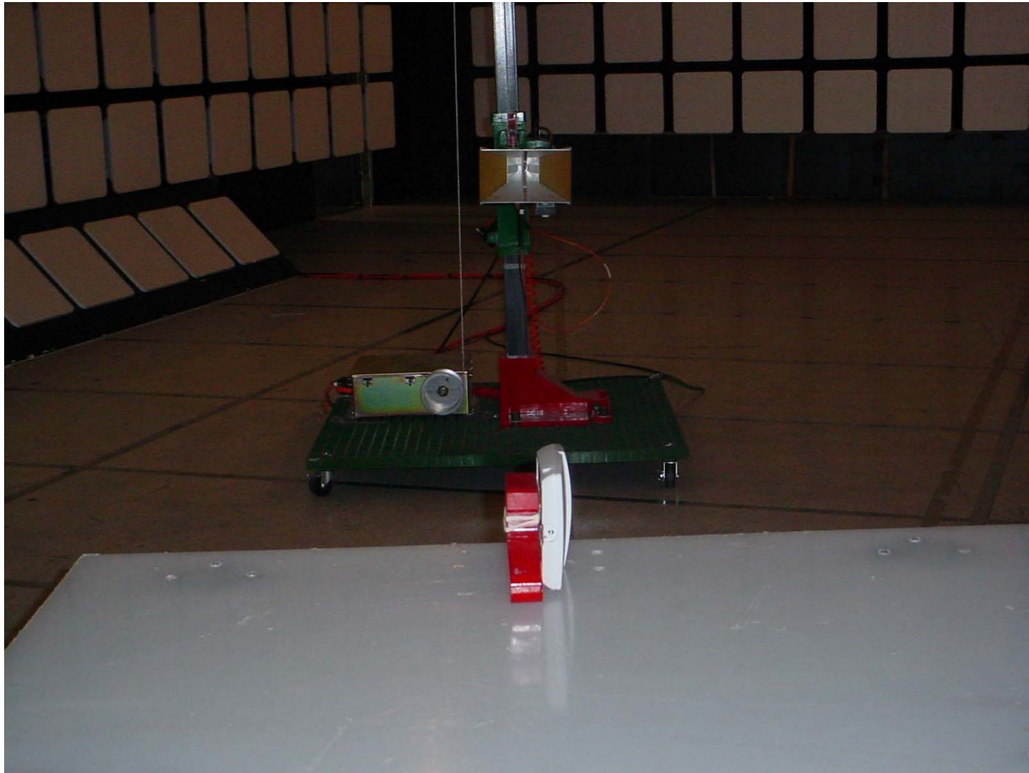
Photo #5: Altitude 350-2 Access Point with internal antennas – Test Orthogonal Position #3
