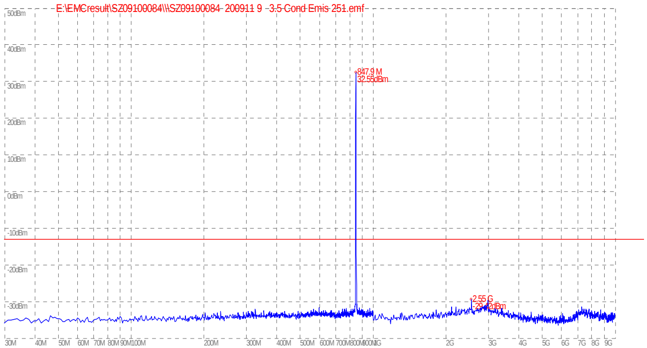
(Plot C: GSM 850MHz Channel = 251, 30MHz to 10GHz)
