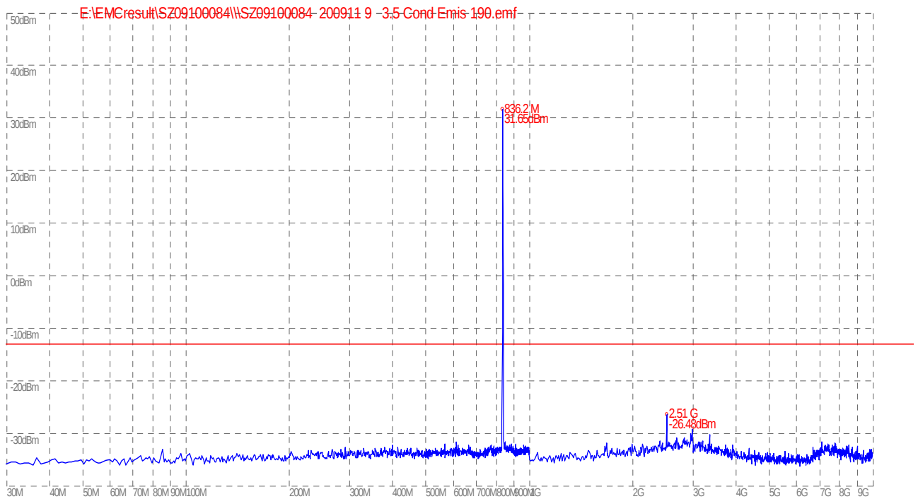
(Plot B: GSM 850MHz Channel = 190, 30MHz to 10GHz)
