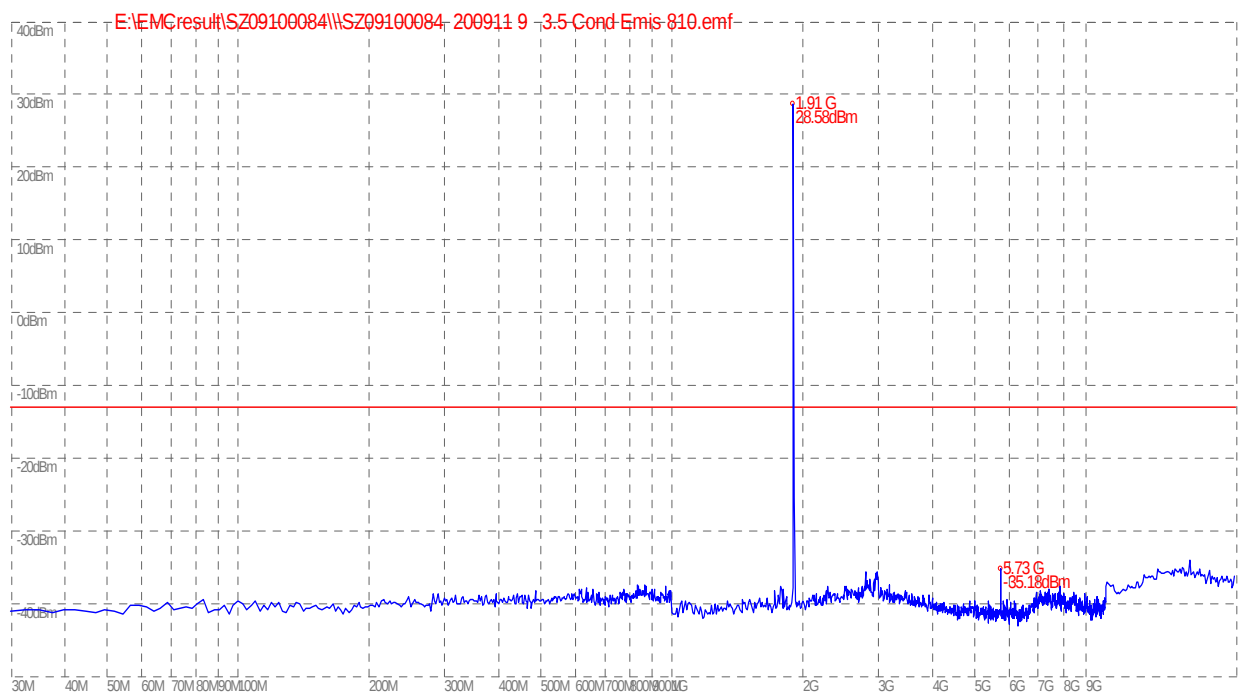
(Plot F: GSM 1900MHz Channel = 810, 30MHz to 20GHz)
