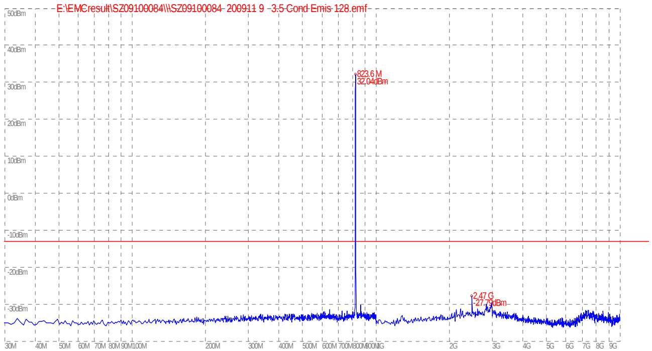
(Plot A: GSM 850MHz Channel = 128, 30MHz to 10GHz)
