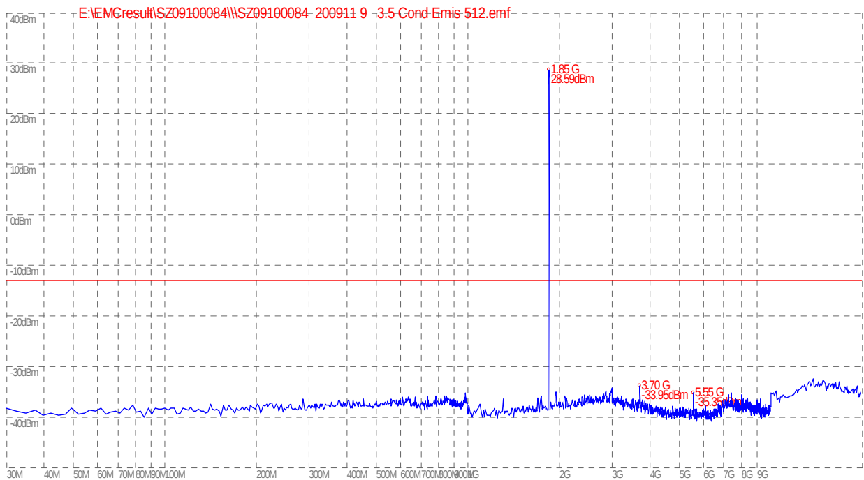
(Plot D: GSM 1900MHz Channel = 512, 30MHz to 20GHz)
