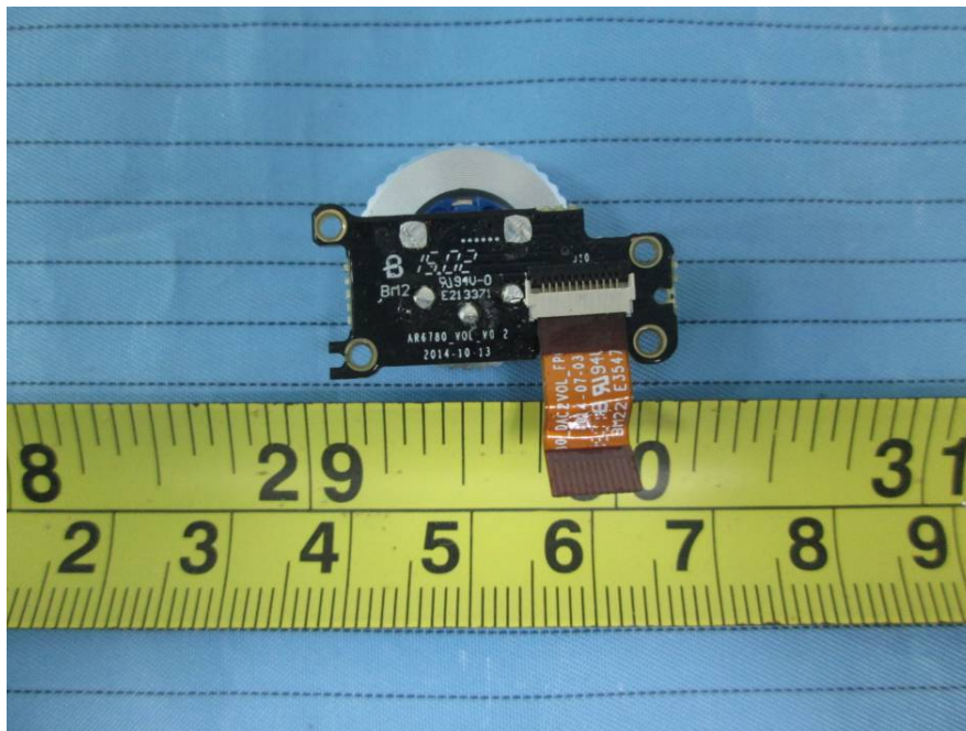
EUT – Connected Board Bottom View
