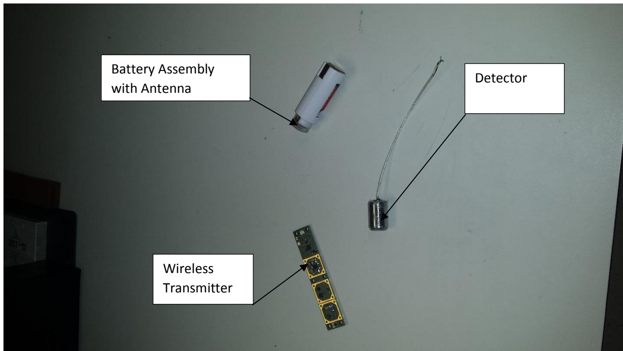
Photograph 1. Wireless Pilot Probe (Transmitter) De-assembled – Internal Components
