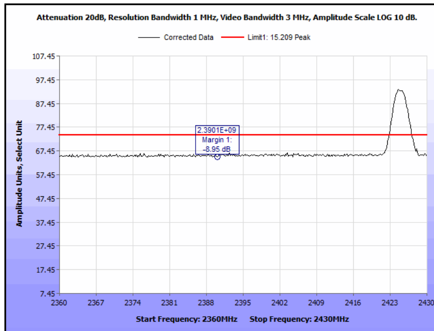
Plot 12. Radiated Restricted Band Edge, Peak, Channel 1
