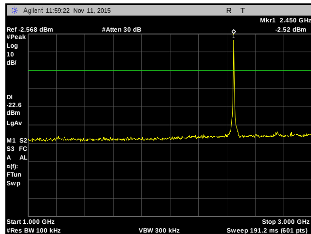
Plot 19. Conducted Spurious Emissions, 1 GHz – 3 GHz, Channel 2
