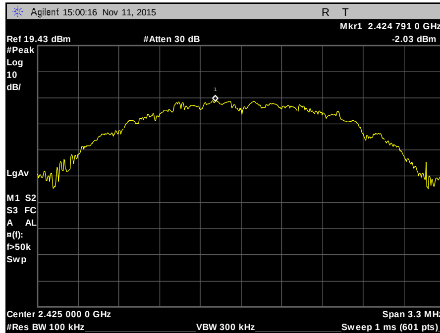
Plot 23. Peak Power Spectral Density, Channel 1
