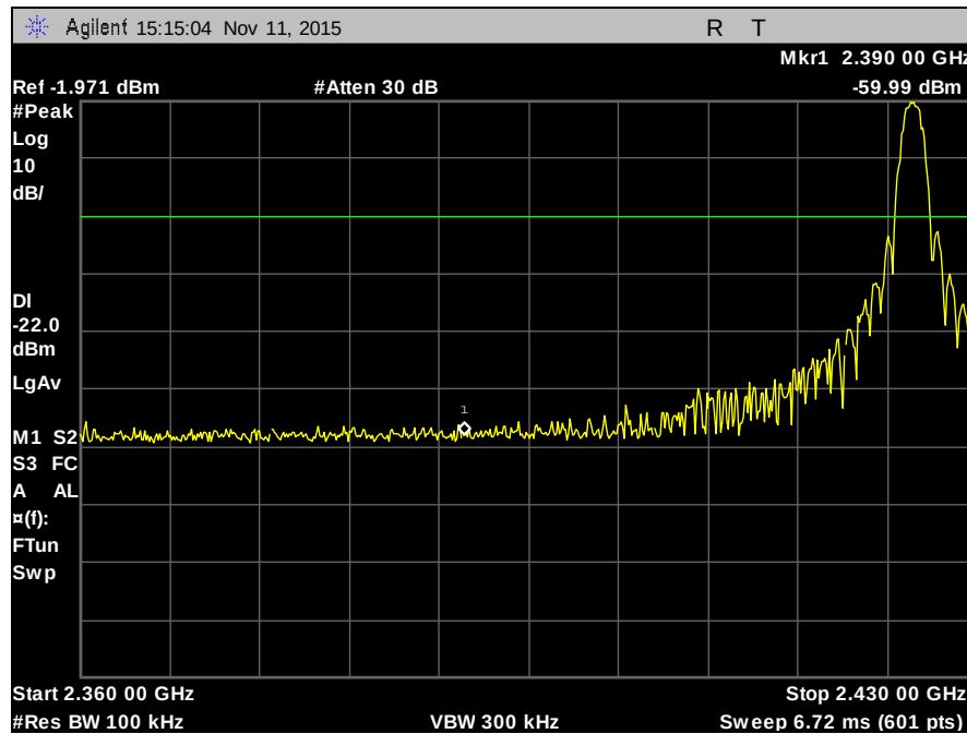
Plot 21. Conducted Band Edge, Channel 1
