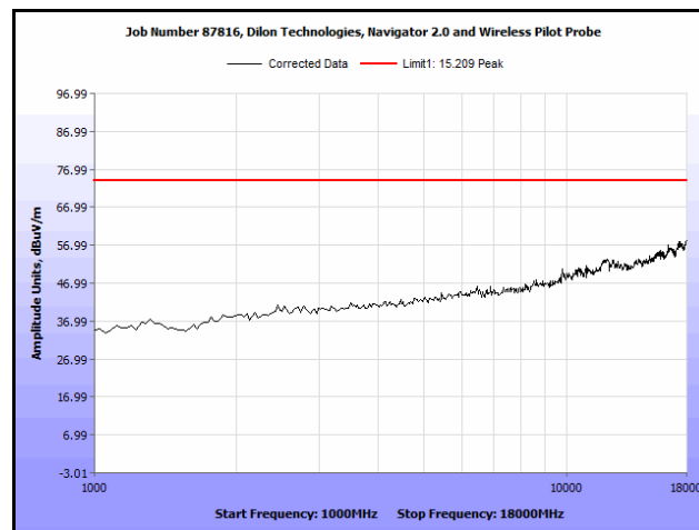
Plot 10. Radiated Spurious Emissions, 1 GHz – 18 GHz, Peak, Channel 2
