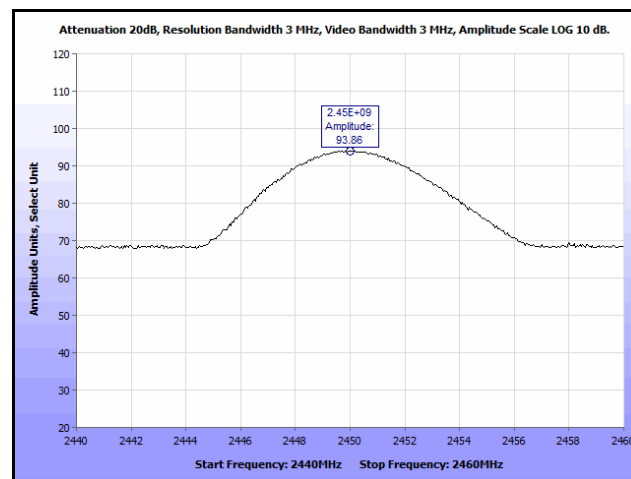
Plot 4. Peak Power Output, Channel 2
