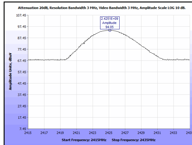
Plot 3. Peak Power Output, Channel 1
