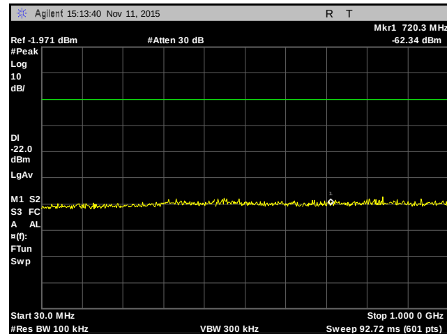
Plot 15. Conducted Spurious Emissions, 30 MHz – 1 GHz, Channel 1
