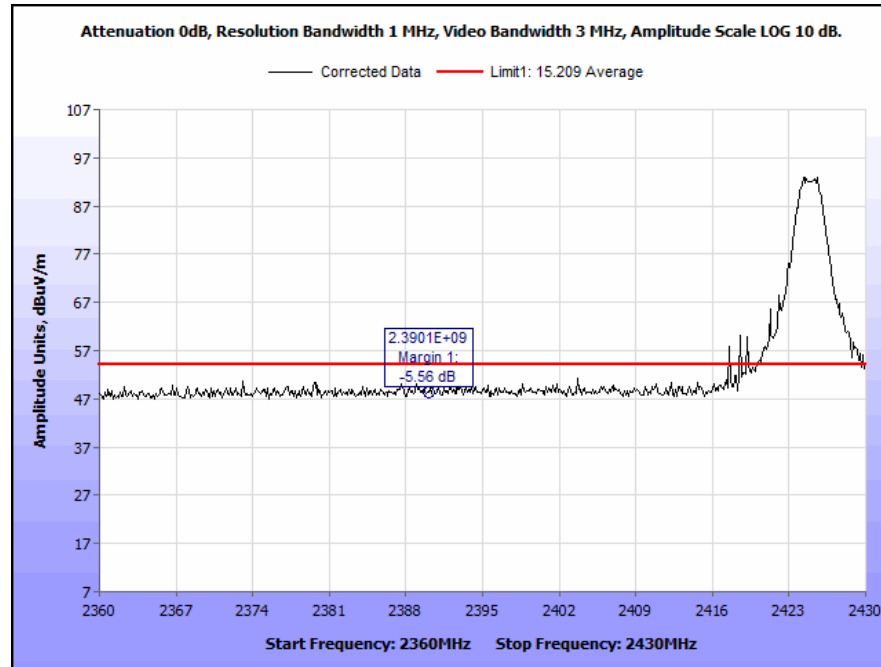
Plot 11. Radiated Restricted Band Edge, Average, Channel 1
