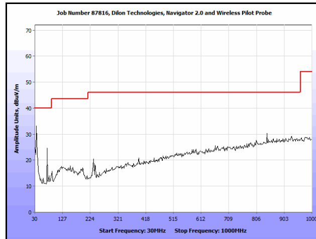
Plot 5. Radiated Spurious Emissions, 30 MHz – 1 GHz, Channel 1
