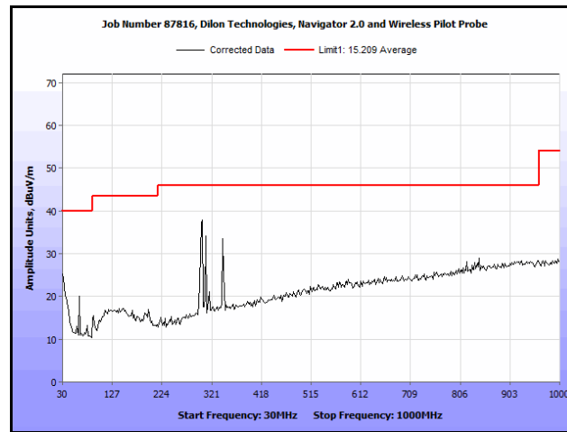
Plot 8. Radiated Spurious Emissions, 30 MHz – 1 GHz, Channel 2
