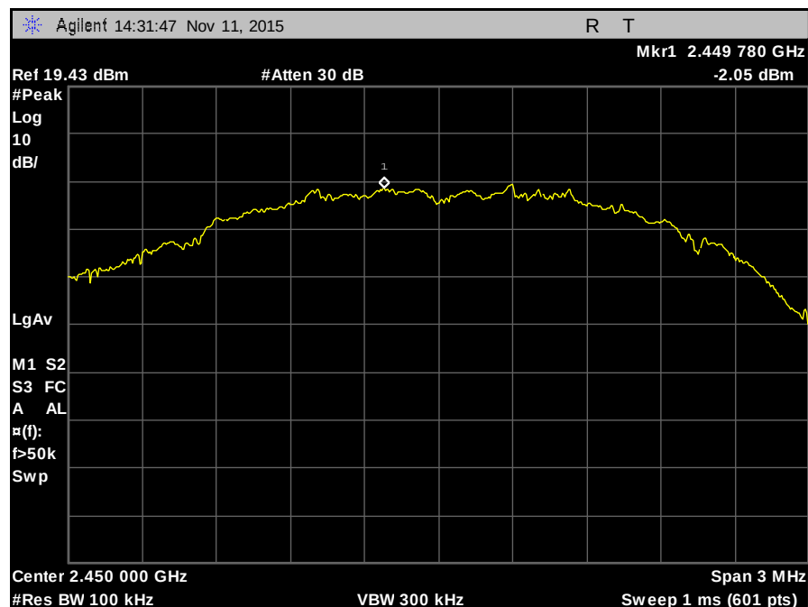
Plot 24. Peak Power Spectral Density, Channel 2
