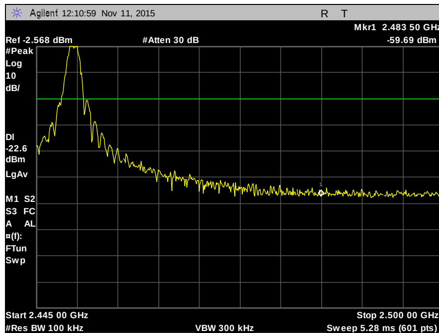
Plot 22. Conducted Band Edge, Channel 2
