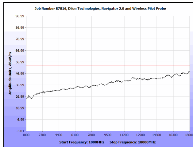
Plot 6. Radiated Spurious Emissions, 1 GHz – 18 GHz, Average, Channel 1
