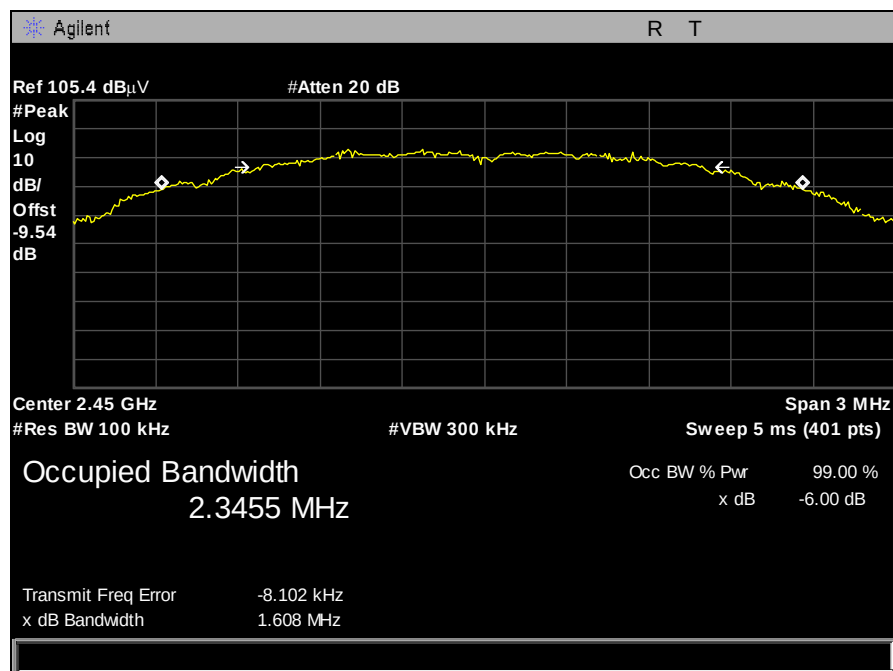
Plot 2. 6 dB Occupied Bandwidth, Channel 2
