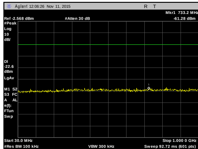
Plot 18. Conducted Spurious Emissions, 30 MHz – 1 GHz, Channel 2
