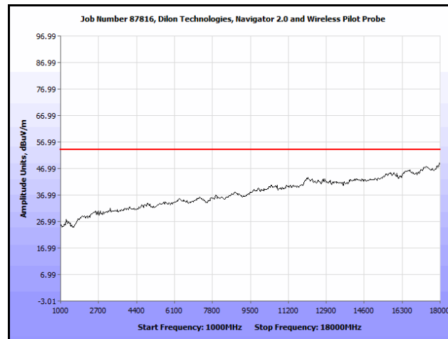
Plot 9. Radiated Spurious Emissions, 1 GHz – 18 GHz, Average, Channel 2
