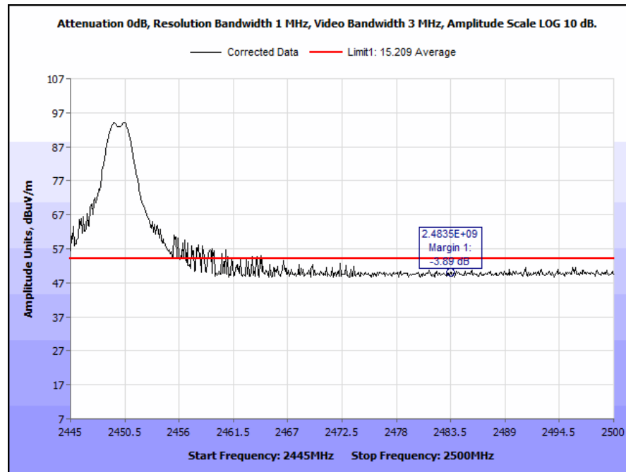
Plot 13. Radiated Restricted Band Edge, Average, Channel 2
