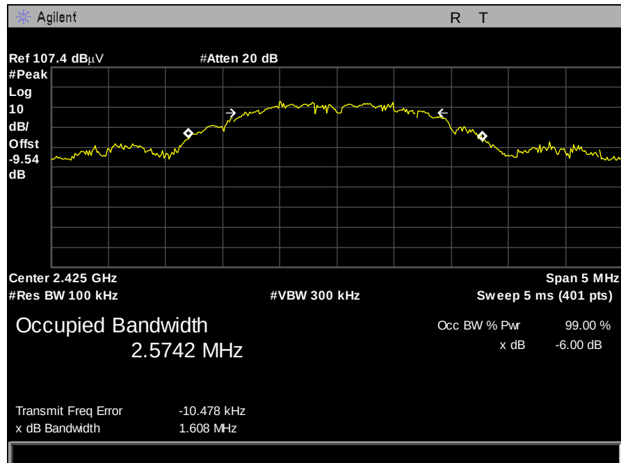
Plot 1. 6 dB Occupied Bandwidth, Channel 1
