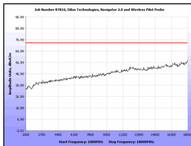
Plot 7. Radiated Spurious Emissions, 1 GHz – 18 GHz, Peak, Channel 1
