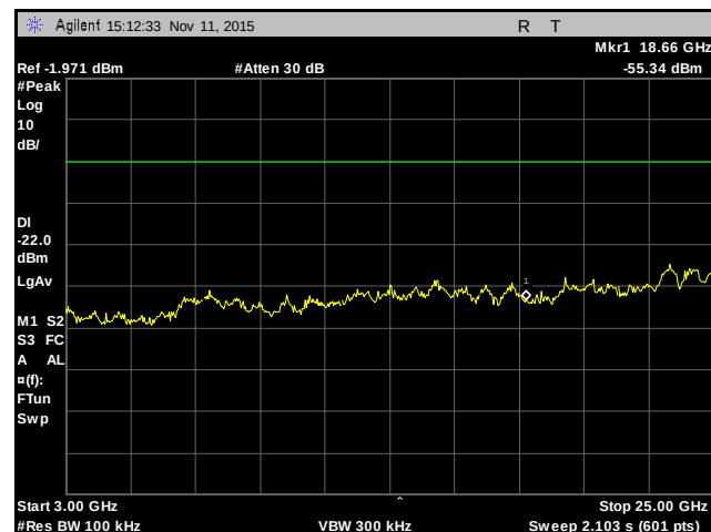
Plot 17. Conducted Spurious Emissions, 3 GHz – 25 GHz, Channel 1
