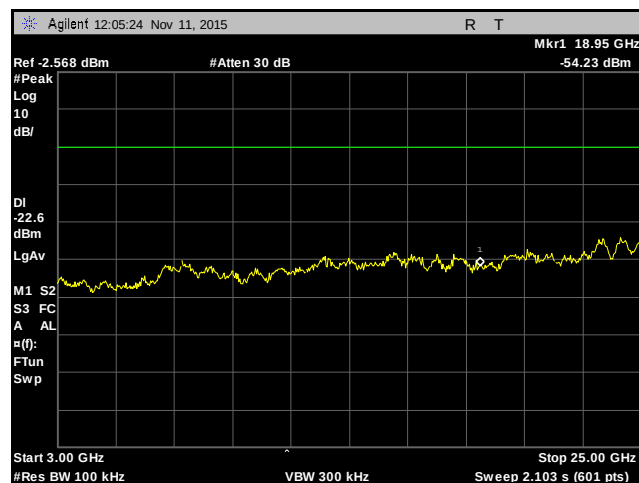
Plot 20. Conducted Spurious Emissions, 3 GHz – 25 GHz, Channel 2
