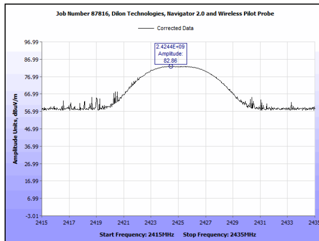
Plot 3. Peak Power Output, Channel 1
