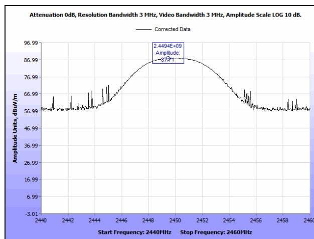
Plot 4. Peak Power Output, Channel 2
