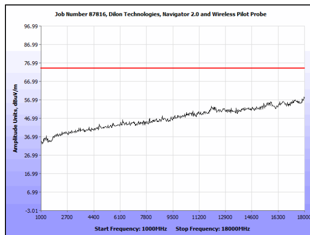
Plot 7. Radiated Spurious Emissions, 1 GHz – 18 GHz, Peak, Channel 1
