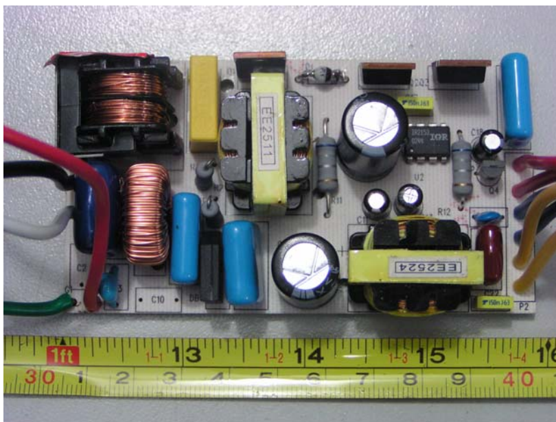
EUT of FEB-2-26-UNV-H-S-A - PCB View (1)
