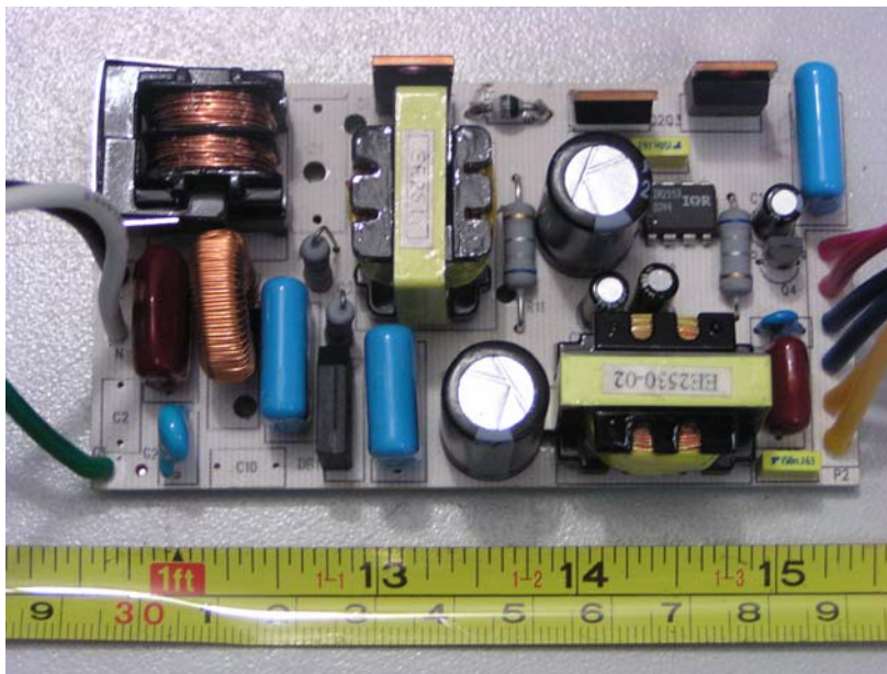
EUT of FEB-2-13-UNV-H-S-A - PCB View (1)
