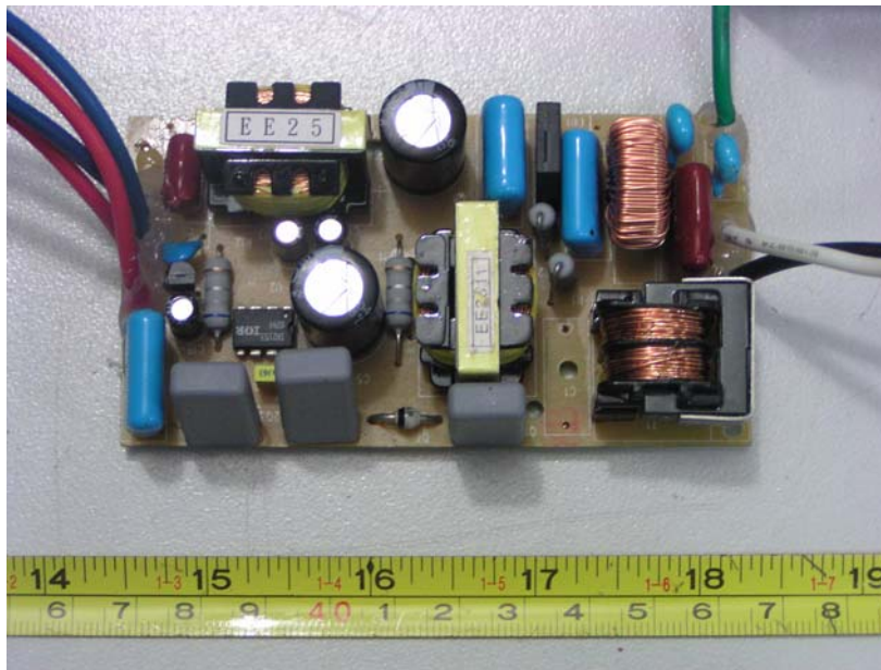
EUT of FEB-1-13-UNV-H-S-A - PCB View (1)
