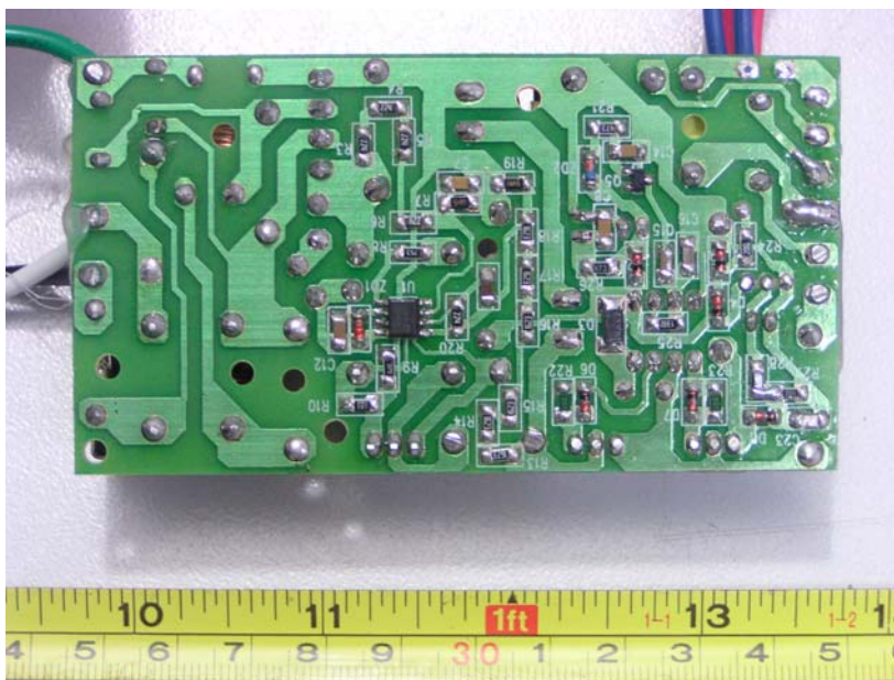
EUT of FEB-1-26-UNV-H-S-A - PCB View (2)
