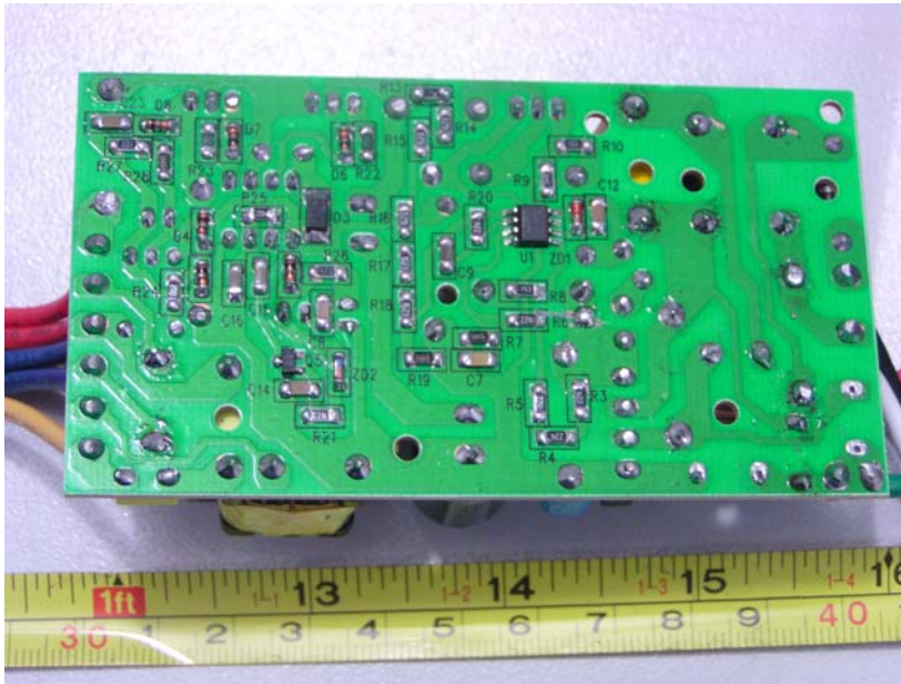
EUT of FEB-2-26-UNV-H-S-A - PCB View (2)
