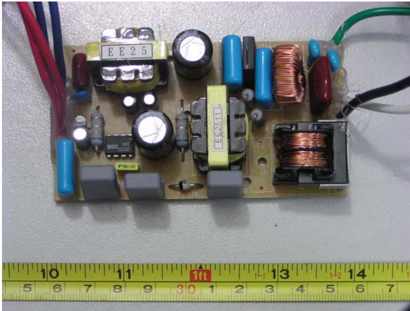
EUT of FEB-1-26-UNV-H-S-A - PCB View (1)
