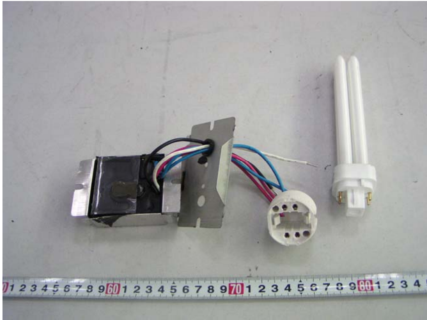
FEB-1-13-120-N-S-A: EUT - Inside View (1)
