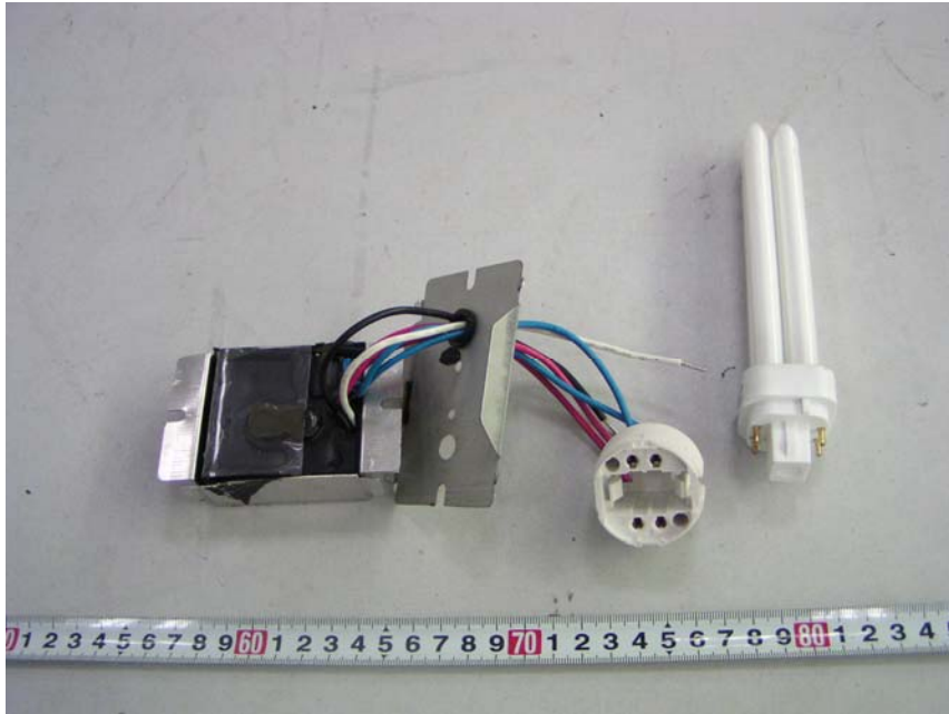
FEB-1-26-120-N-S-A: EUT - Inside View (1)
