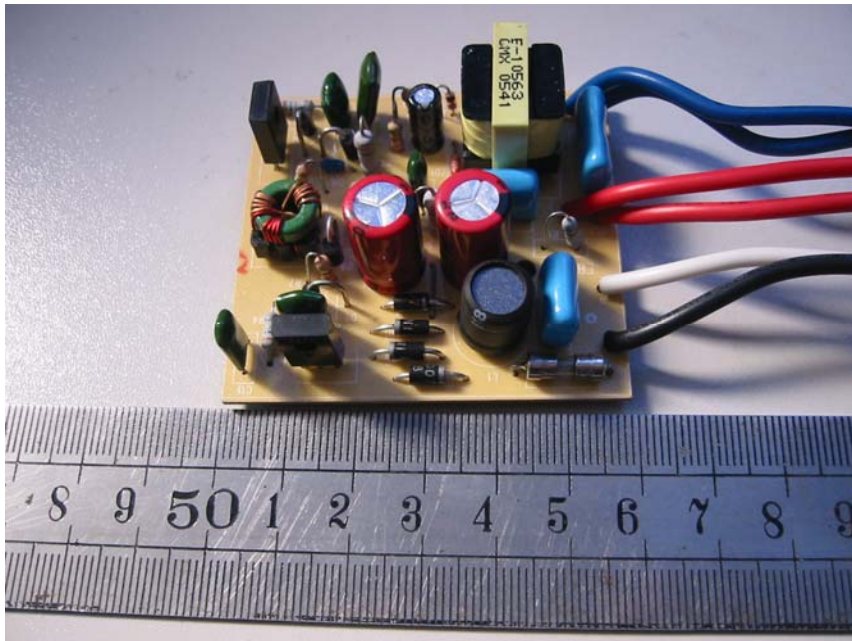
FEB-1-13-120-N-S-A: EUT – PCB Front View
