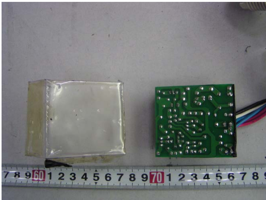
FEB-1-26-120-N-S-A: EUT – PCB Rear View
