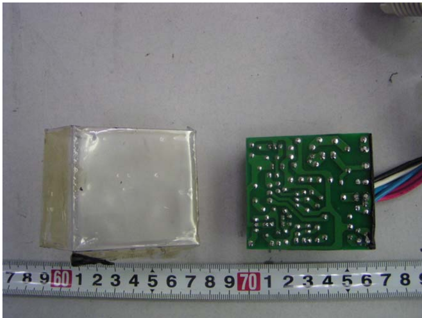
FEB-1-13-120-N-S-A: EUT – PCB Rear View
