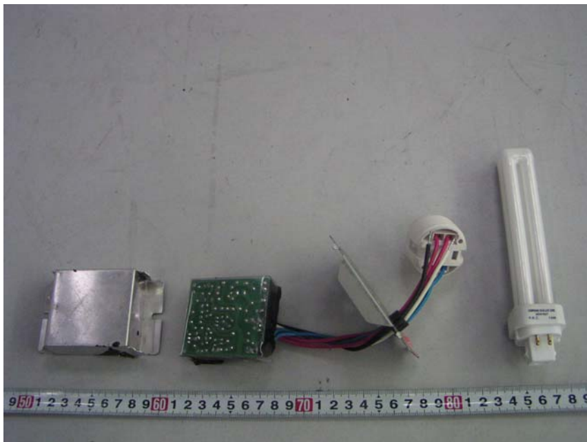
FEB-1-26-120-N-S-A: EUT - Inside View (2)
