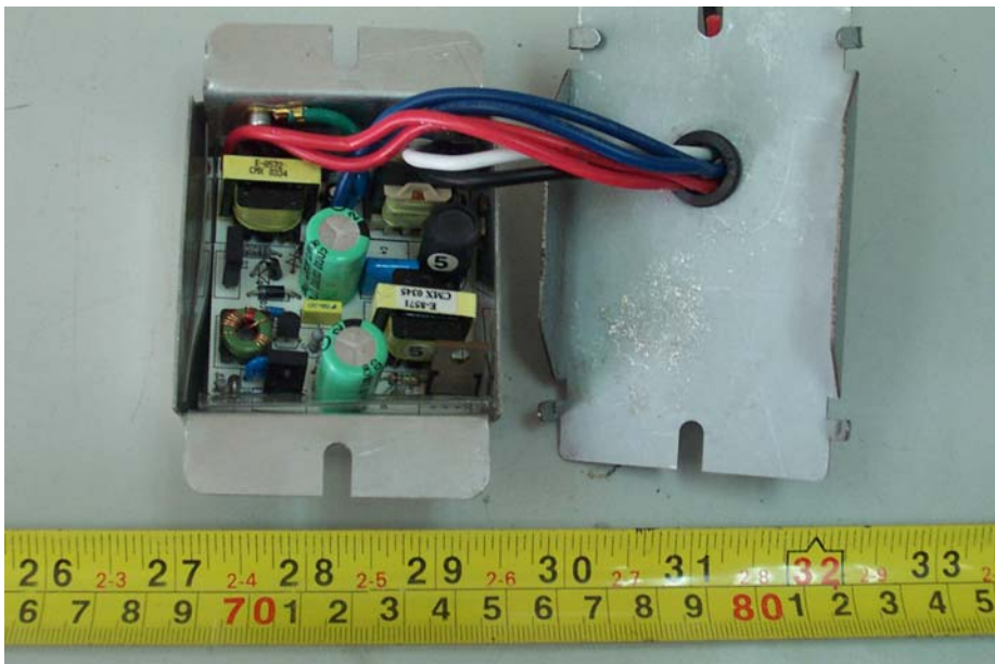
EUT of FEB-2-13-120-EH-S-A - Uncovered View
