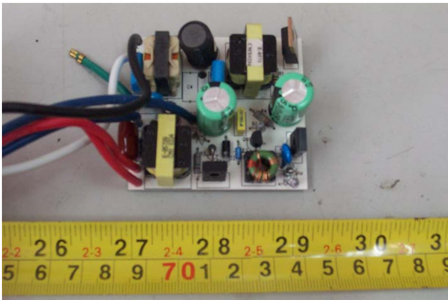
EUT of FEB-1-26-120-EH-S-A - PCB View (1)
