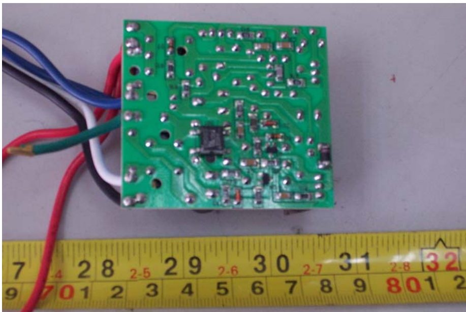
EUT of FEB-2-13-120-EH-S-A - PCB View (2)
