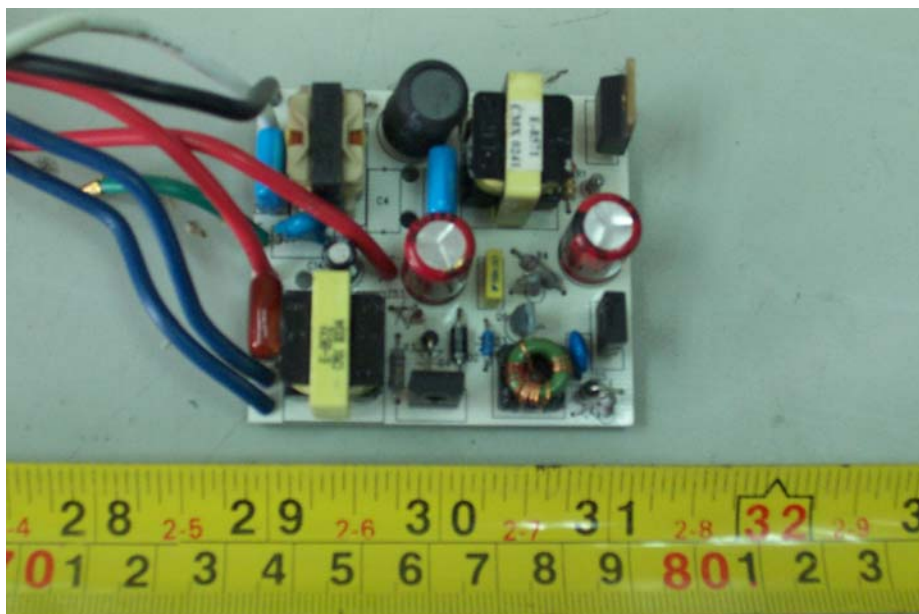
EUT of FEB-1-13-120-EH-S-A - PCB View (1)
