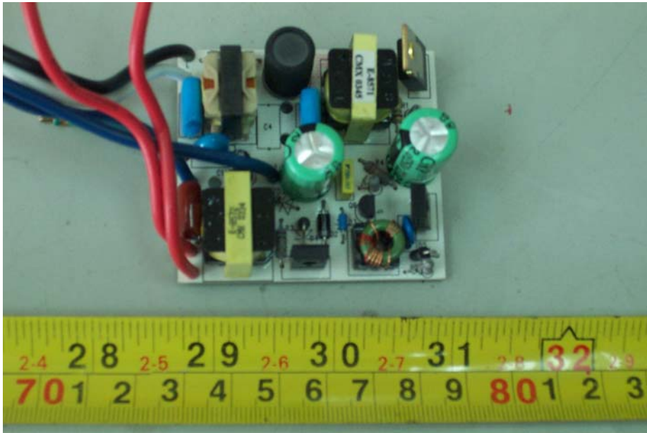
EUT of FEB-2-13-120-EH-S-A - PCB View (1)
