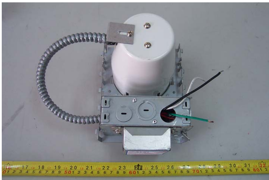
General Appearance of FEB-1-26-120-EH-S-A - 2
