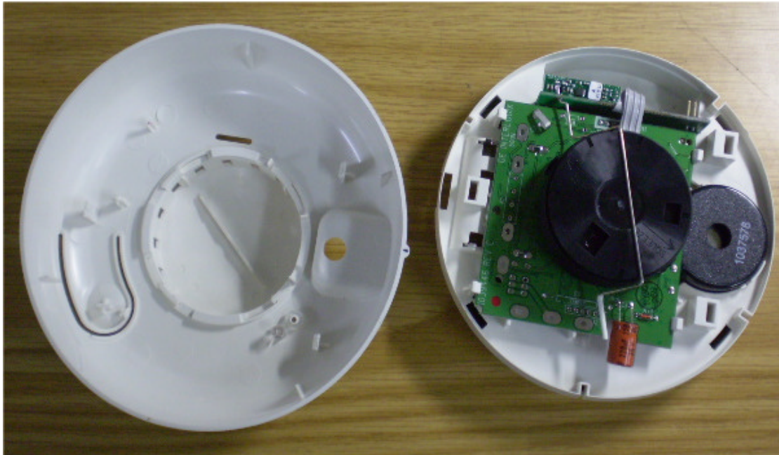
Photograph No.2 EL2603 smoke detector with cover removed
