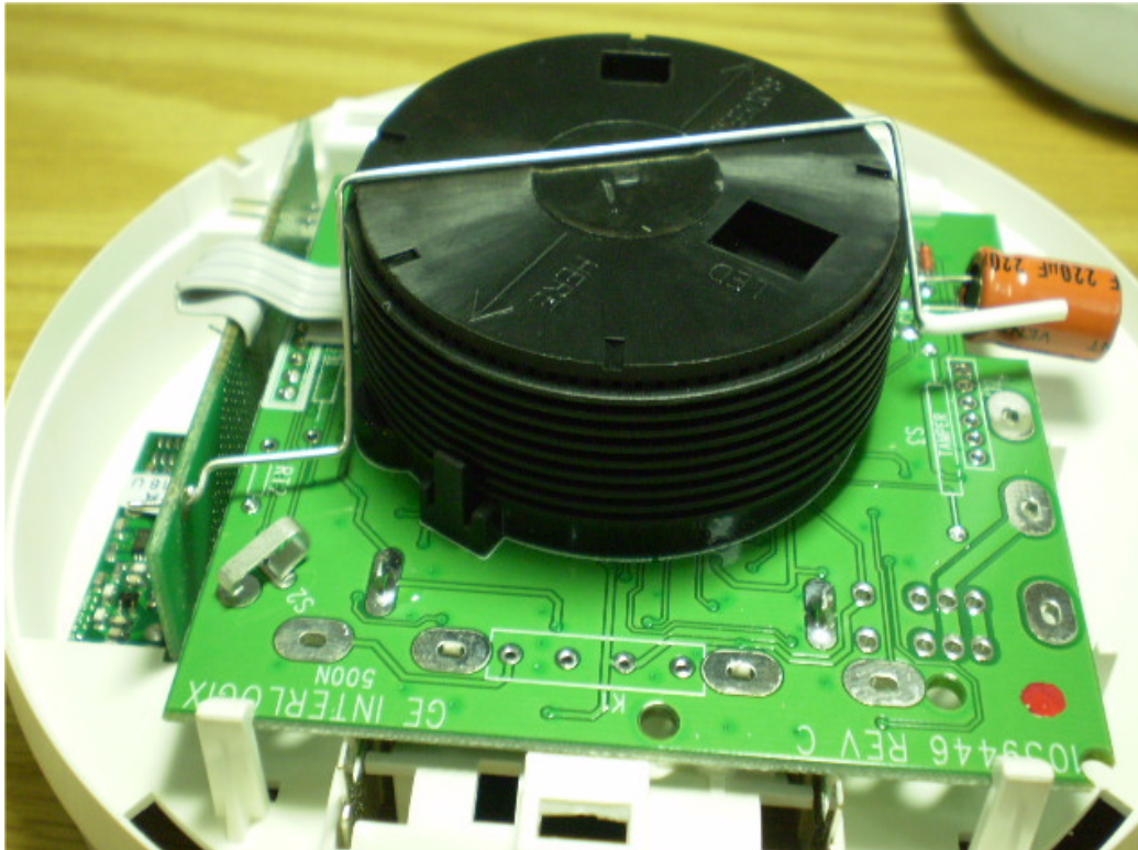
Photograph No.4 EL2603 smoke detector side view with antenna
