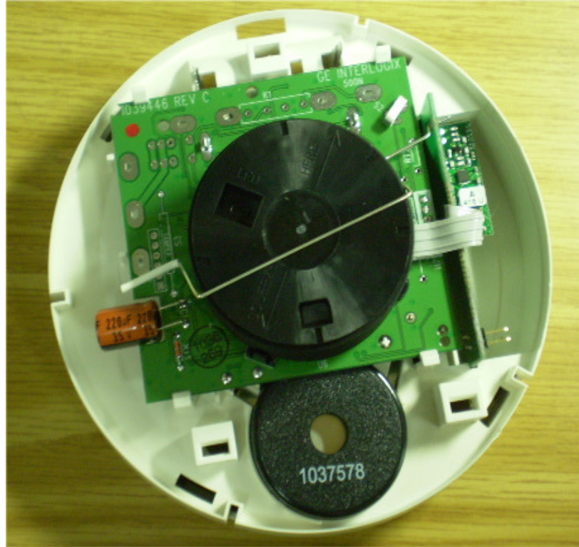
Photograph No.3 EL2603 smoke detector internal view
