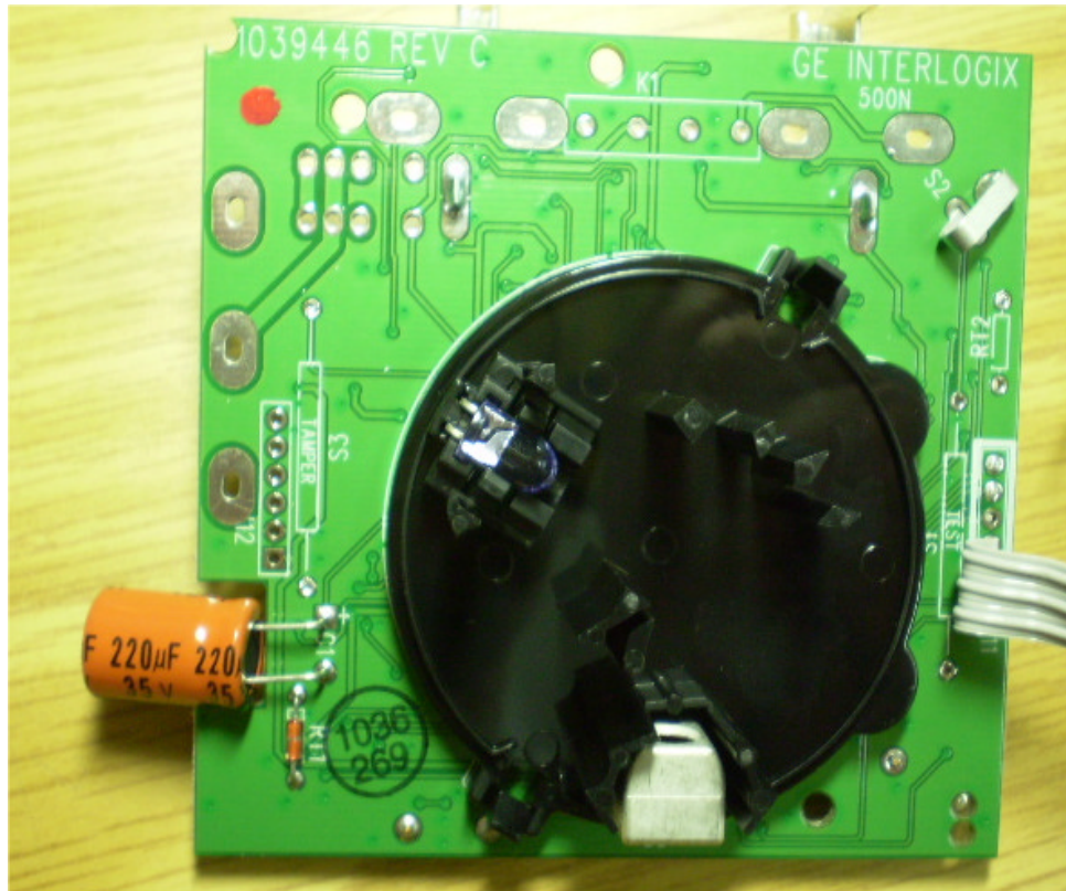
Photograph No.5 EL2603 sensor PCB
