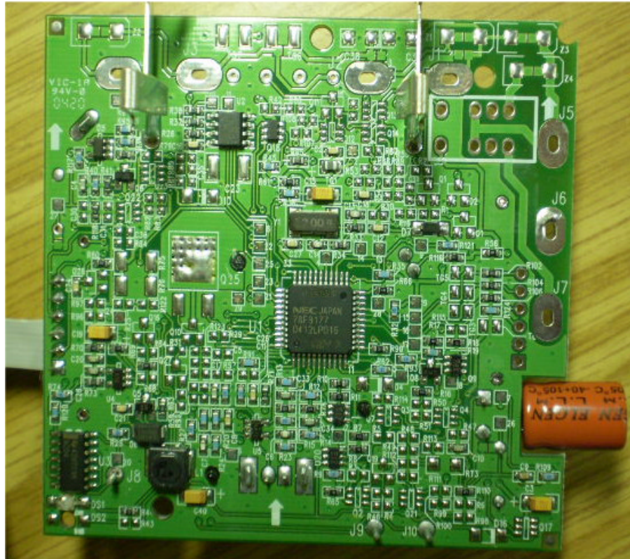
Photograph No.6 EL2603 sensor PCB second side
