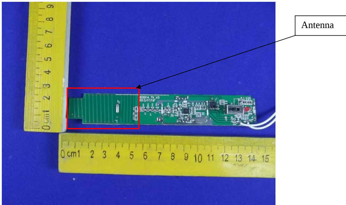
Figure 8 PCB of the EUT-Front View
