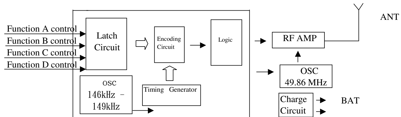
TX Block Diagram
