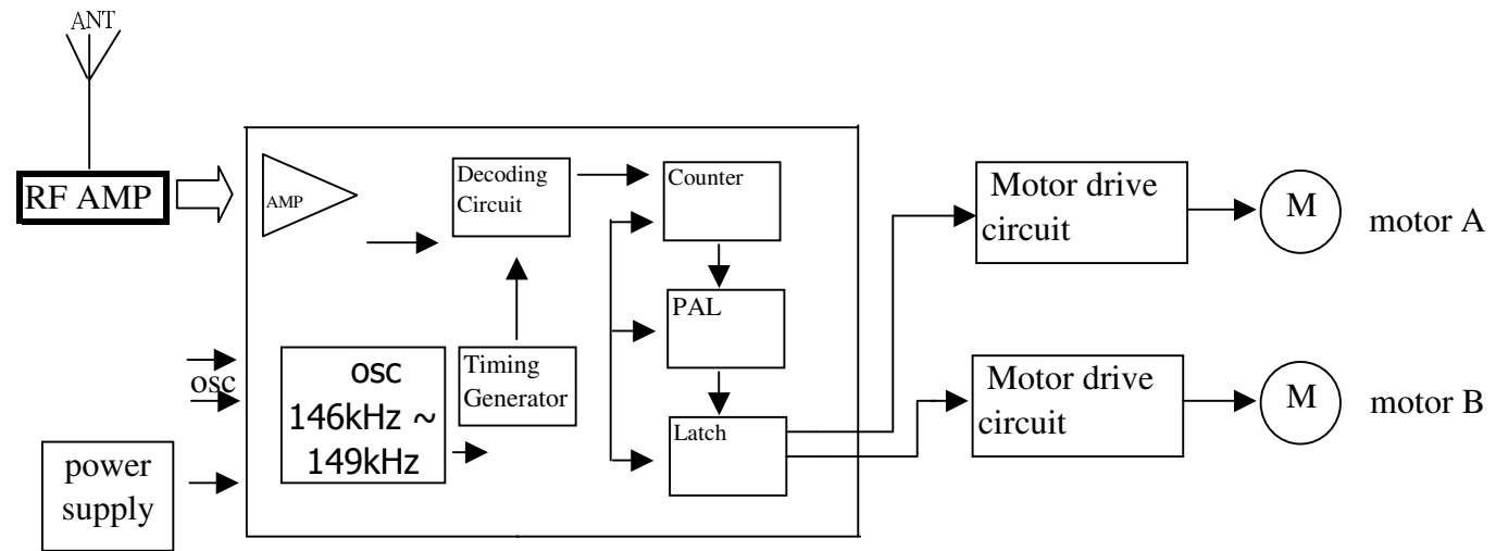
RX Block Diagram
