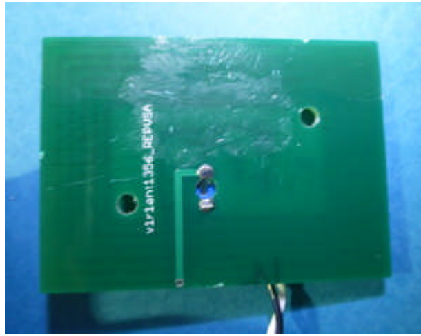
RFID Antenna PCB Bottom
