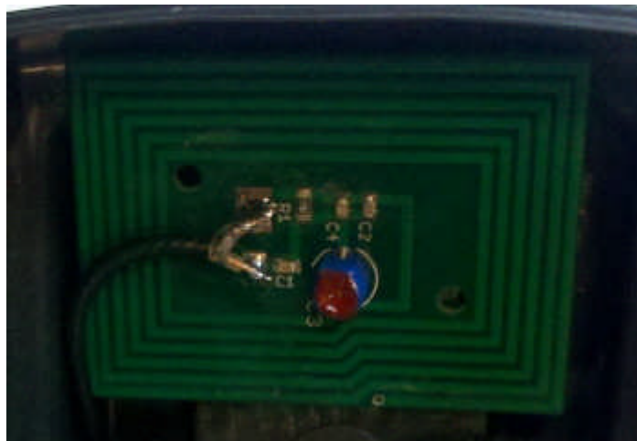
RFID Antenna PCB Top
