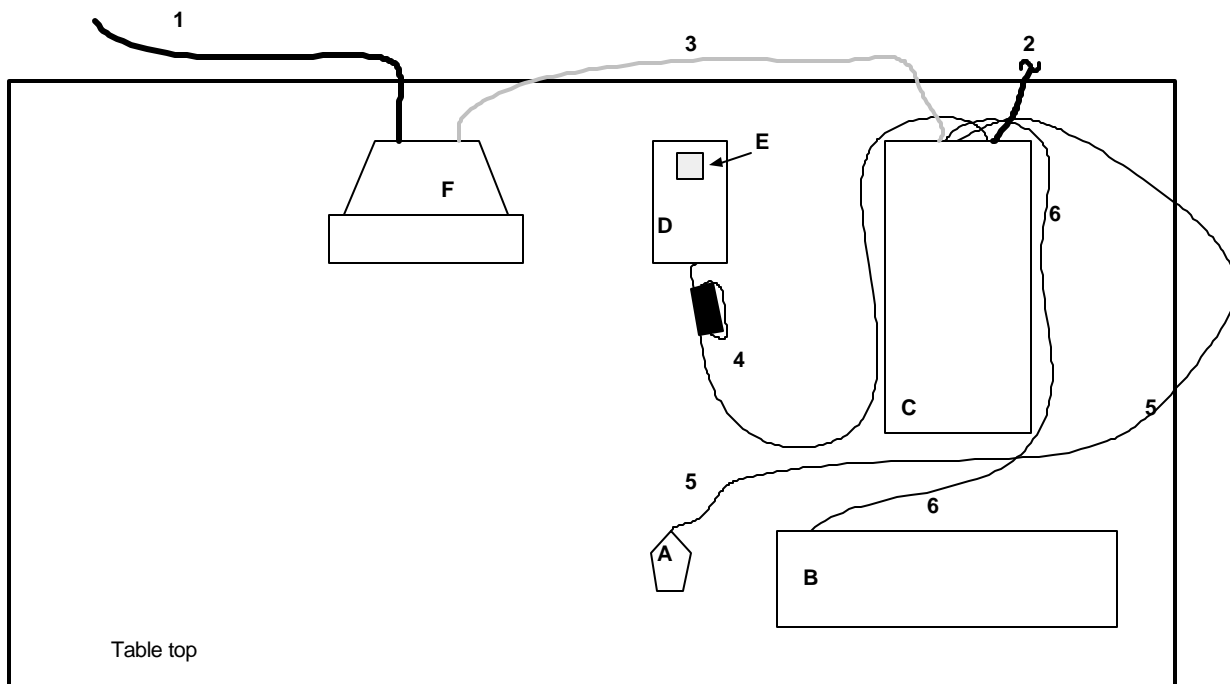
Figure 6. Basic EUT Setup (Legend designation is on previous page)
