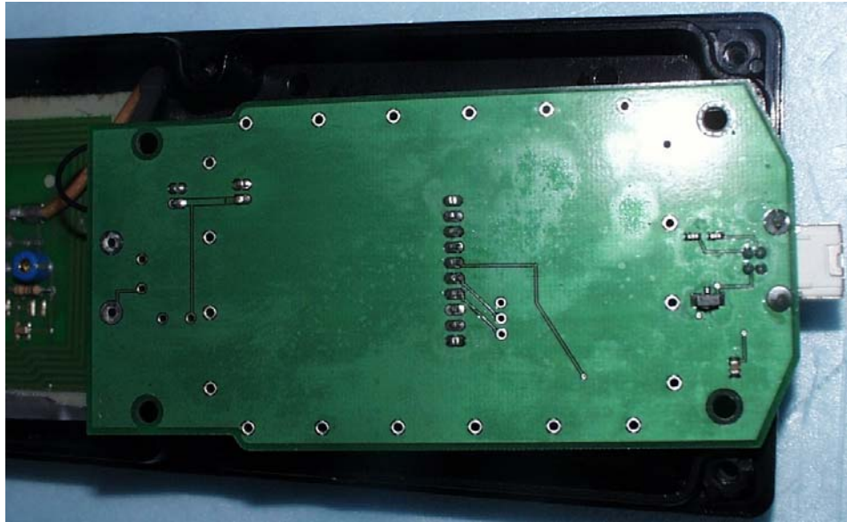
Close up of back of USB / RS232 converter
