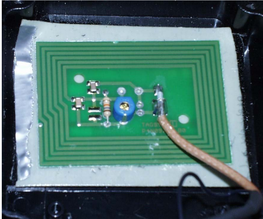
Antenna assembly
