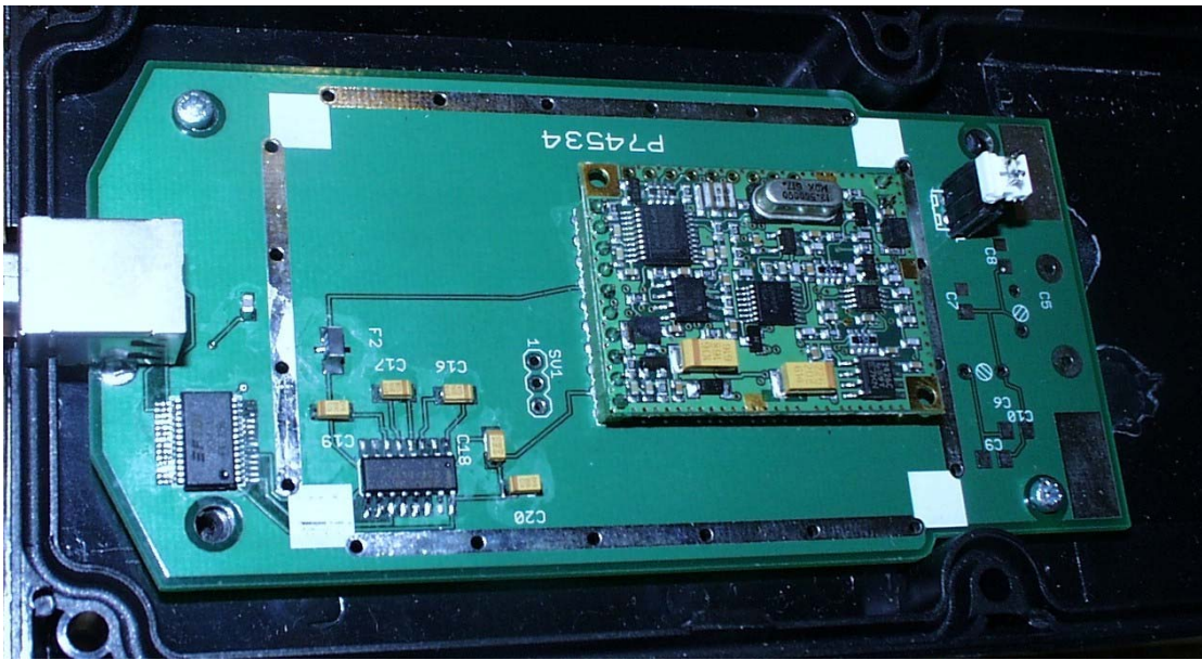
Close-up of RFID coupler attached to the USB / RS232 converter circuit board
