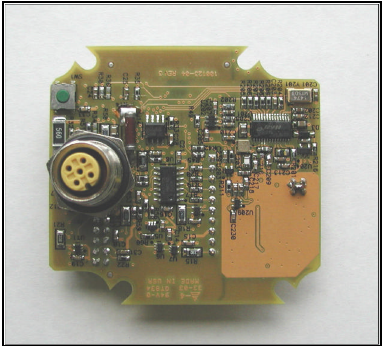
PHOTOGRAPH 37: iEFM (BACK)
