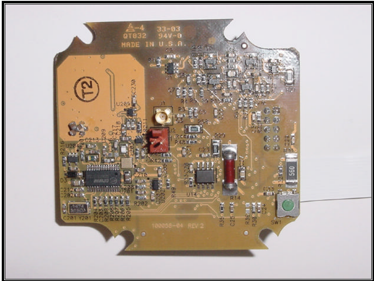
PHOTOGRAPH 34: iTLM-1 BOTTOM
