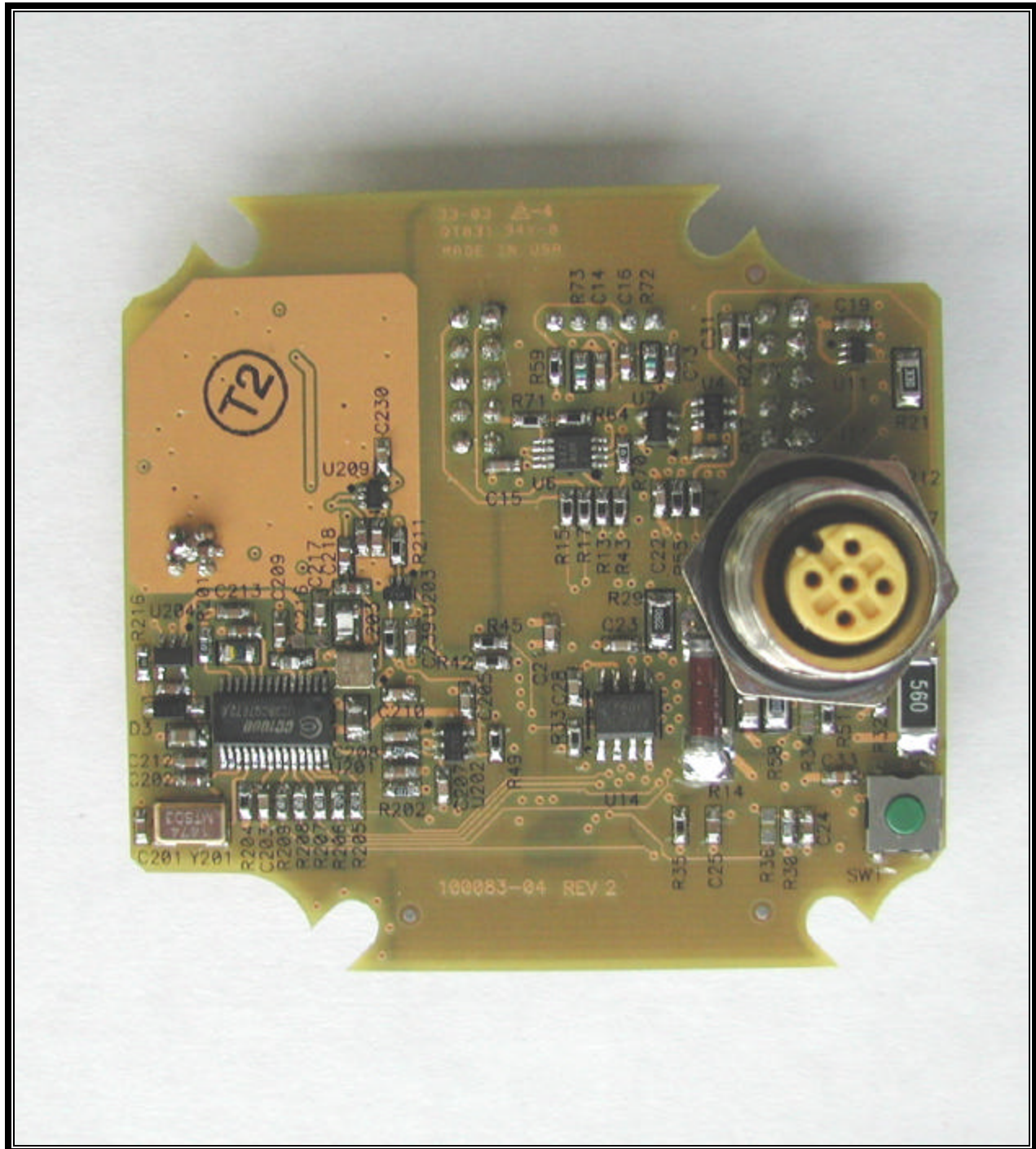
PHOTOGRAPH 39: iWPM-T (BACK)
