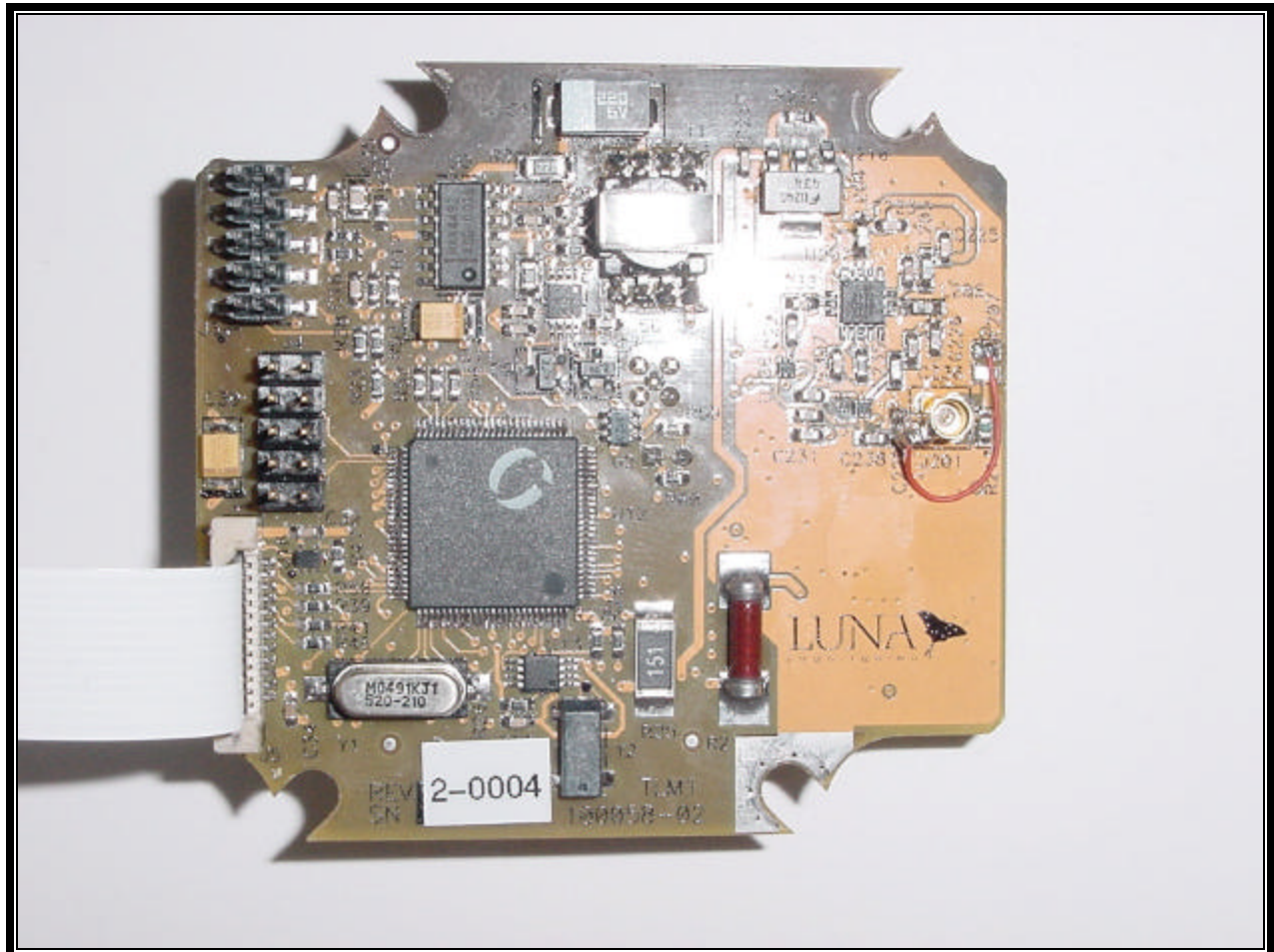
PHOTOGRAPH 33: iTLM-1 TOP
