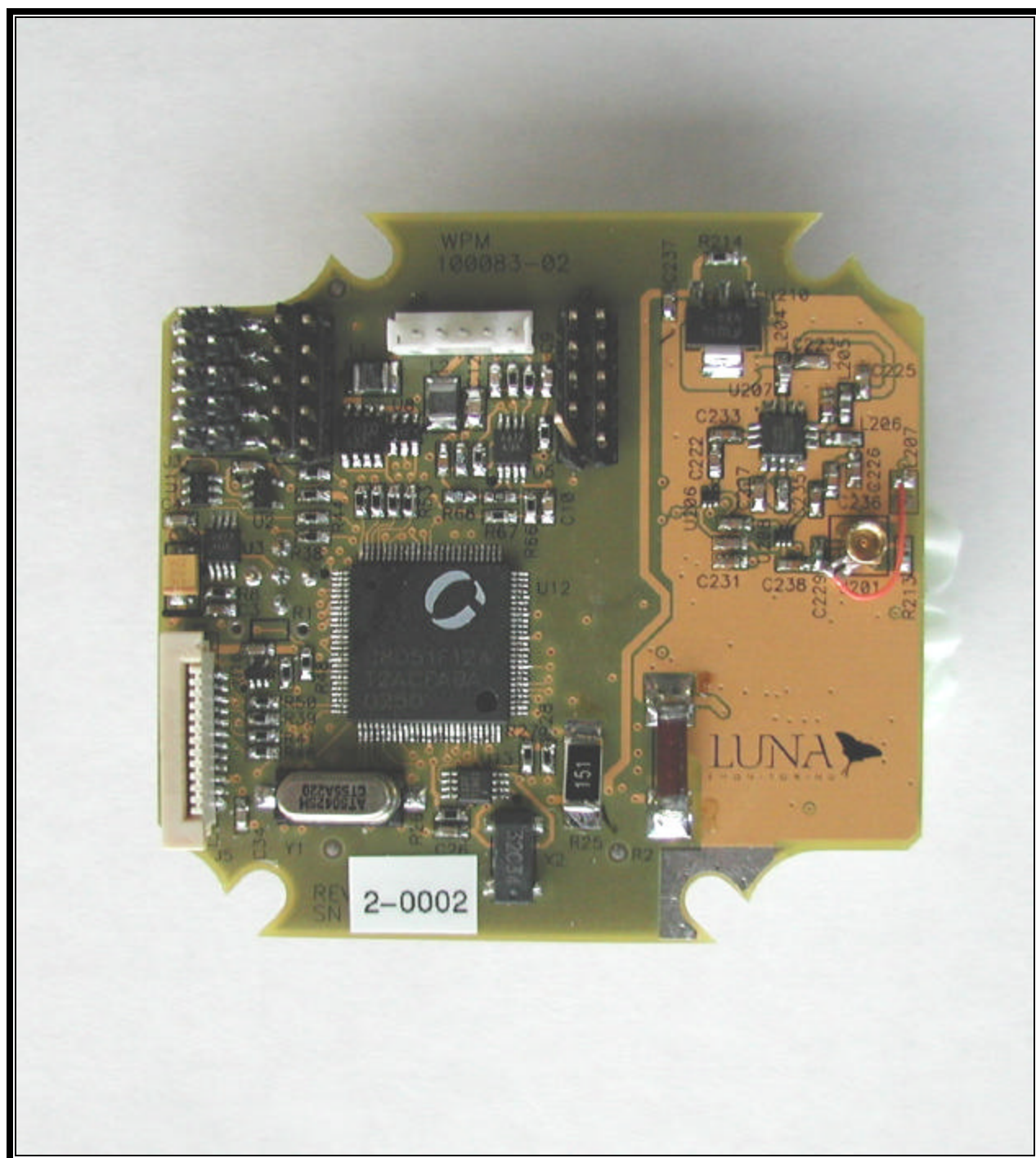
PHOTOGRAPH 38: iWPM-T (FRONT)
