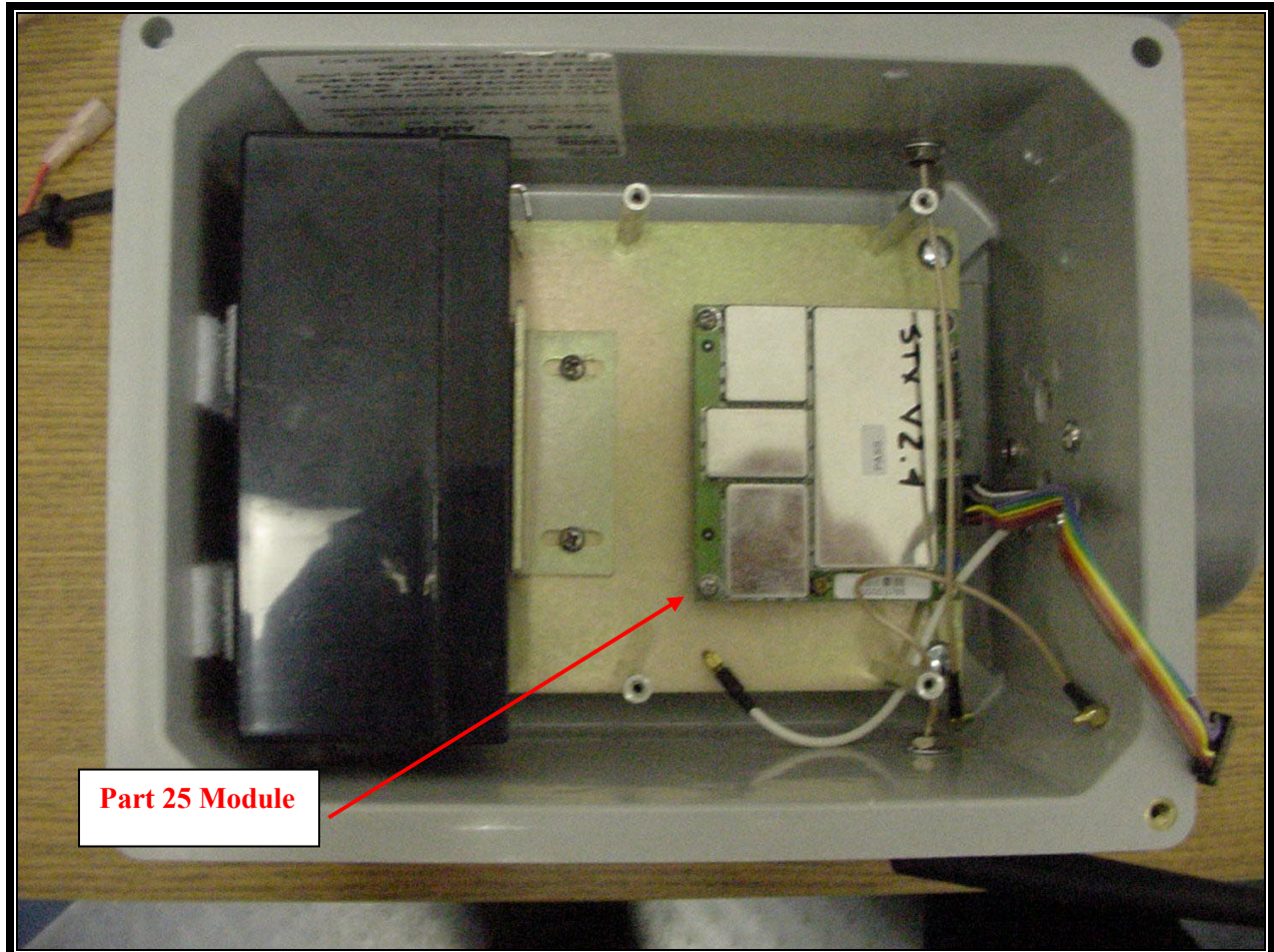
PHOTOGRAPH 11: LOCATION OF PART 25 MODULE
