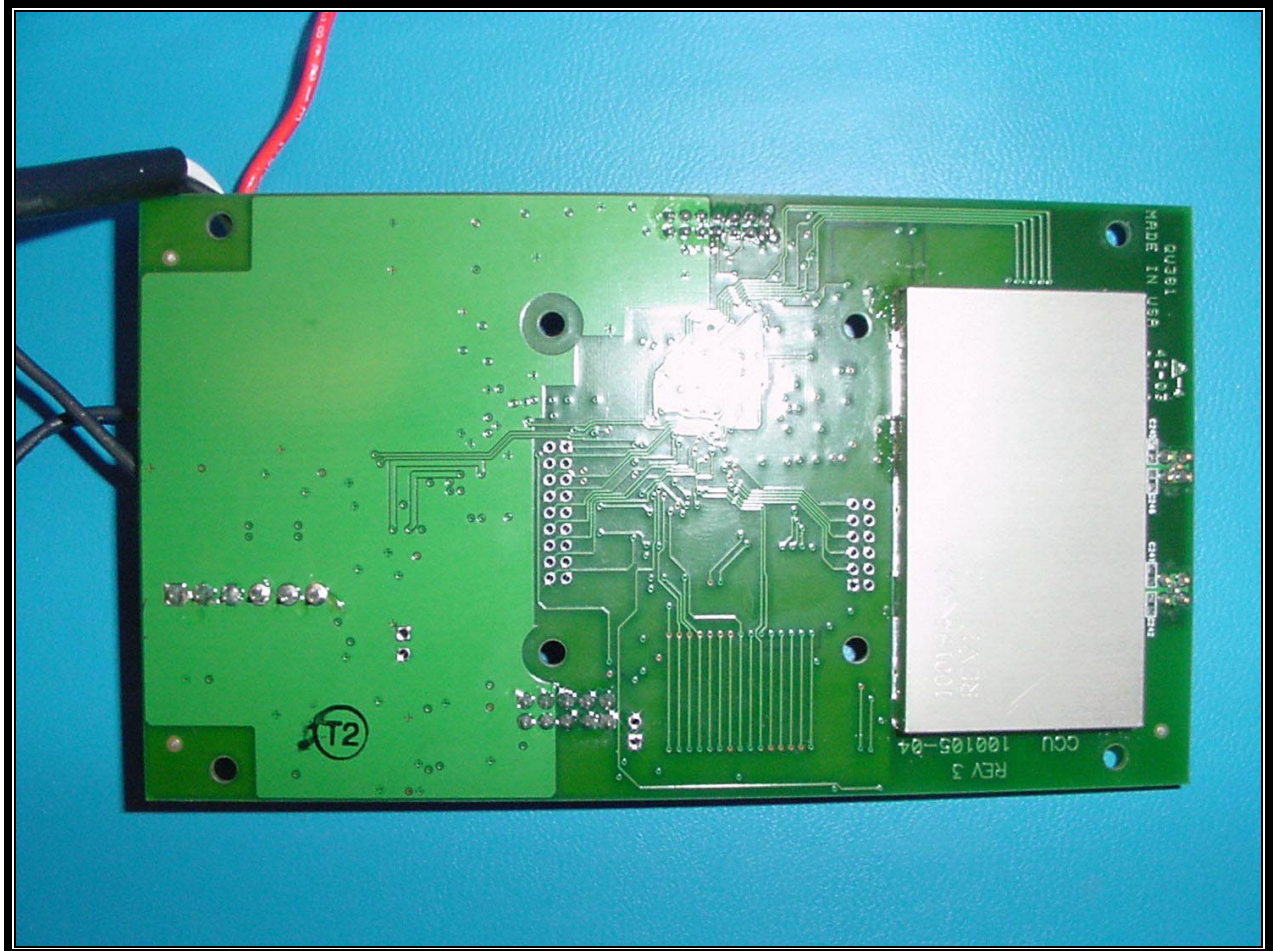
PHOTOGRAPH 9: PCB REAR WITH SHIELD
