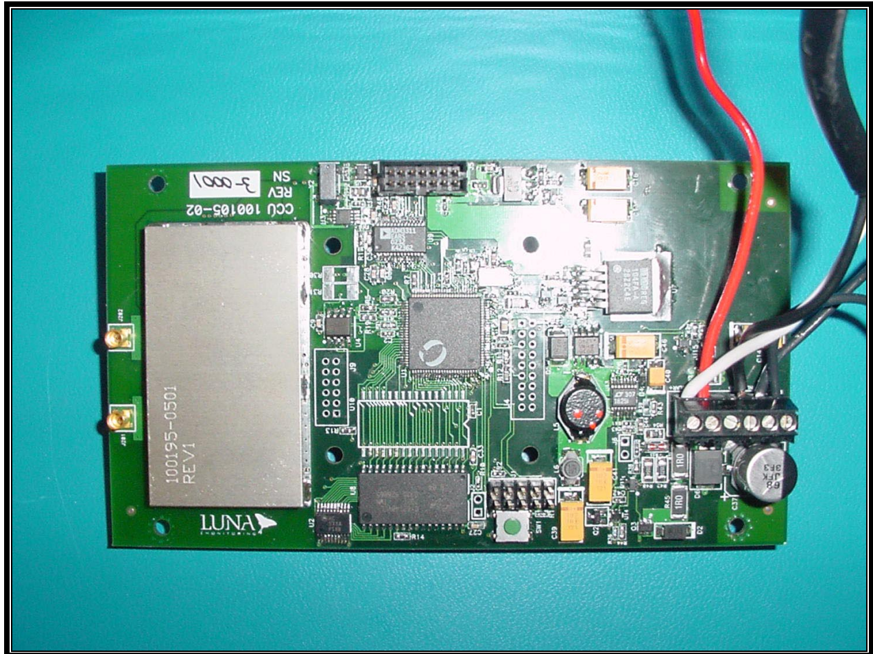
PHOTOGRAPH 7: PCB FRONT WITH SHIELD
