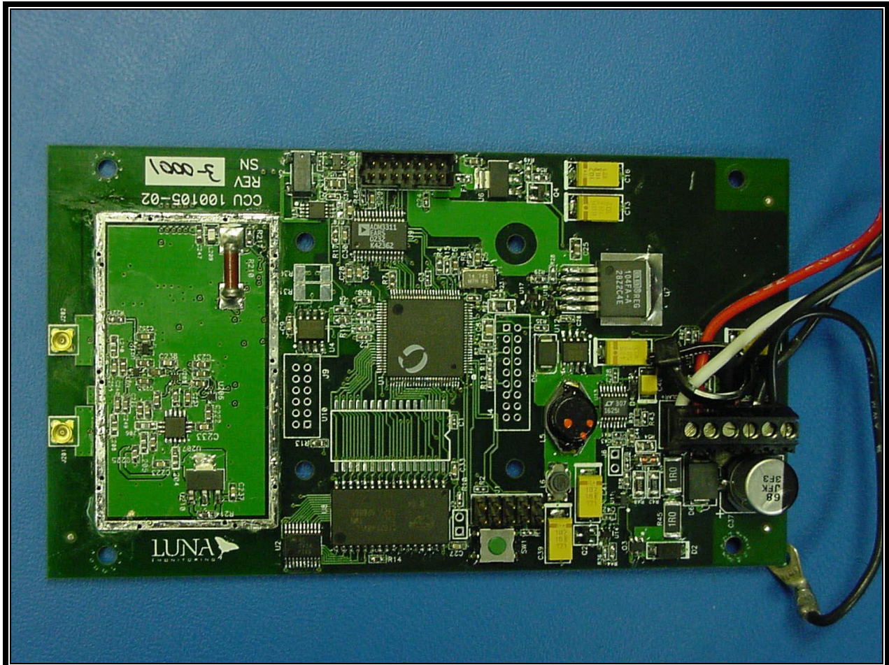
PHOTOGRAPH 8: PCB FRONT WITHOUT SHIELD
