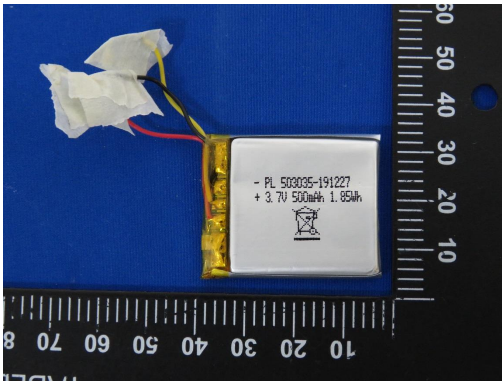
Battery: PL503035
