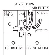
Figure 6: RECOMMENDED SMOKE DETECTORS LOCATIONS TO AVOID AIR STREAMS WITH COMBUSTION PARTICLES
