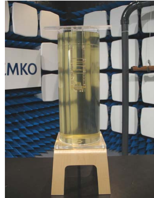
Test set-up, EUT in Plexiglas cylinder
