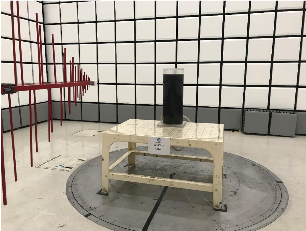
Radiated Emission Below 1GHz Front View
