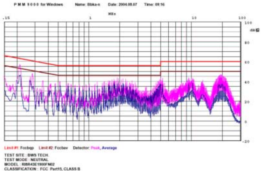
Plots of Power Line Conducted Emission
