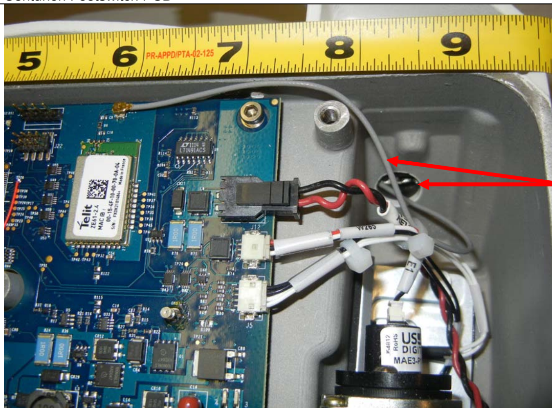
Centurion Footswitch PCB
