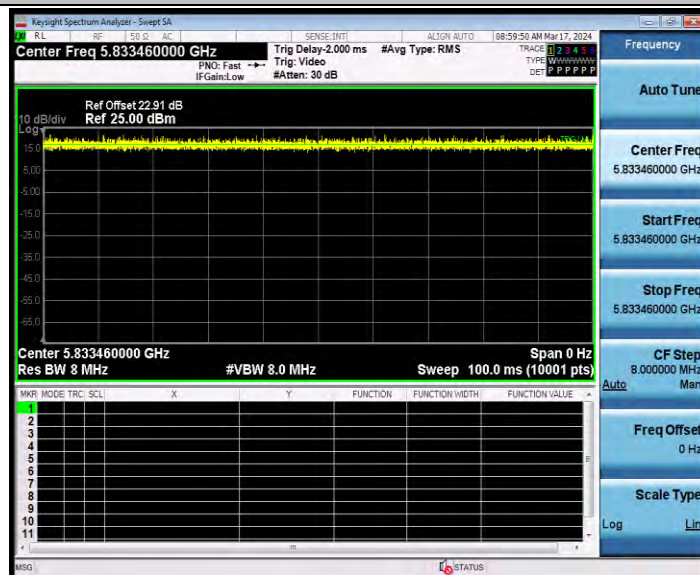
11AX20SISO_Ant1_5825_52Tone_RU40
