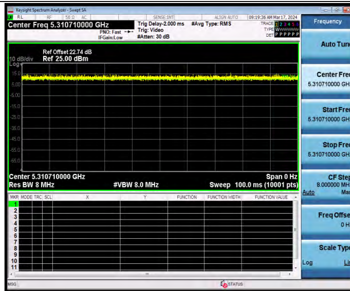
11AX40SISO_Ant2_5310_484Tone_RU65
