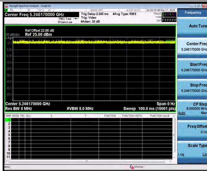
11AX20SISO_Ant1_5240_106Tone_RU54
