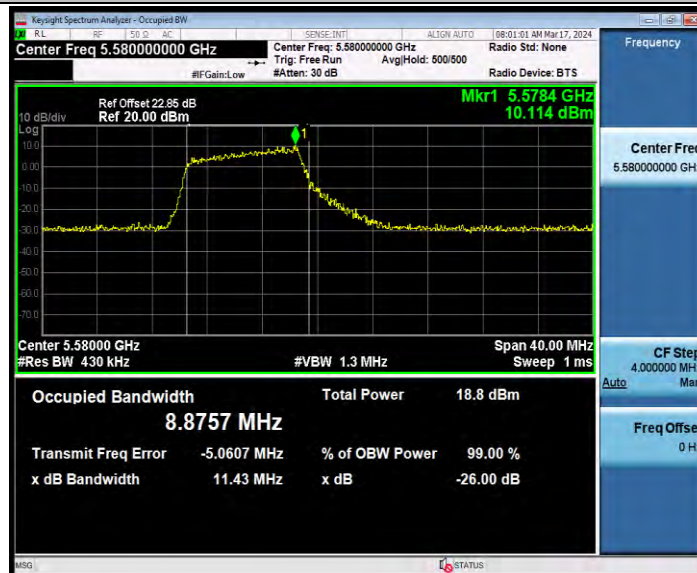
11AX20SISO_Ant1_5580_242Tone_RU61
