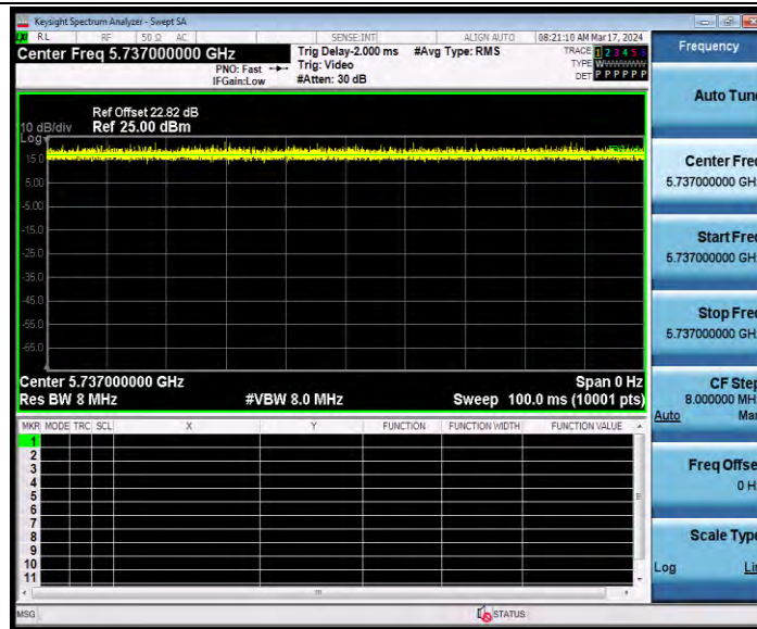
11AX20SISO_Ant1_5745_52Tone_RU37
