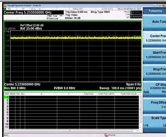
11AX40SISO_Ant2_5230_484Tone_RU65
