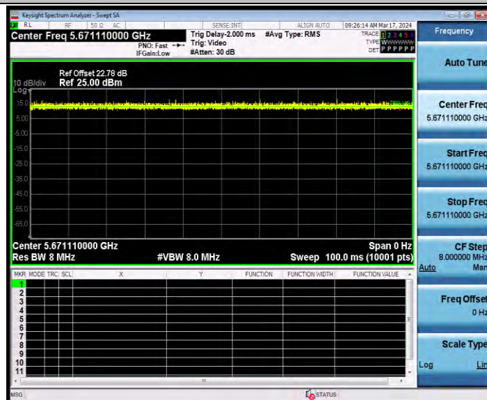
11AX40SISO_Ant2_5670_484Tone_RU65
