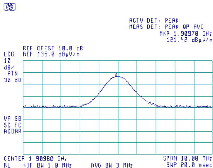
Plot 8.1.11 Transmitter carrier field strength at high frequency in vertical antenna polarization, EUT horizontal position
