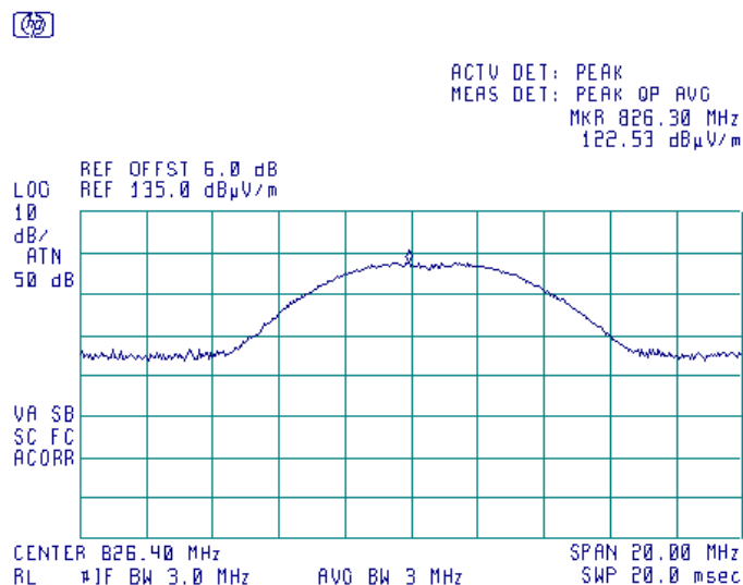
Plot 7.1.14 Transmitter carrier field strength at low frequency in horizontal antenna polarization, EUT vertical position
