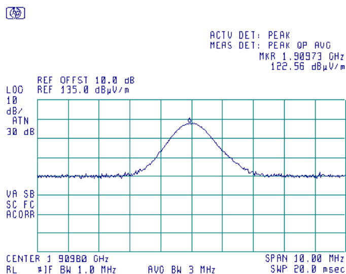
Plot 8.1.12 Transmitter carrier field strength at high frequency in horizontal antenna polarization, EUT horizontal position
