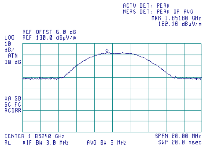
Plot 8.1.14 Transmitter carrier field strength at low frequency in horizontal antenna polarization, EUT vertical position
