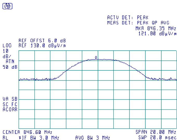
Plot 7.1.23 Transmitter carrier field strength at high frequency in vertical antenna polarization, EUT horizontal position
