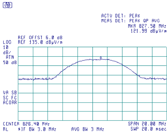
Plot 7.1.13 Transmitter carrier field strength at low frequency in vertical antenna polarization, EUT vertical position
