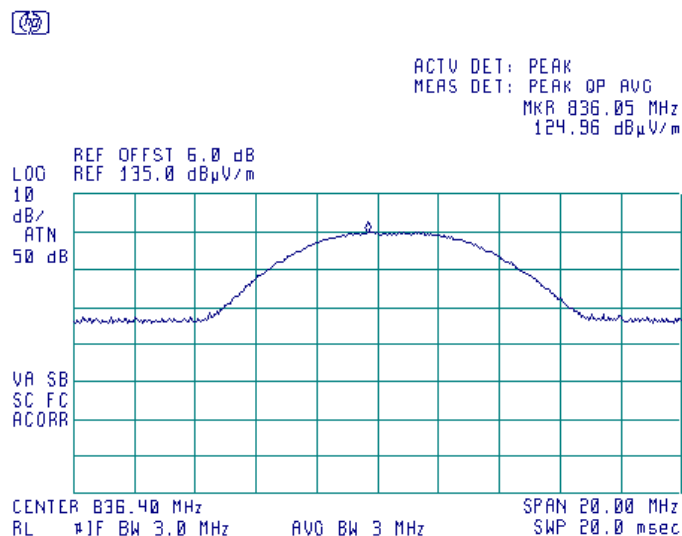
Plot 7.1.20 Transmitter carrier field strength at mid frequency in horizontal antenna polarization, EUT horizontal position
