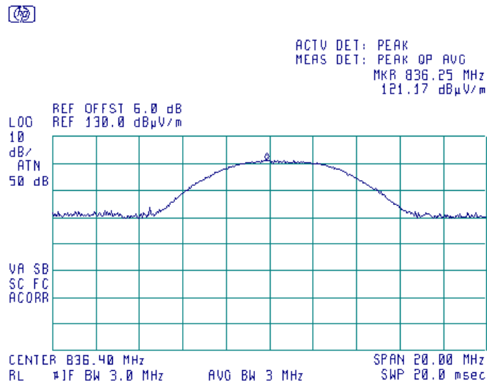
Plot 7.1.19 Transmitter carrier field strength at mid frequency in vertical antenna polarization, EUT horizontal position
