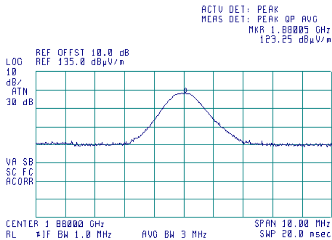
Plot 8.1.6 Transmitter carrier field strength at mid frequency in horizontal antenna polarization, EUT vertical position
