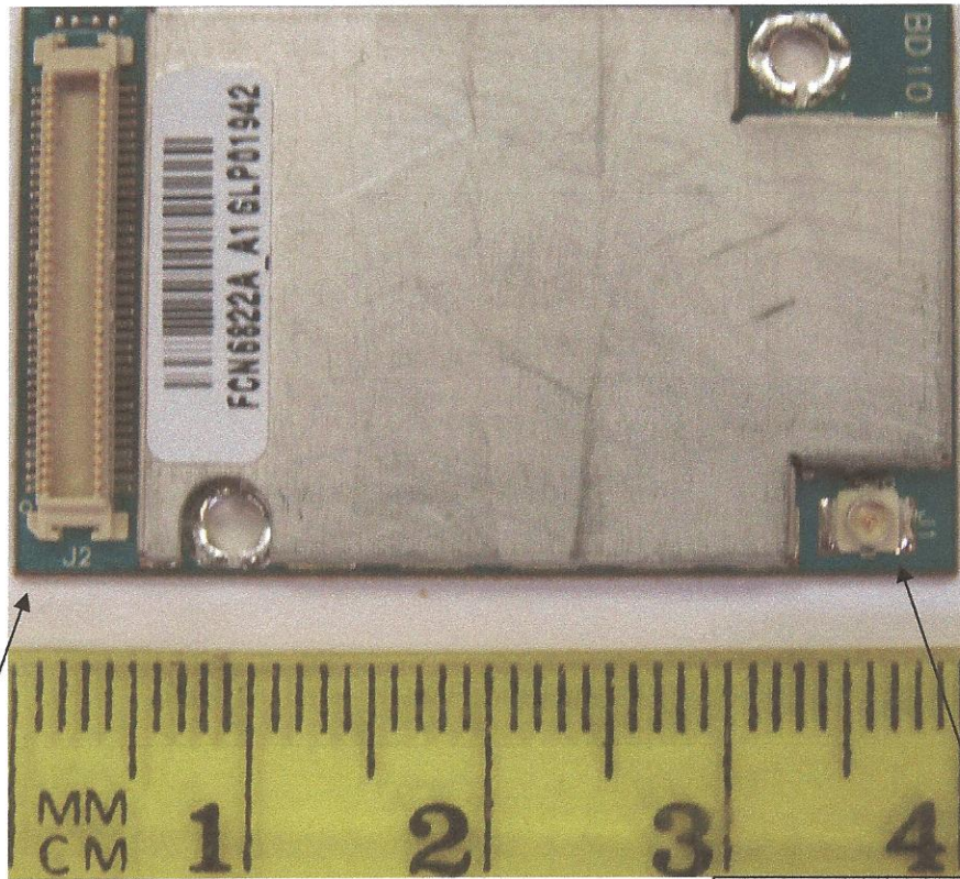
UFL Main RF Connector
