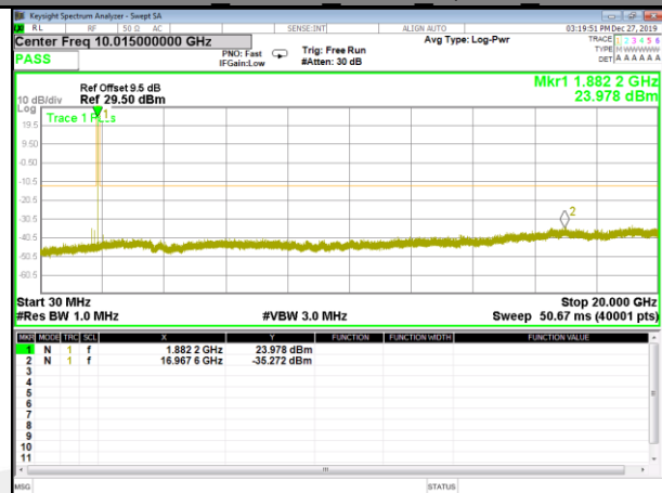
Band 25 15KHz 12#0 QPSK Mid
