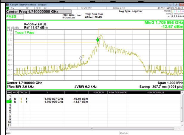
Band 4 15KHz 1#0 BPSK Low
