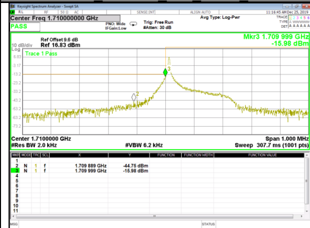
Band 4 3.75KHz 1#47 BPSK High
