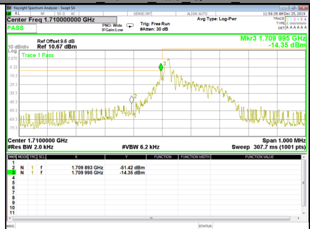
Band 4 15KHz 1#0 QPSK Low
