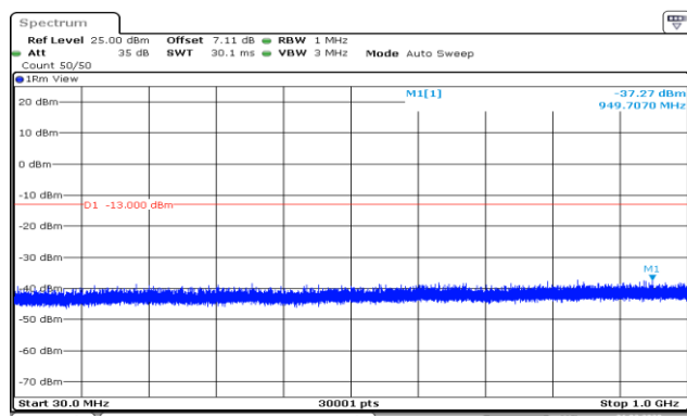
GPRS_1900_Lower(30MHz-1GHz)
