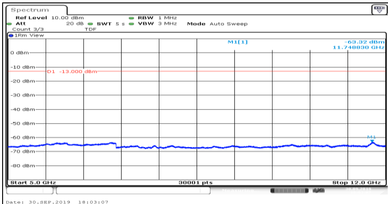
Band85_5MHz_QPSK_134092_1
