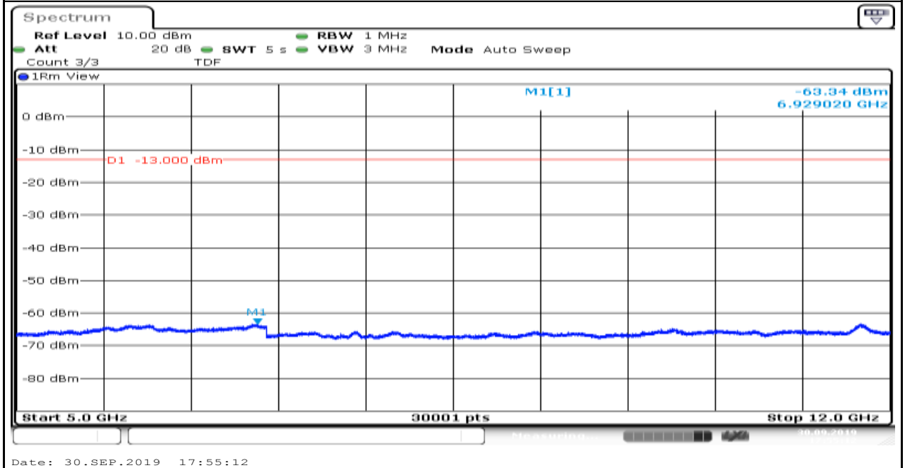
Band85_5MHz_QPSK_134027_6
