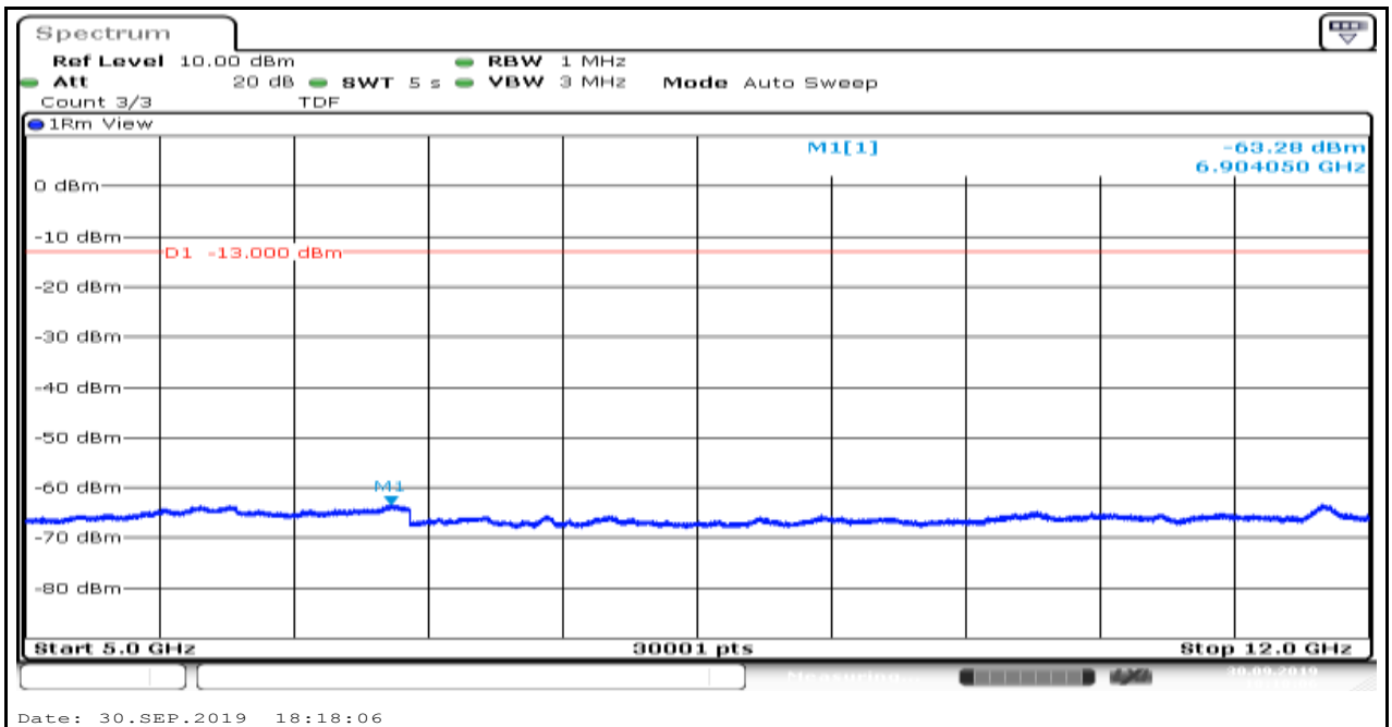
Band85_5MHz_16QAM_134157_1
