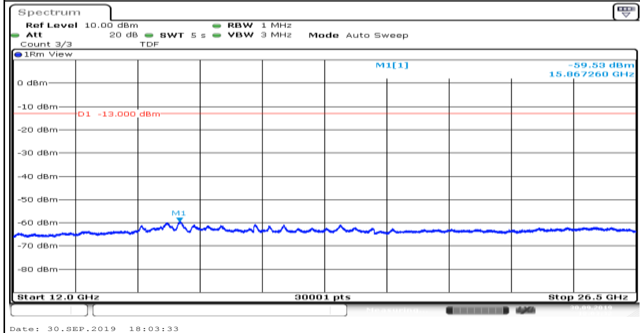
Band85_5MHz_QPSK_134092_6
