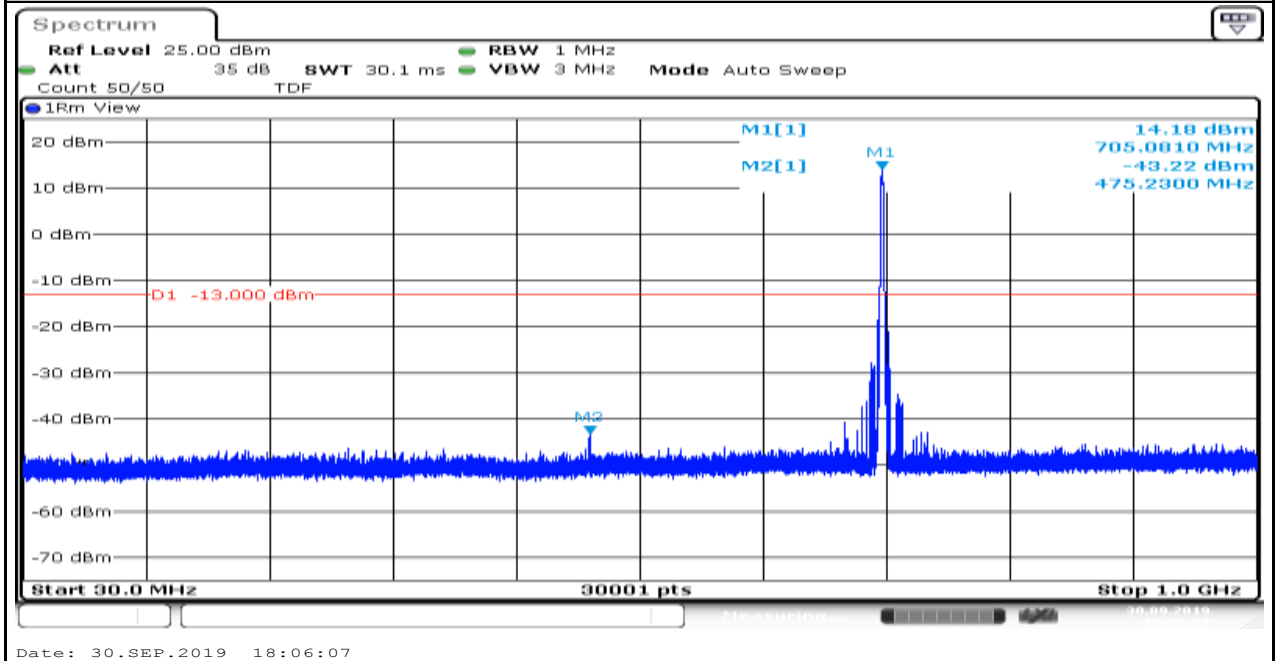
Band85_5MHz_QPSK_134157_1
