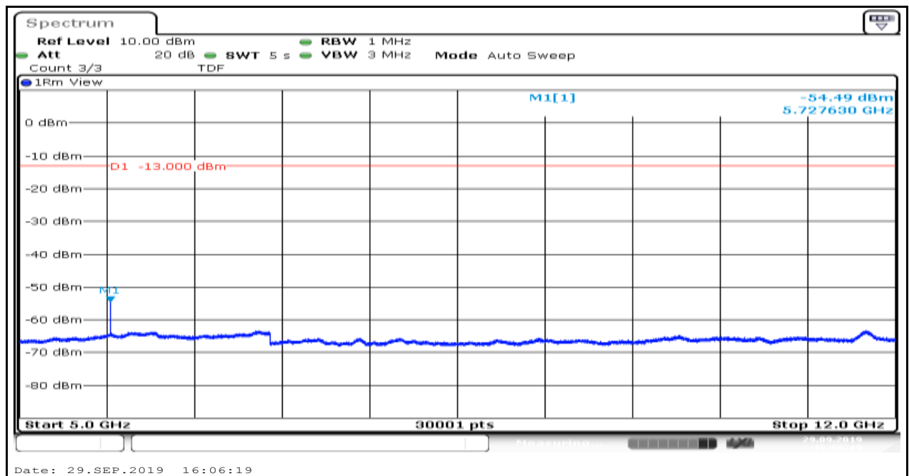
Band2_1.4MHz_QPSK_19193_6
