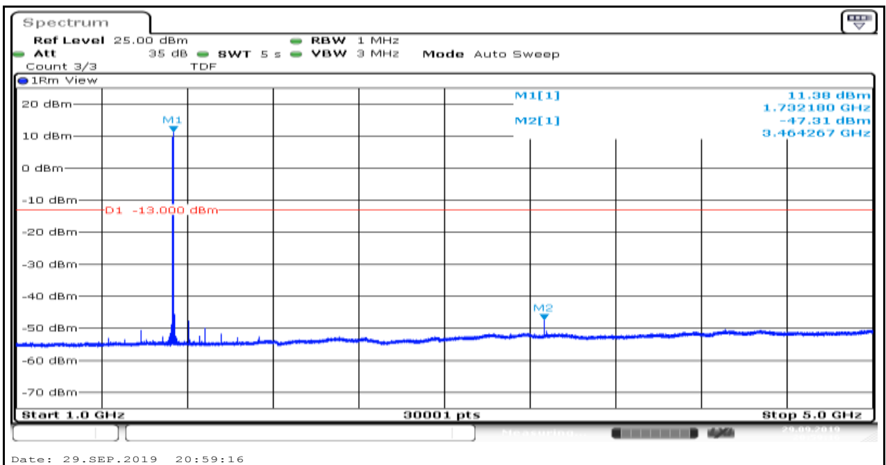
Band4_1.4MHz_16QAM_20393_1
