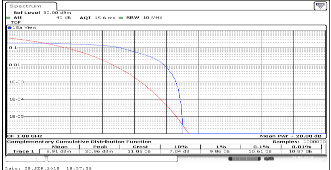
Band2_10MHz_16QAM_18900_6
