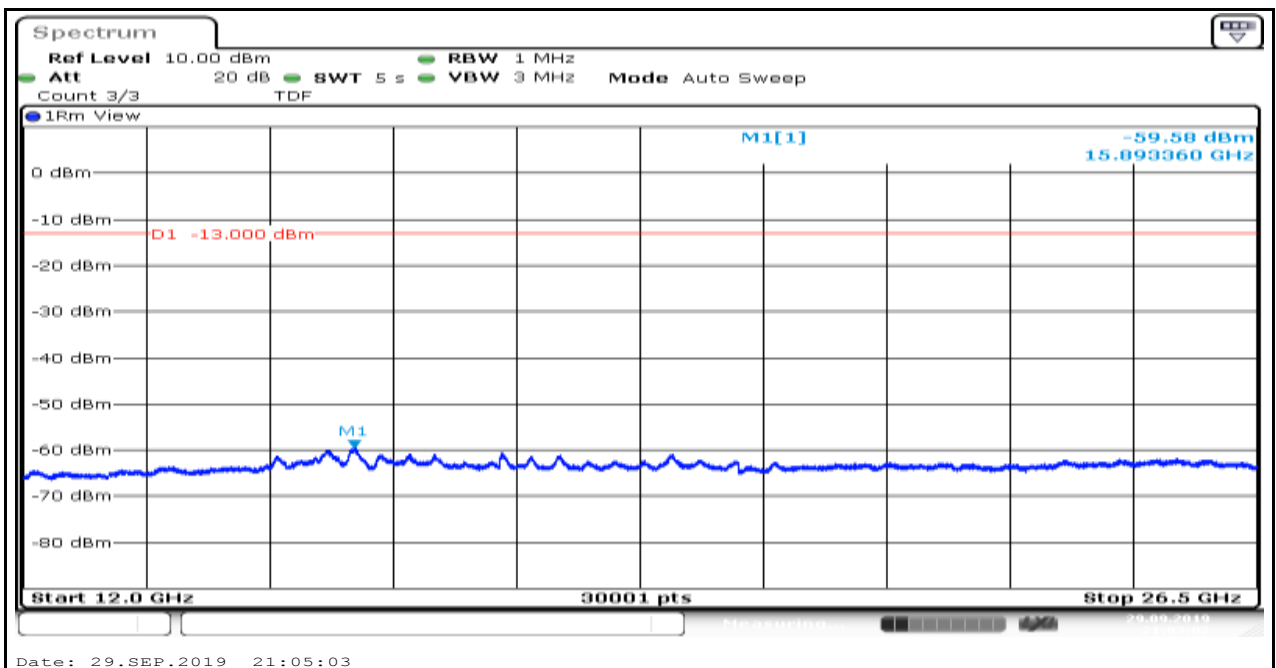
Band4_1.4MHz_16QAM_19957_1
