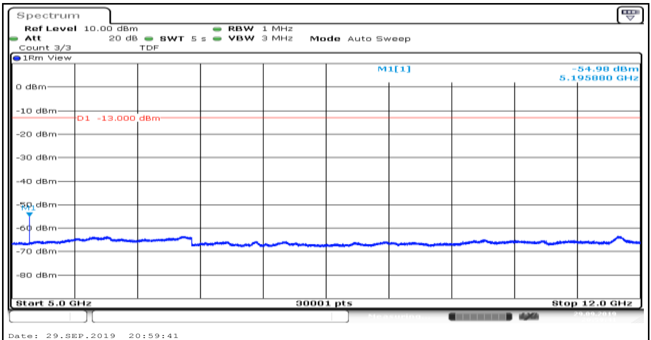
Band4_1.4MHz_16QAM_20175_1
