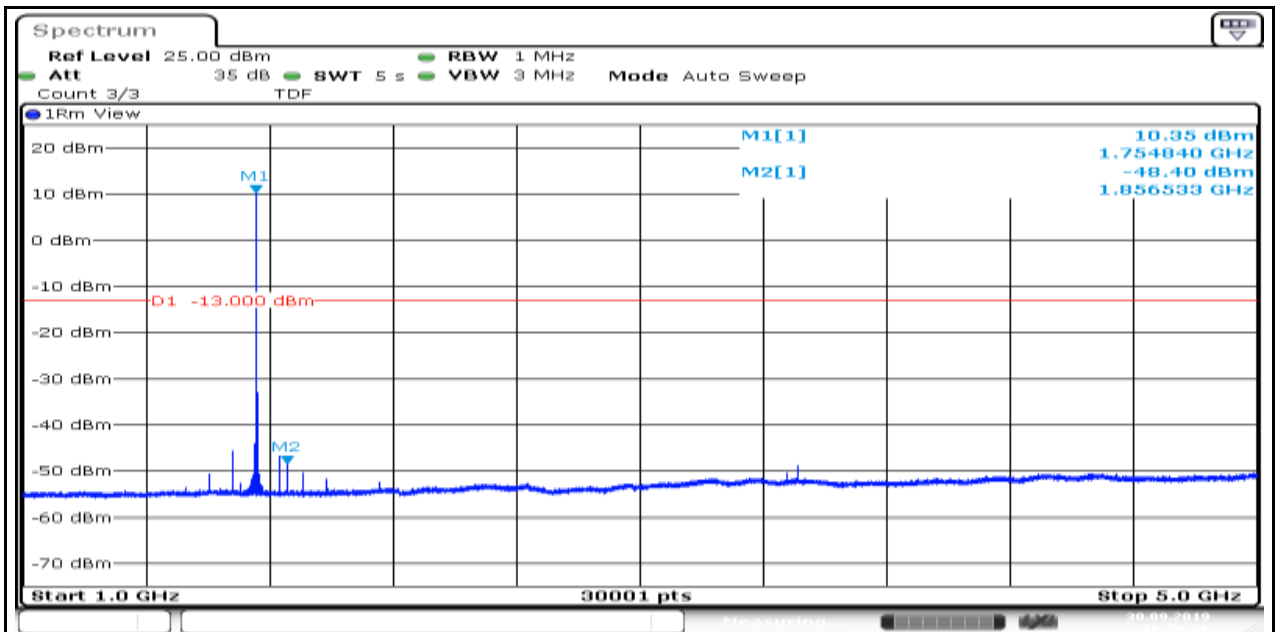
Band4_1.4MHz_16QAM_20393_1
