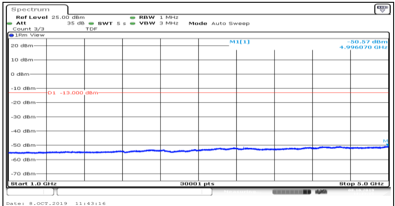
Band5_1.4MHz_QPSK_20525_1
