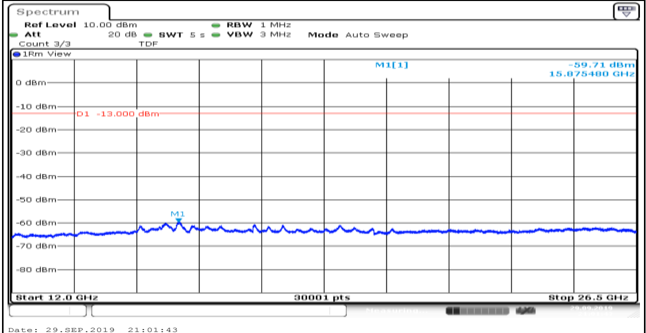
Band4_1.4MHz_QPSK_20175_1
