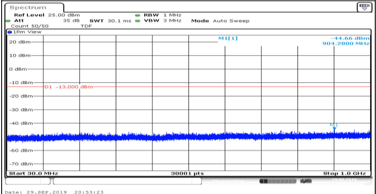
Band4_1.4MHz_QPSK_19957_6
