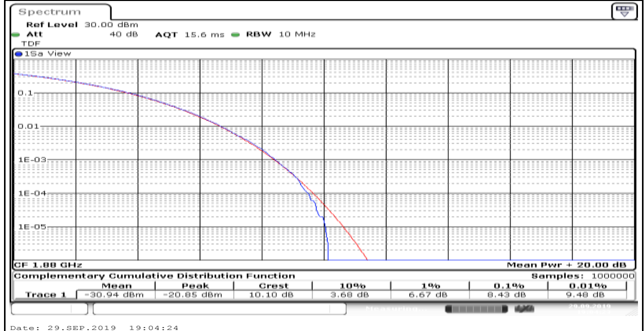
Band2_1.4MHz_QPSK_18900_6
