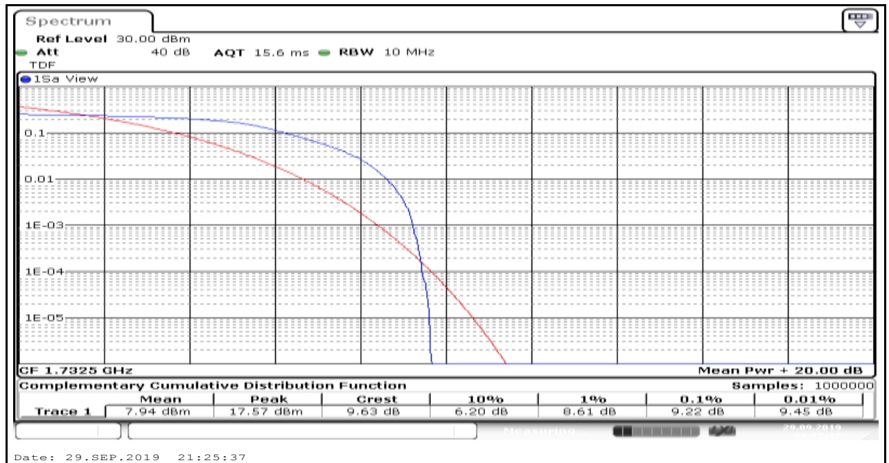
Band4_15MHz_QPSK_20175_6
