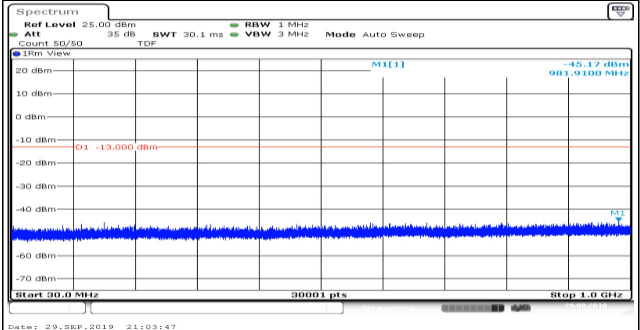
Band4_1.4MHz_QPSK_20393_5
