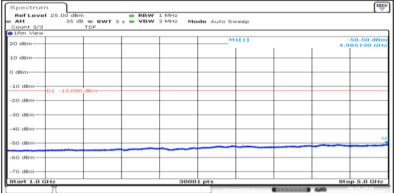
Band5_1.4MHz_QPSK_20407_6
