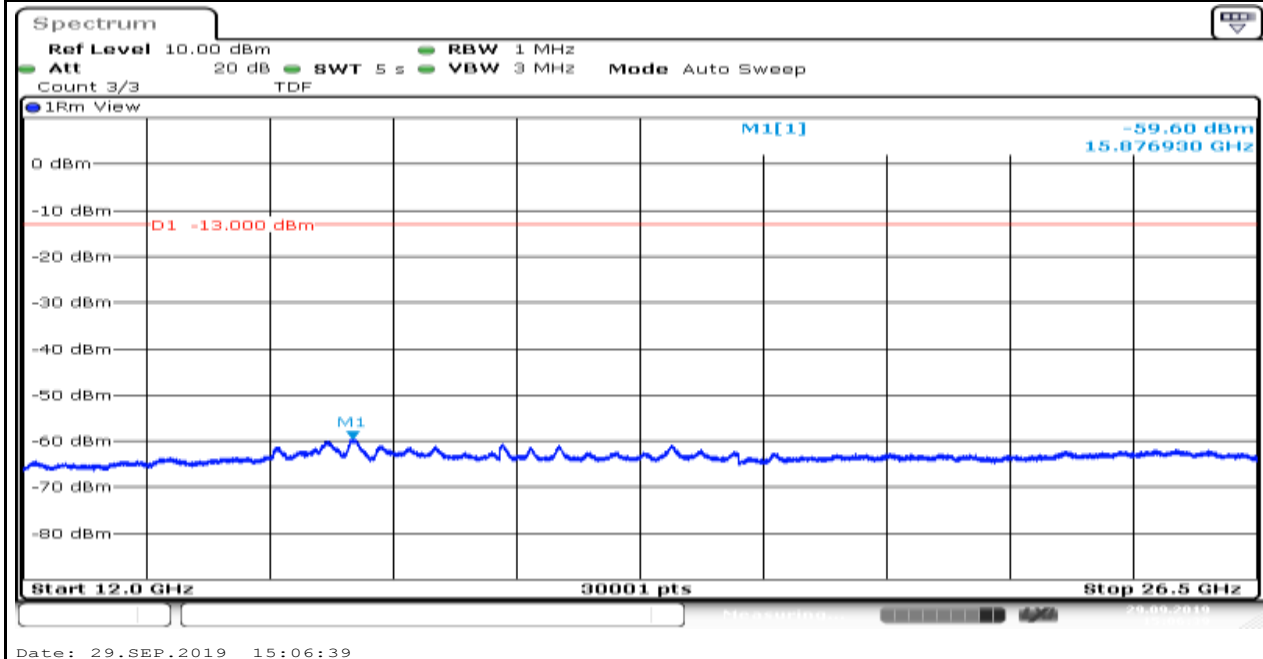
Band2_1.4MHz_16QAM_18607_1
