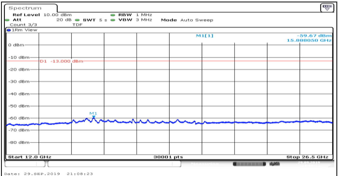
Band4_1.4MHz_QPSK_20393_6
