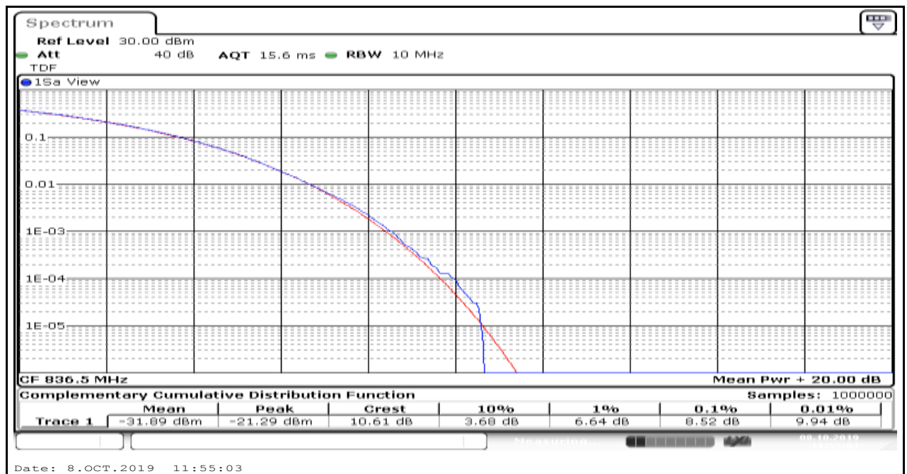
Band5_1.4MHz_QPSK_20525_6
