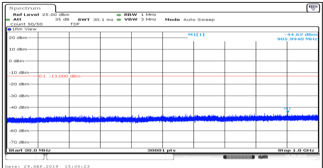
Band2_1.4MHz_16QAM_18607_6
