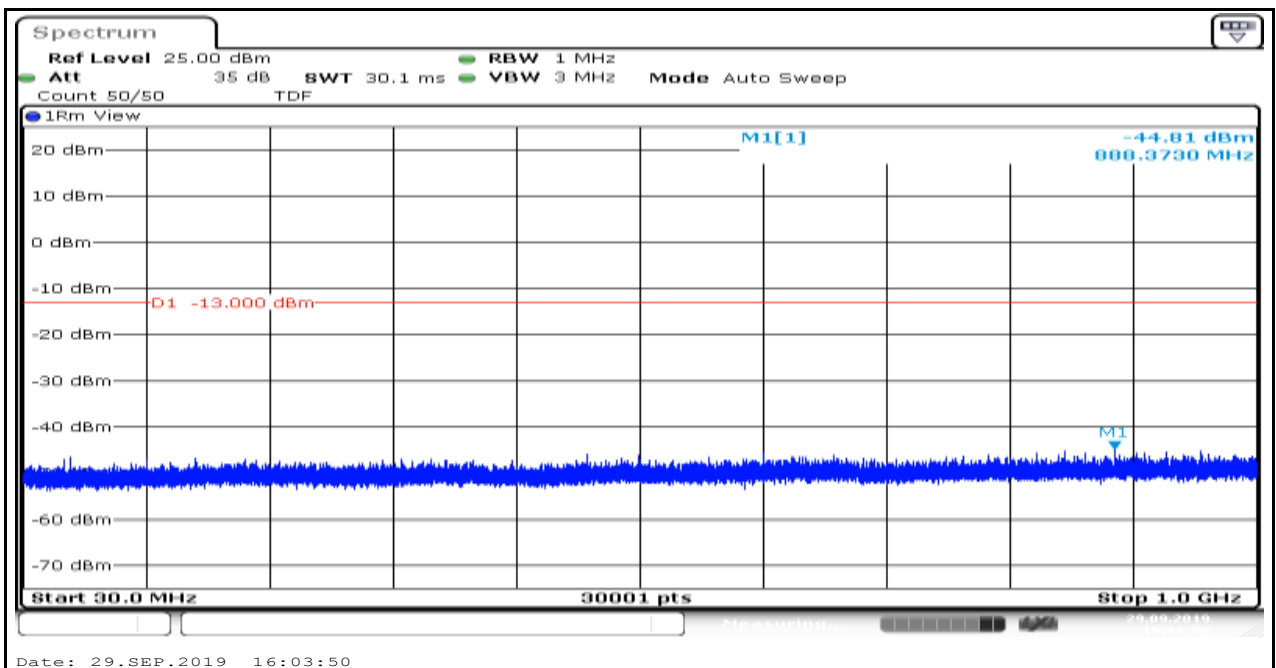
Band2_1.4MHz_16QAM_19193_1
