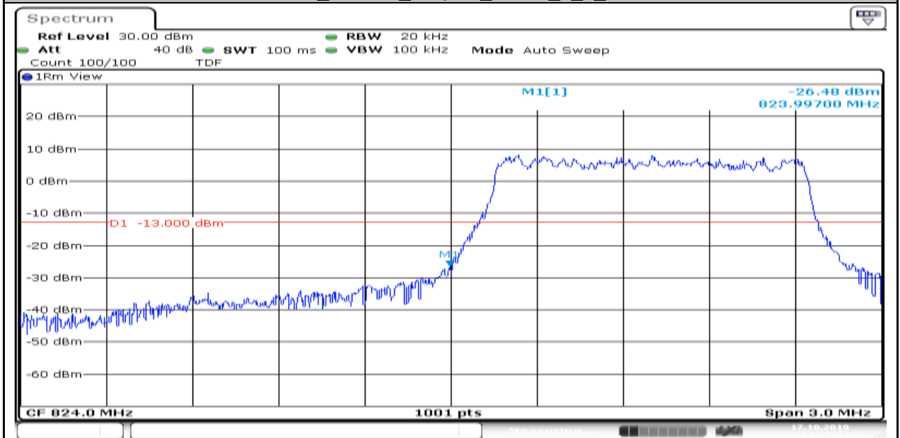
Band5_1.4MHz_16QAM_20407_6_0_Low
