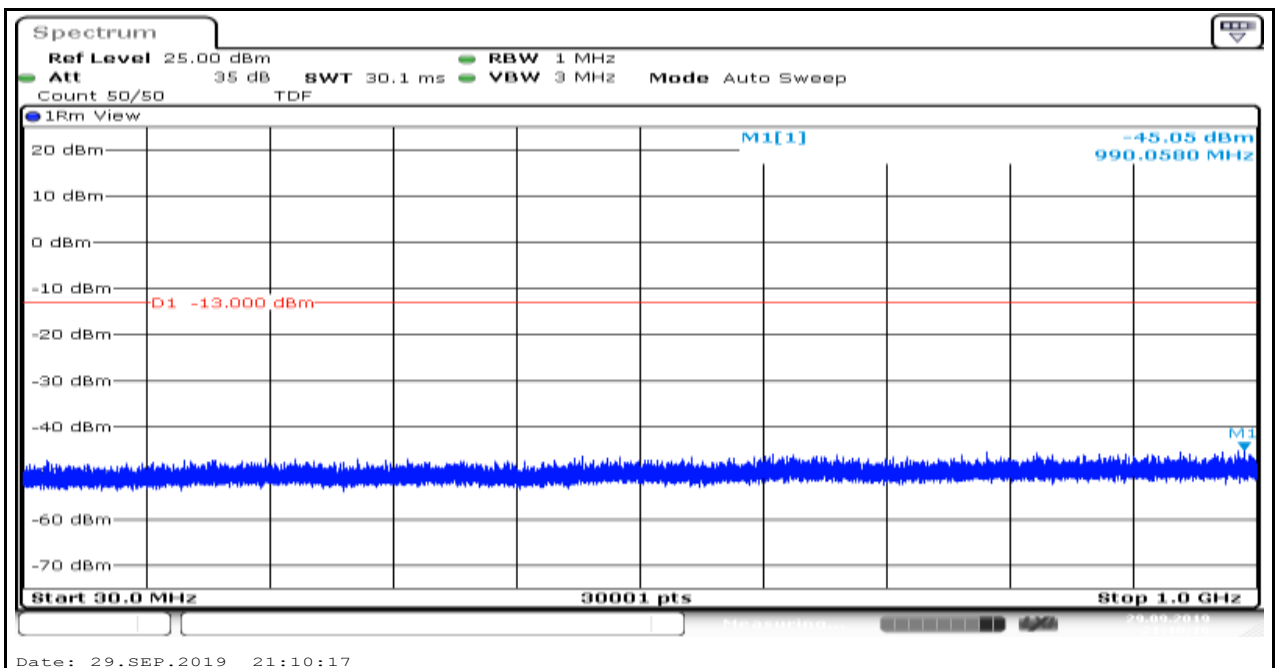
Band4_1.4MHz_16QAM_20393_5
