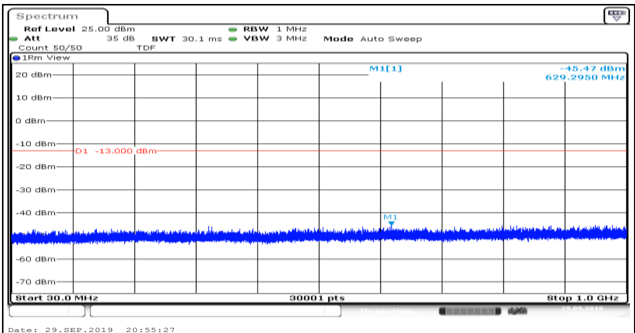
Band4_1.4MHz_16QAM_19957_6
