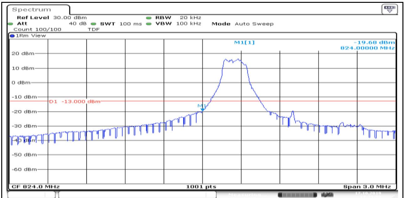
Band5_1.4MHz_16QAM_20643_6_0_Low
