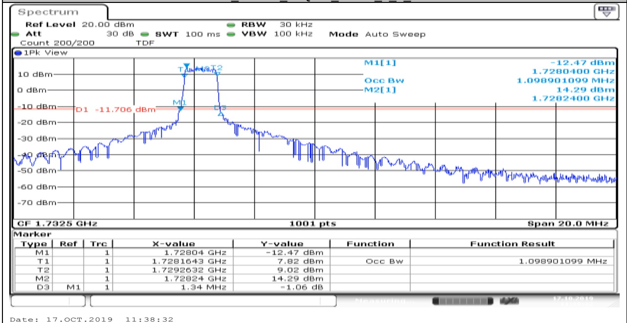
Band4_20MHz_16QAM_20175_6_0_Low
