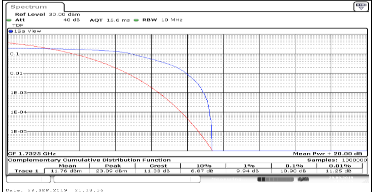
Band4_20MHz_16QAM_20175_6
