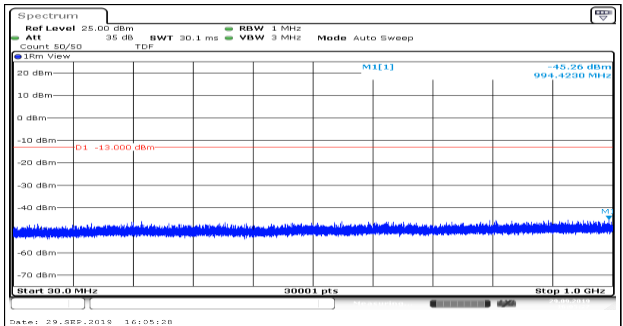
Band2_1.4MHz_QPSK_19193_1
