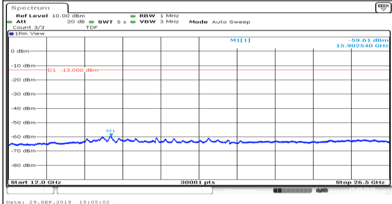
Band2_1.4MHz_QPSK_18607_1
