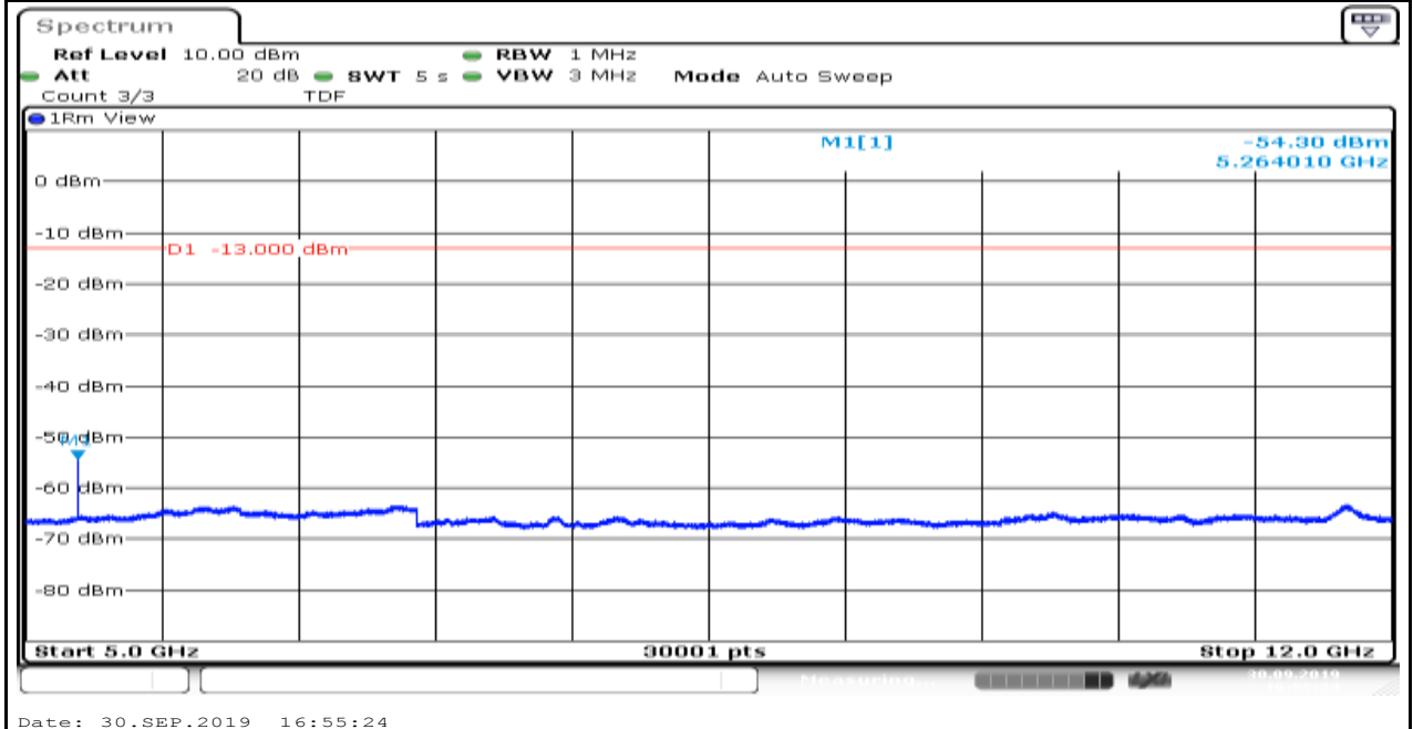
Band4_1.4MHz_QPSK_20393_6
