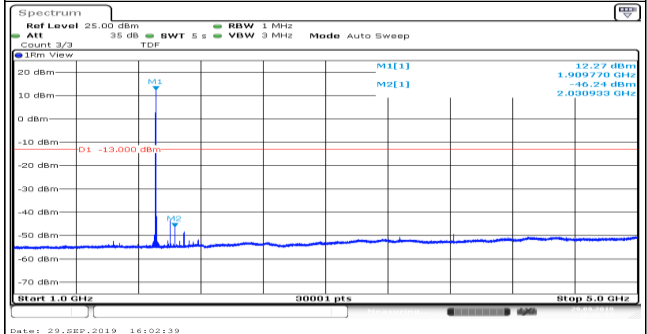
Band2_1.4MHz_QPSK_19193_6
