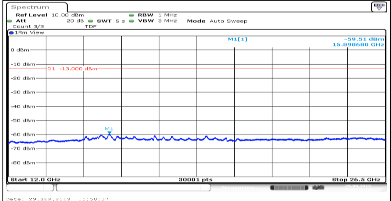
Band2_1.4MHz_16QAM_19193_1
