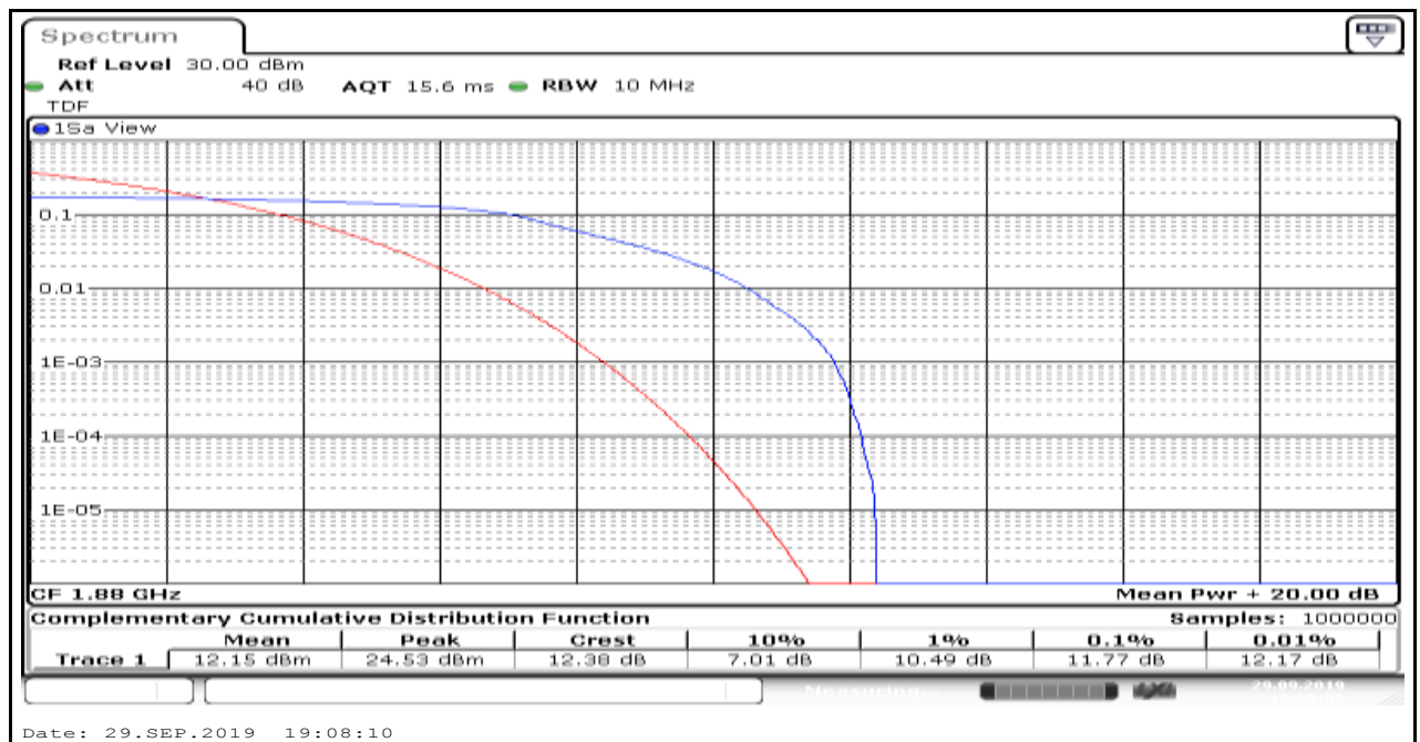
Band2_3MHz_16QAM_18900_6
