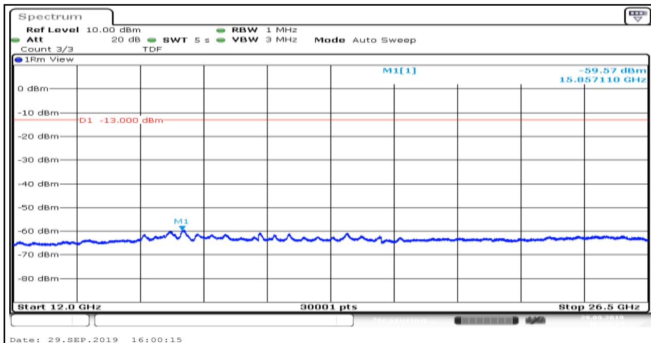
Band2_1.4MHz_QPSK_18900_6
