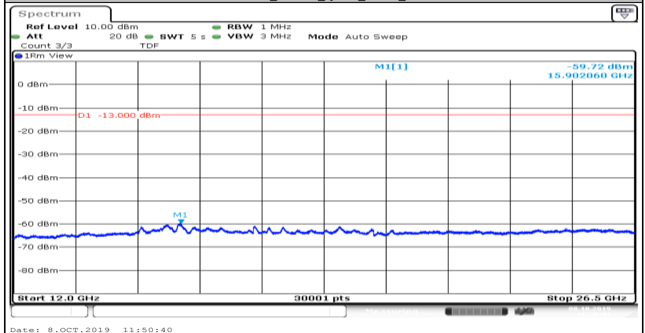
Band5_1.4MHz_QPSK_20525_6
