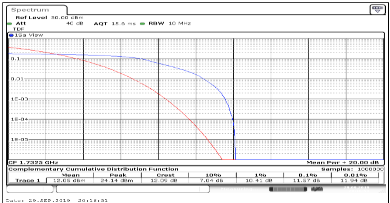
Band4_5MHz_16QAM_20175_6
