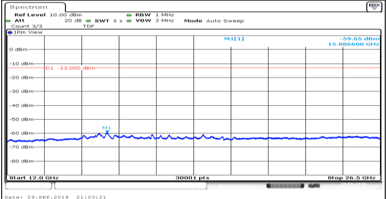
Band4_1.4MHz_16QAM_20175_1
