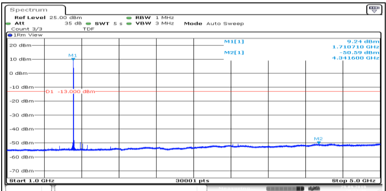
Band4_1.4MHz_QPSK_19957_6
