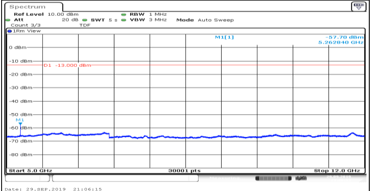
Band4_1.4MHz_16QAM_20393_6
