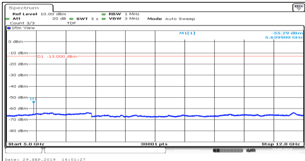
Band2_1.4MHz_16QAM_18900_6
