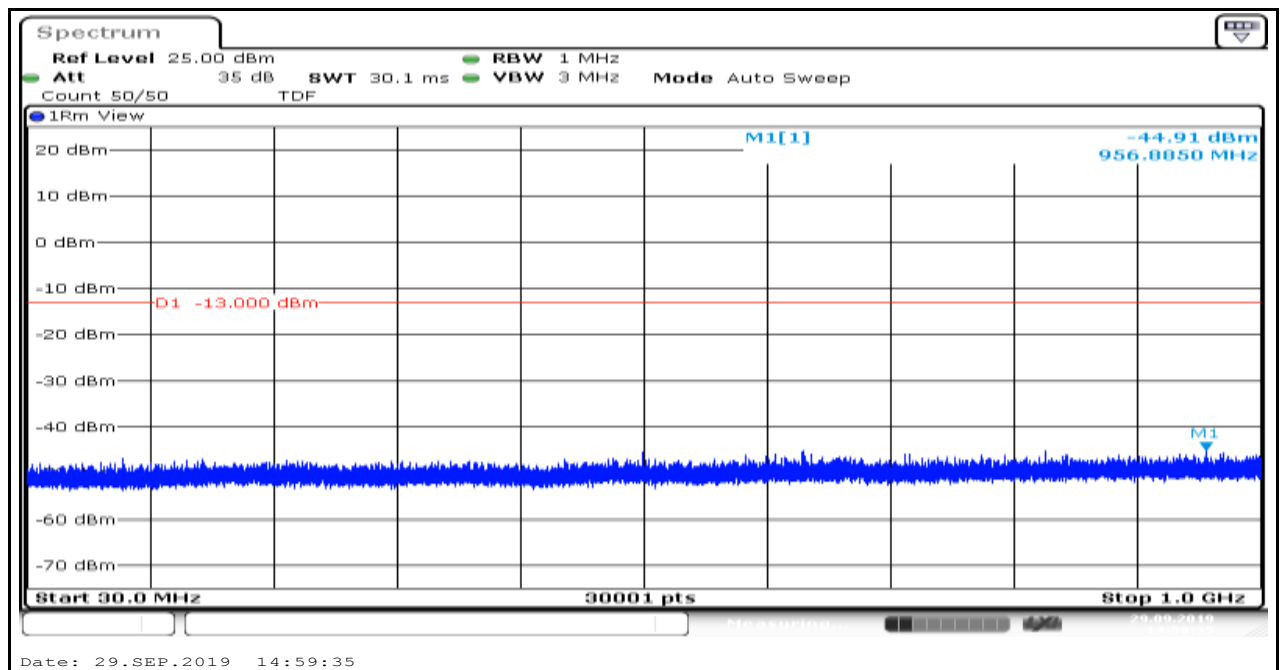
Band2_1.4MHz_QPSK_18607_6
