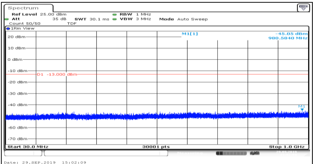
Band2_1.4MHz_16QAM_18607_1
