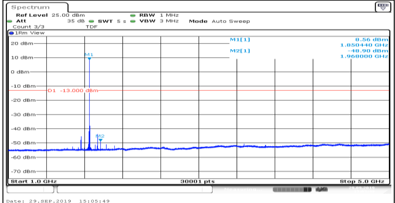
Band2_1.4MHz_16QAM_18607_6
