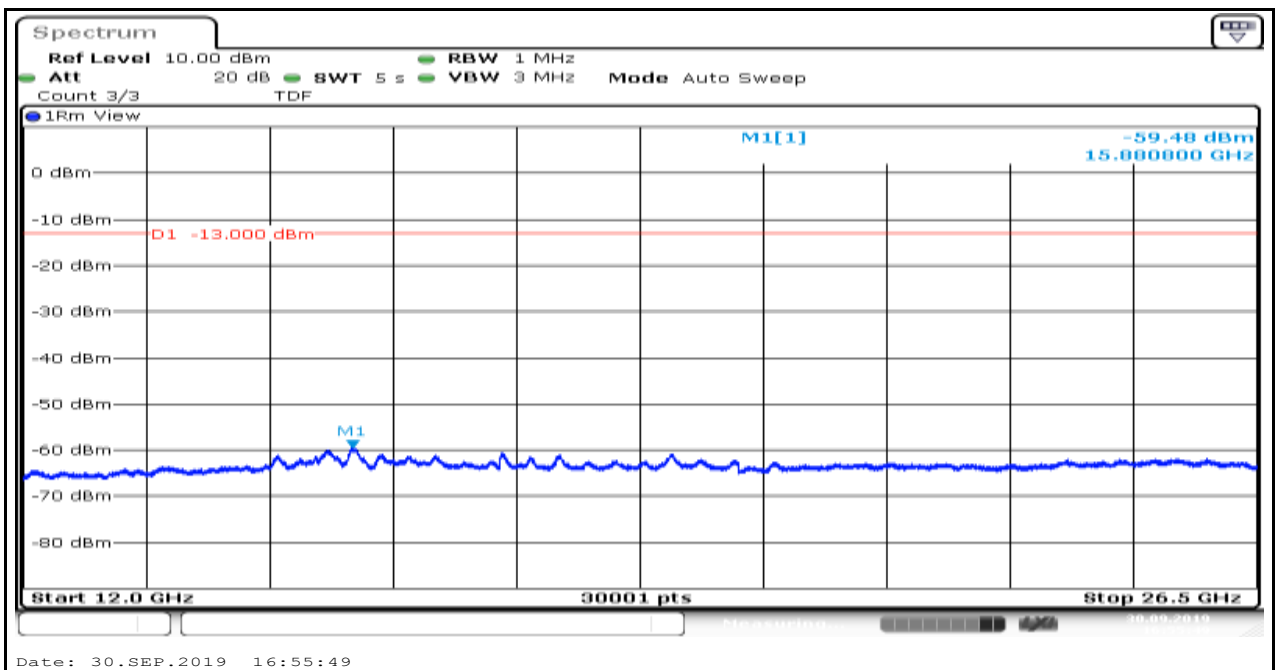
Band4_1.4MHz_QPSK_20393_1
