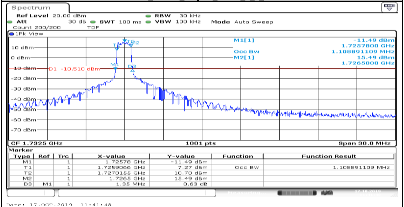
Band4_5MHz_16QAM_20175_6_0_Low
