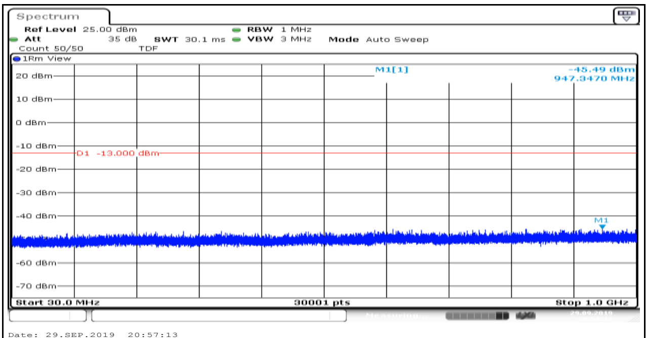
Band4_1.4MHz_QPSK_20175_6
