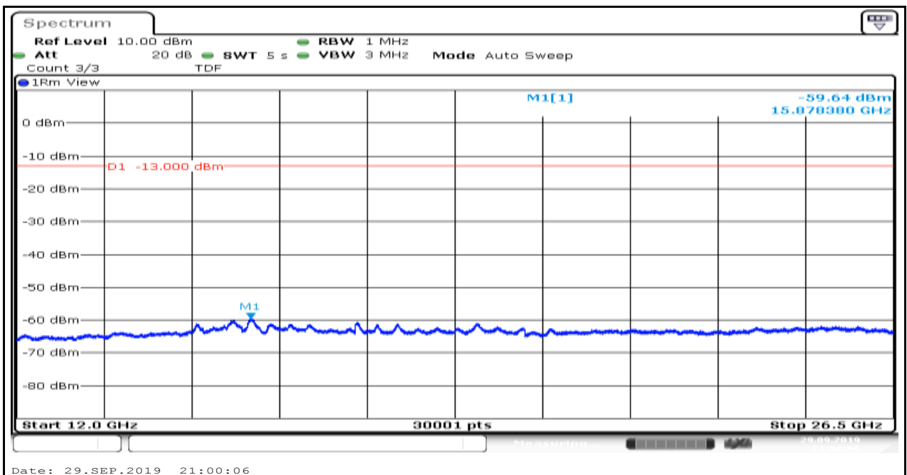
Band4_1.4MHz_16QAM_20175_6
