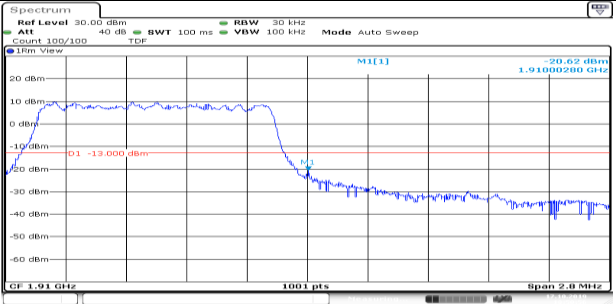
Band2_1.4MHz_16QAM_19193_6_0_Low
