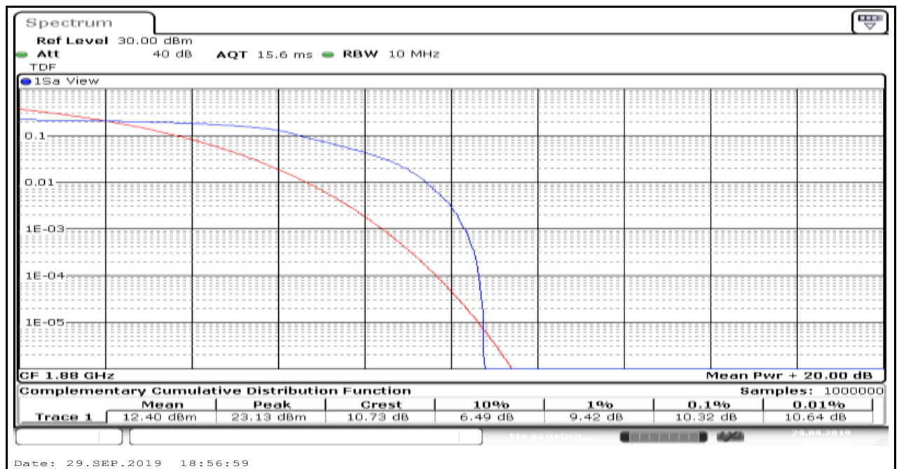
Band2_5MHz_16QAM_18900_6
