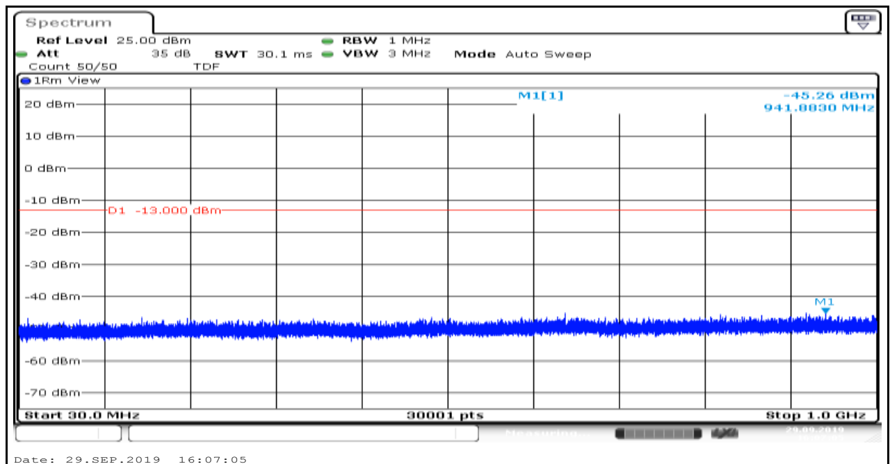
Band2_1.4MHz_16QAM_19193_6
