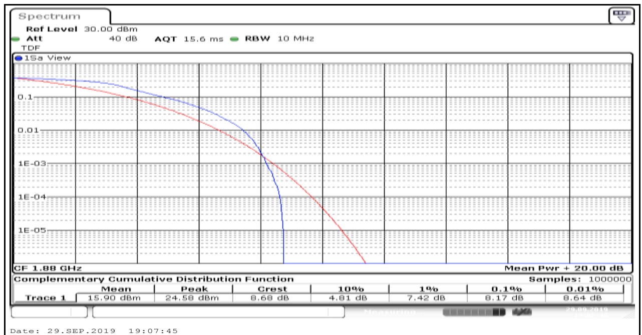
Band2_15MHz_16QAM_18900_6
