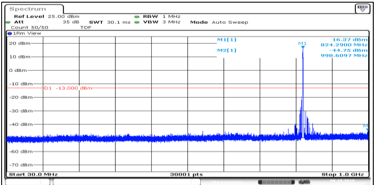
Band5_1.4MHz_QPSK_20407_6
