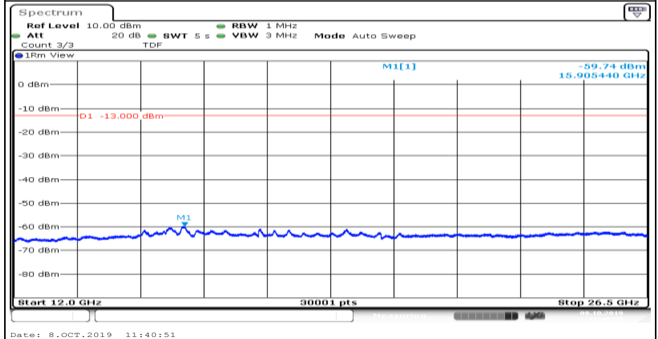
Band5_1.4MHz_QPSK_20525_1
