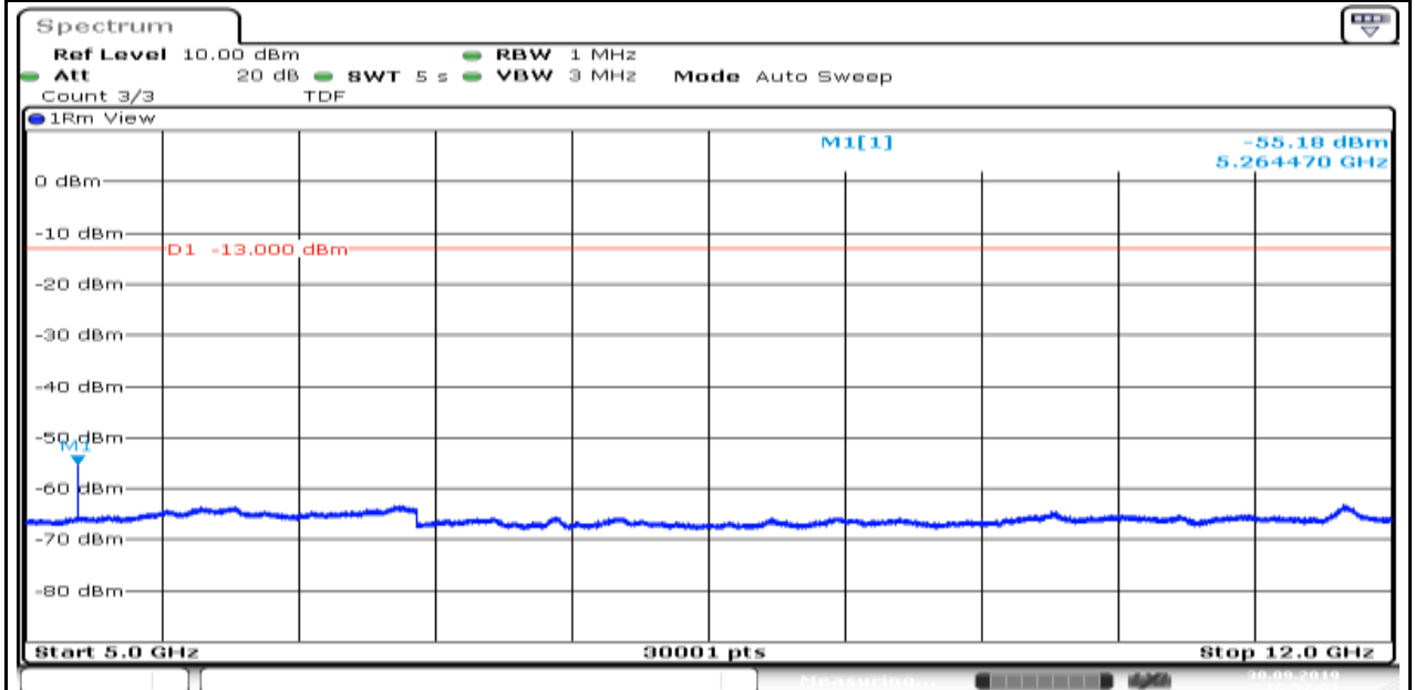
Band4_1.4MHz_16QAM_20393_1
