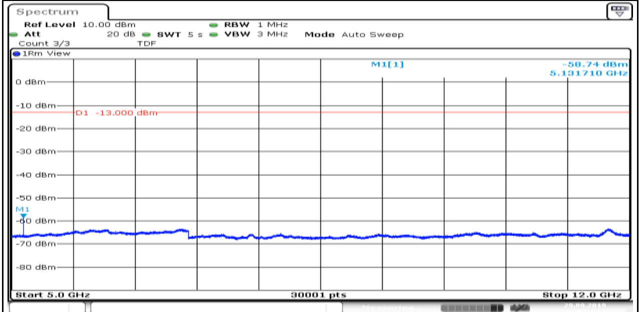
Band4_1.4MHz_QPSK_19957_6
