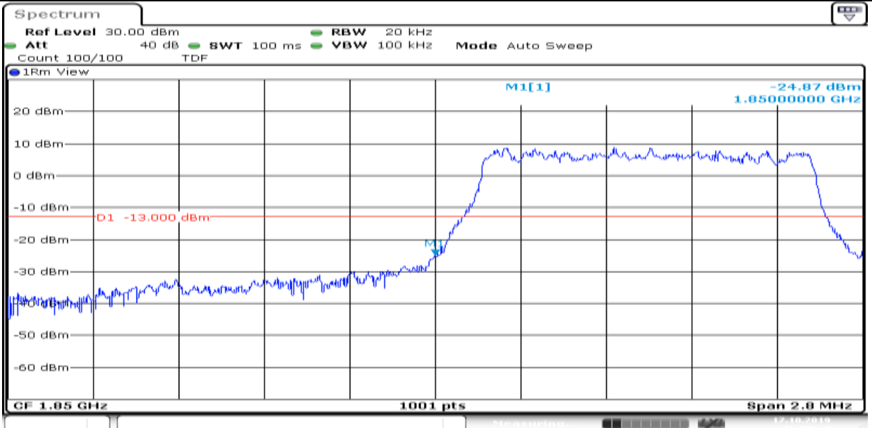
Band2_1.4MHz_16QAM_18607_6_0_Low
