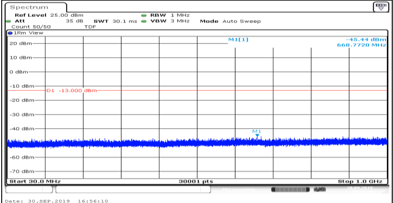
Band4_1.4MHz_16QAM_20393_1
