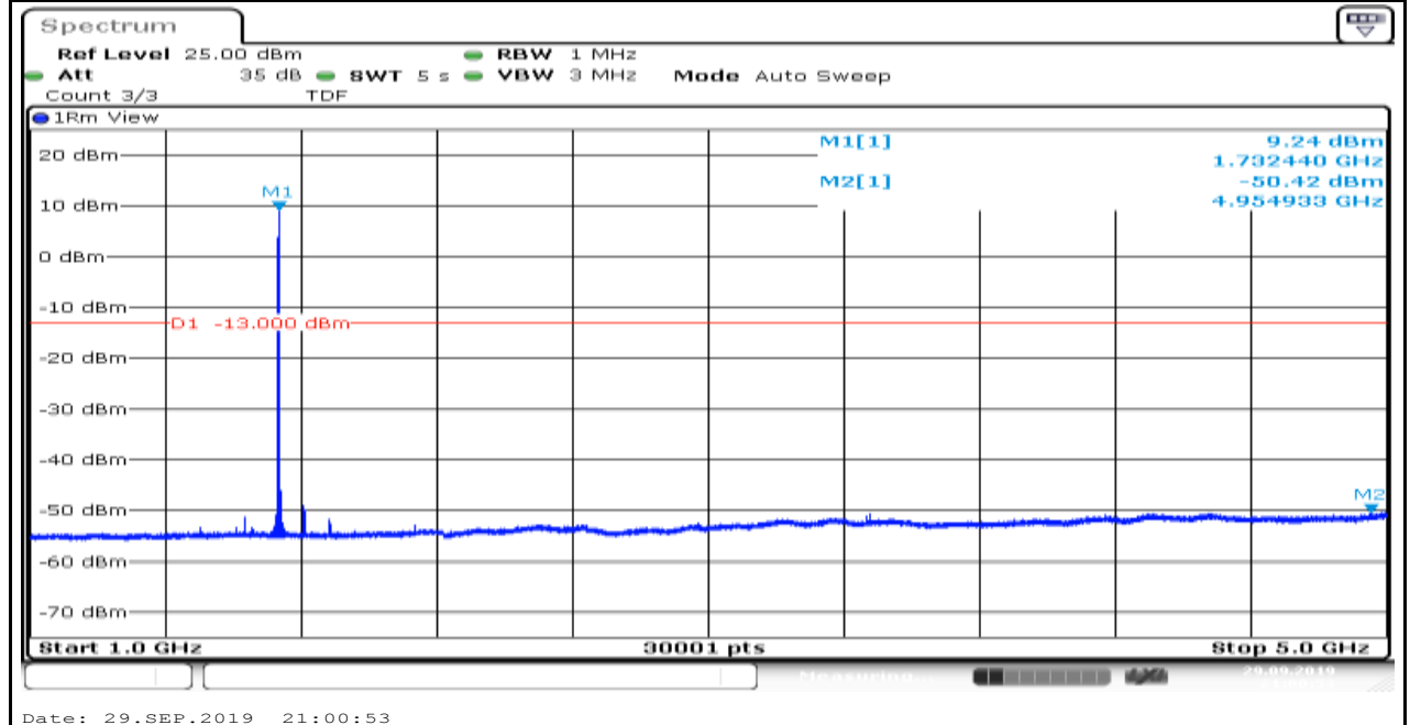
Band4_1.4MHz_QPSK_20175_6
