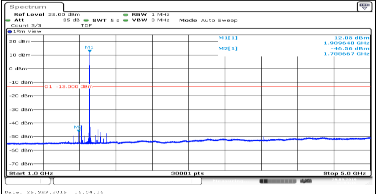
Band2_1.4MHz_16QAM_19193_1
