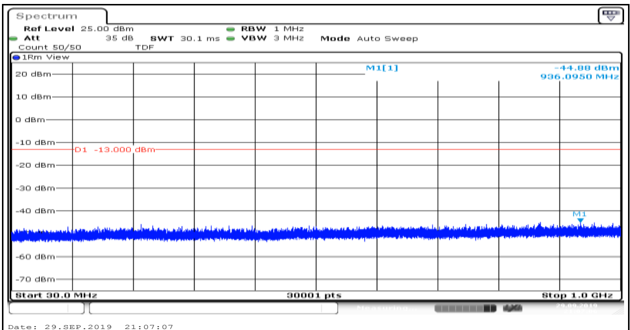
Band4_1.4MHz_QPSK_20393_5
