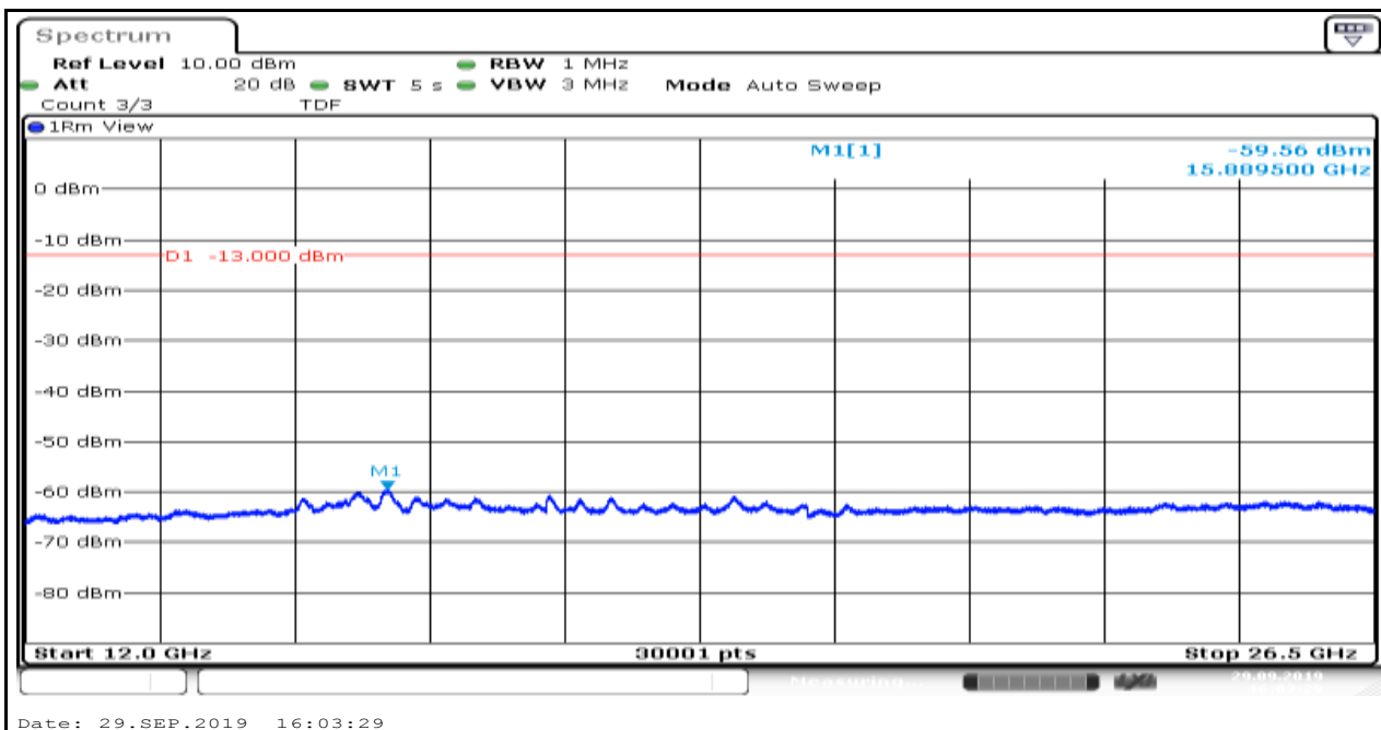
Band2_1.4MHz_QPSK_19193_6
