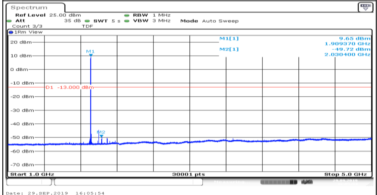
Band2_1.4MHz_QPSK_19193_1
