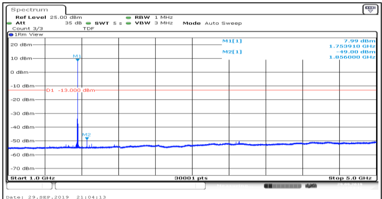
Band4_1.4MHz_QPSK_20393_5
