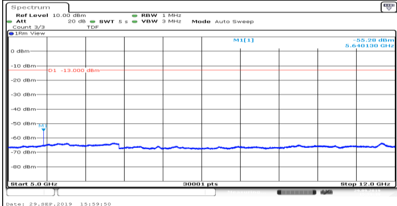
Band2_1.4MHz_QPSK_19193_1
