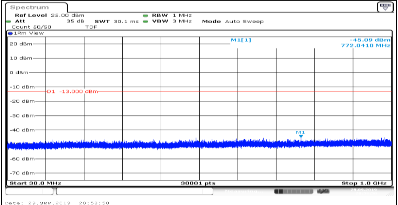
Band4_1.4MHz_16QAM_20175_6
