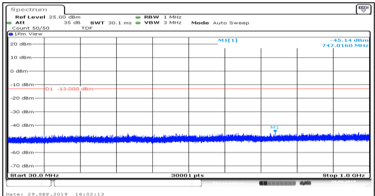
Band2_1.4MHz_QPSK_19193_1
