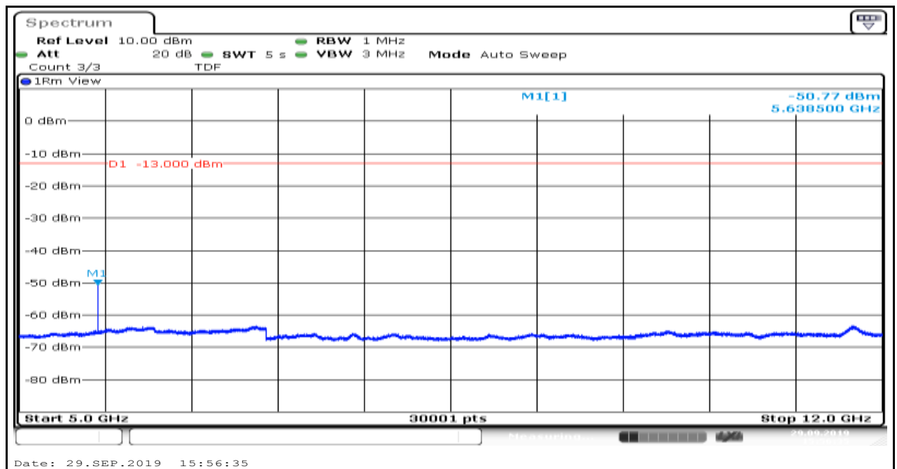
Band2_1.4MHz_QPSK_18900_1
