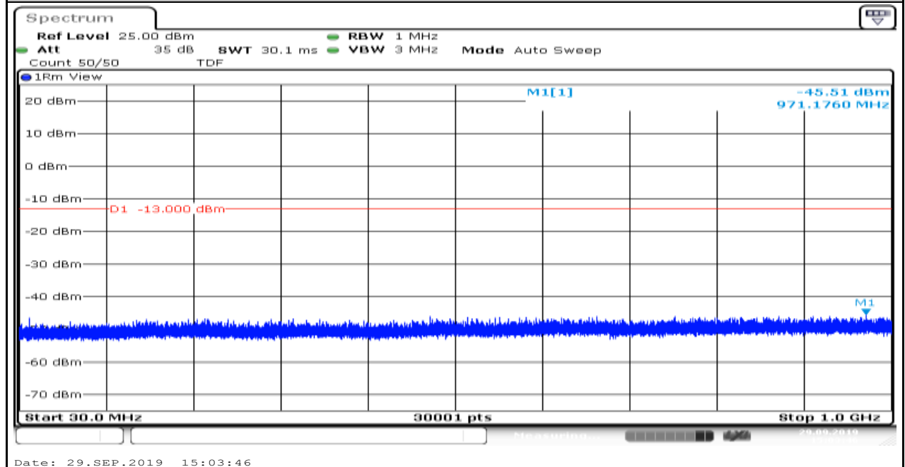
Band2_1.4MHz_QPSK_18900_1
