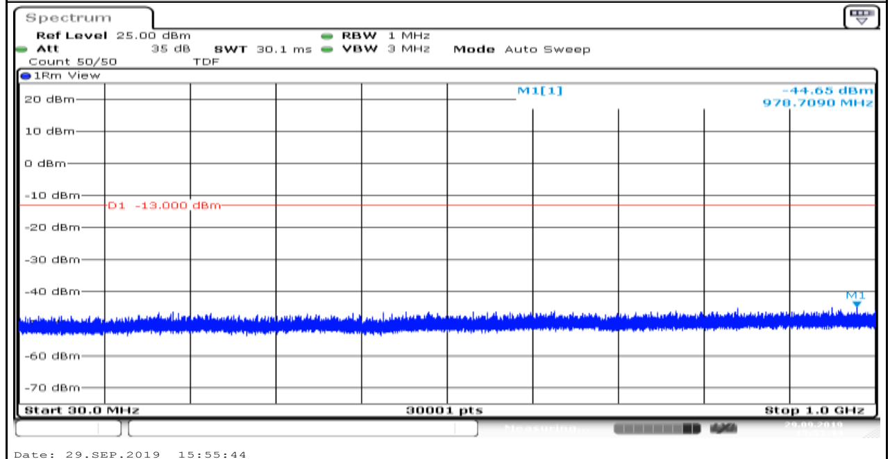
Band2_1.4MHz_QPSK_18900_6
