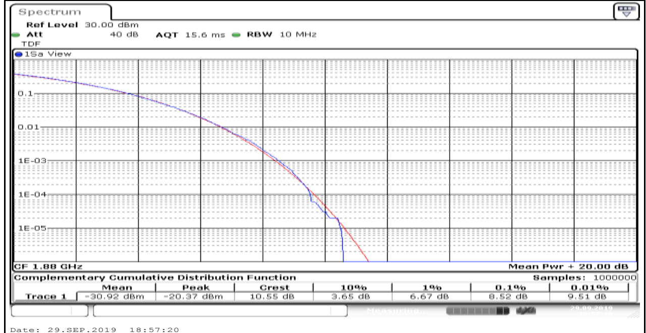
Band2_5MHz_QPSK_18900_6
