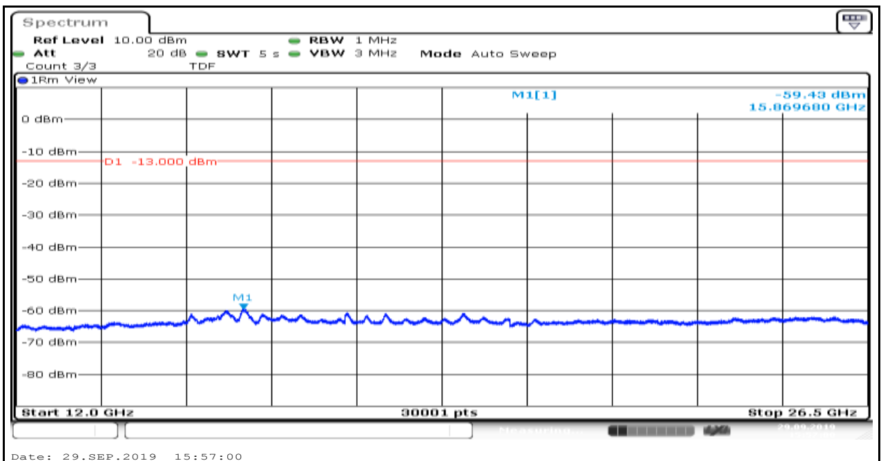
Band2_1.4MHz_QPSK_18900_1
