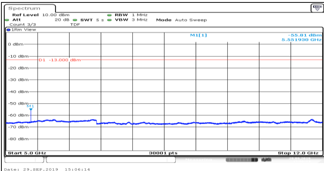
Band2_1.4MHz_16QAM_18607_6
