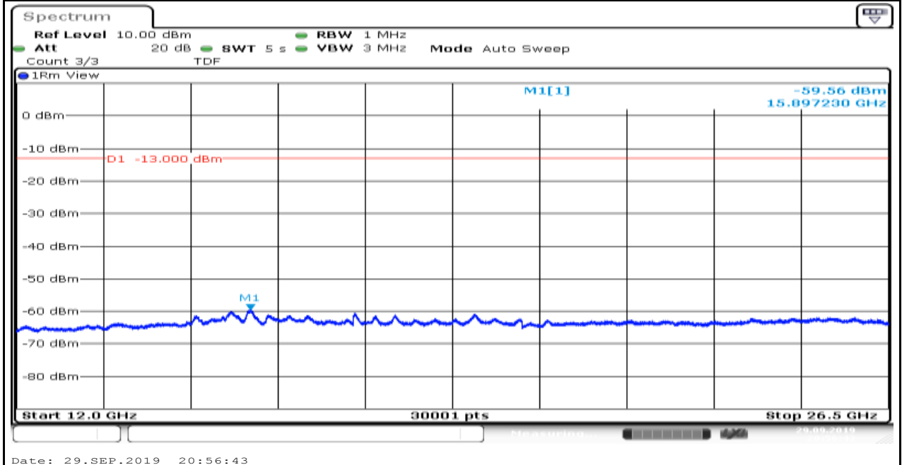
Band4_1.4MHz_16QAM_19957_1
