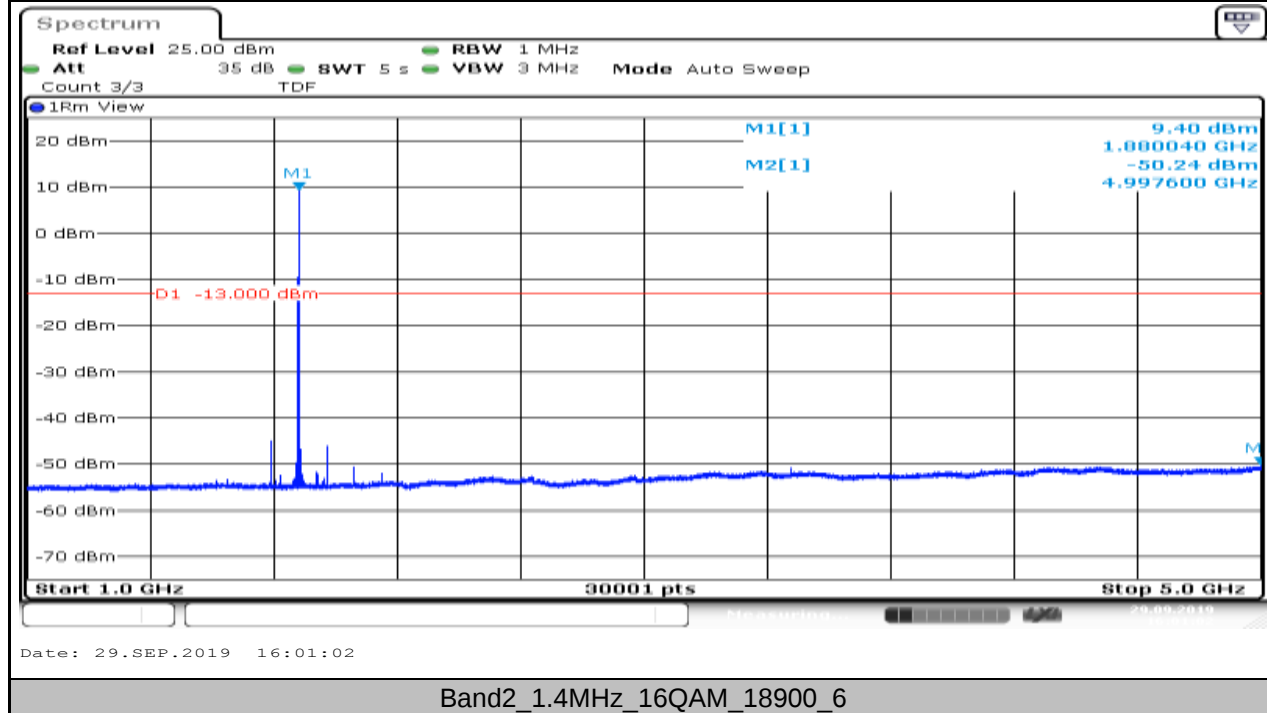
Band2_1.4MHz_16QAM_18900_6
