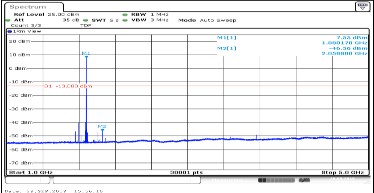
Band2_1.4MHz_QPSK_18900_1
