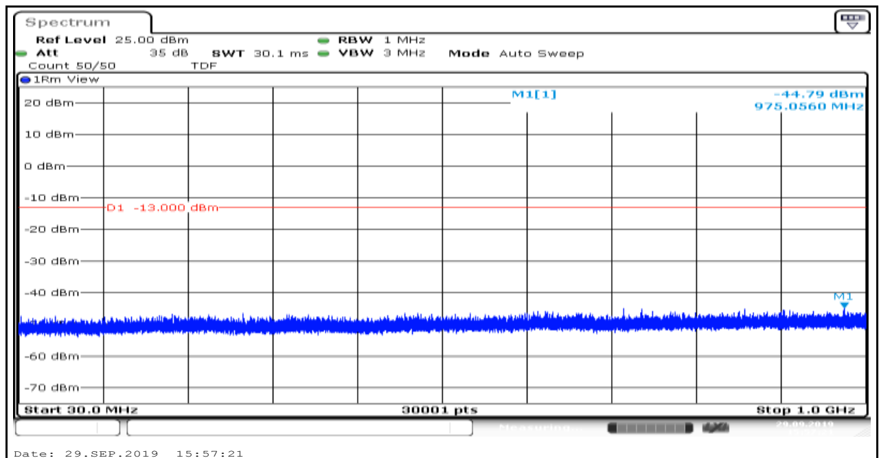
Band2_1.4MHz_16QAM_18900_6
