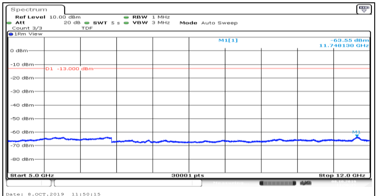
Band5_1.4MHz_QPSK_20407_6
