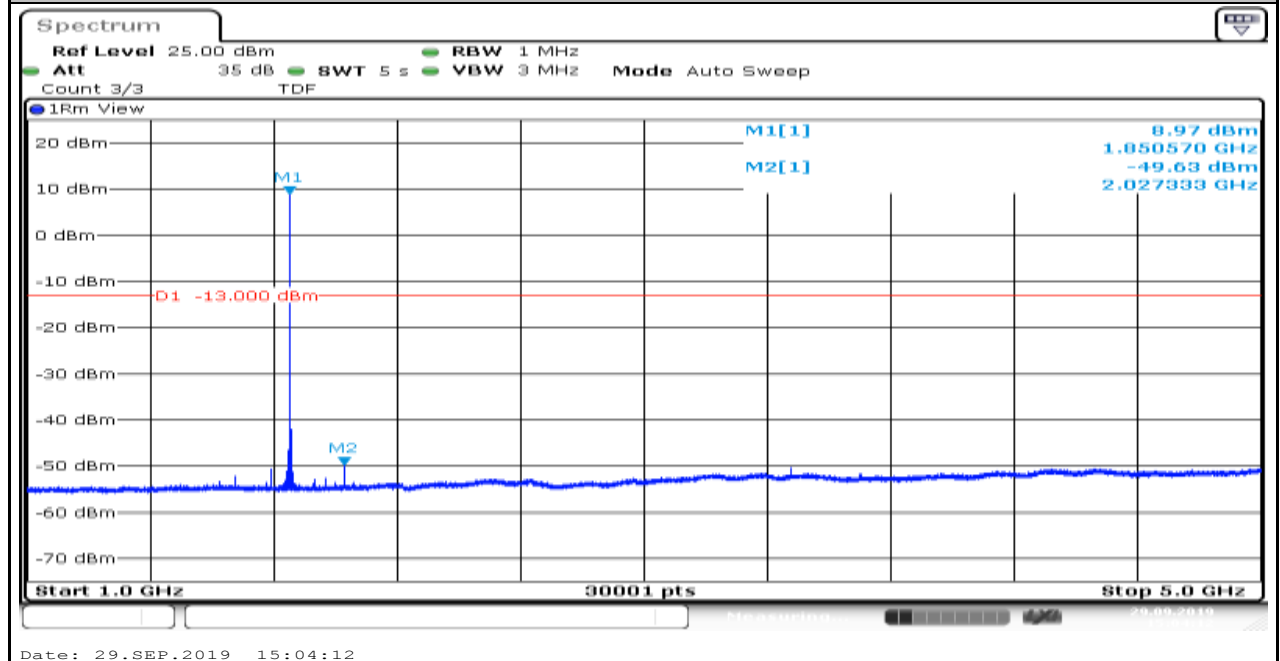
Band2_1.4MHz_QPSK_18607_6
