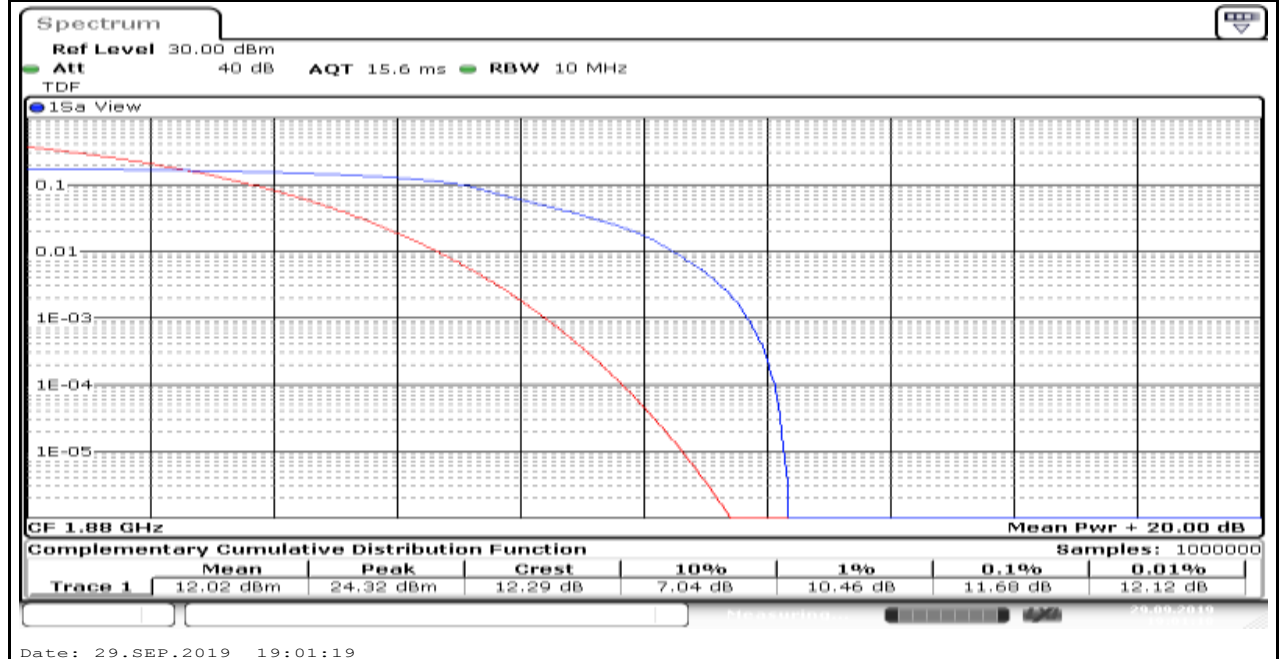
Band2_20MHz_16QAM_18900_6
