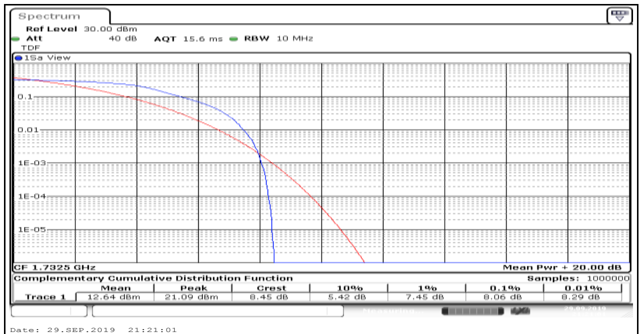
Band4_10MHz_16QAM_20175_6
