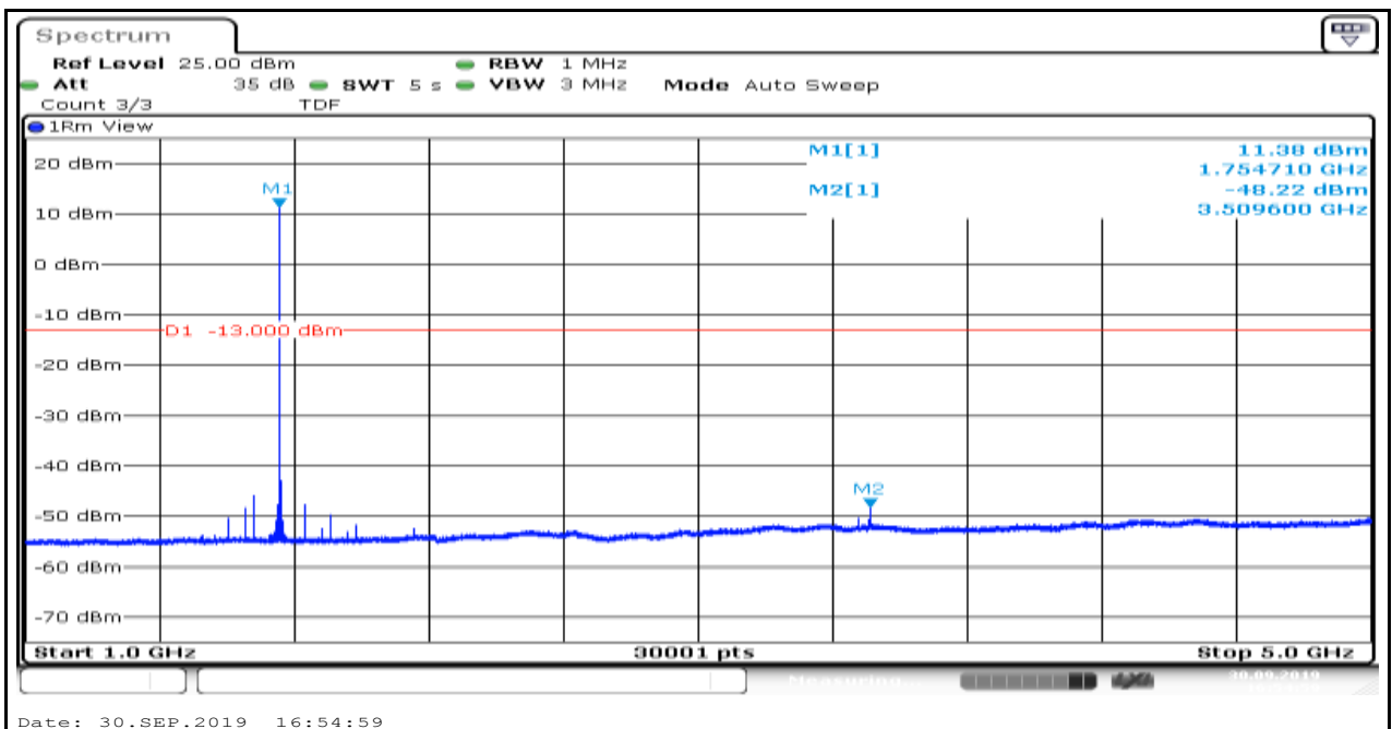
Band4_1.4MHz_QPSK_20393_1
