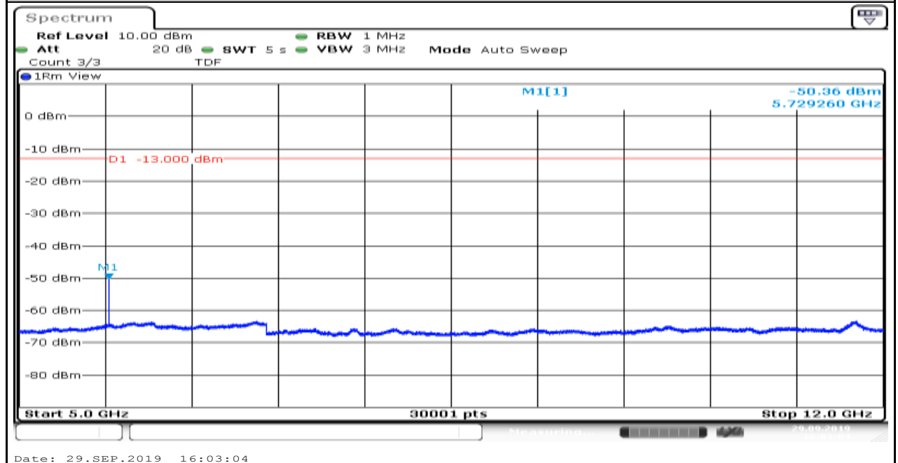
Band2_1.4MHz_16QAM_18607_6
