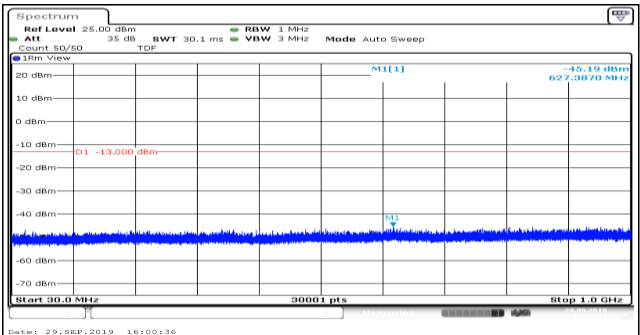
Band2_1.4MHz_16QAM_18900_1
