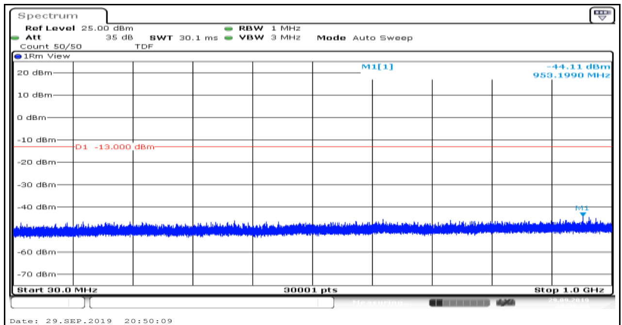
Band4_1.4MHz_QPSK_20175_6
