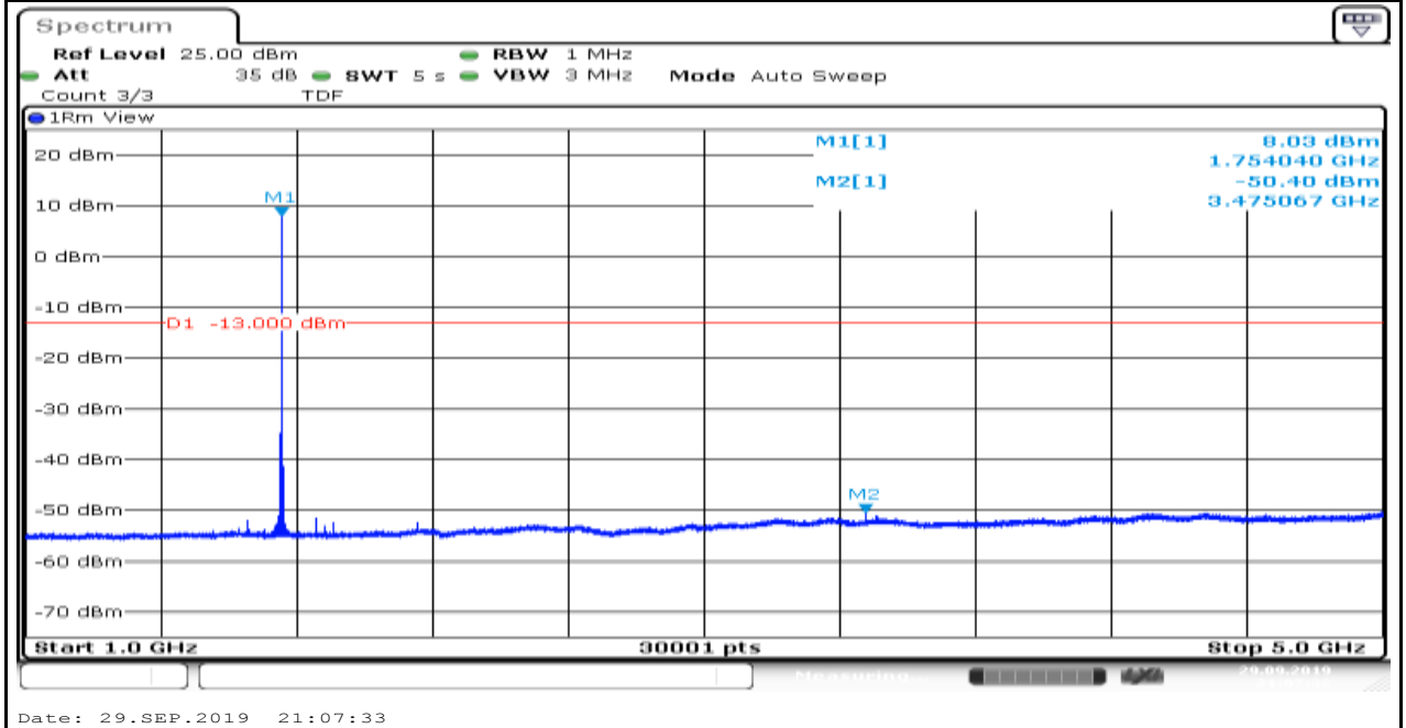
Band4_1.4MHz_QPSK_20393_6
