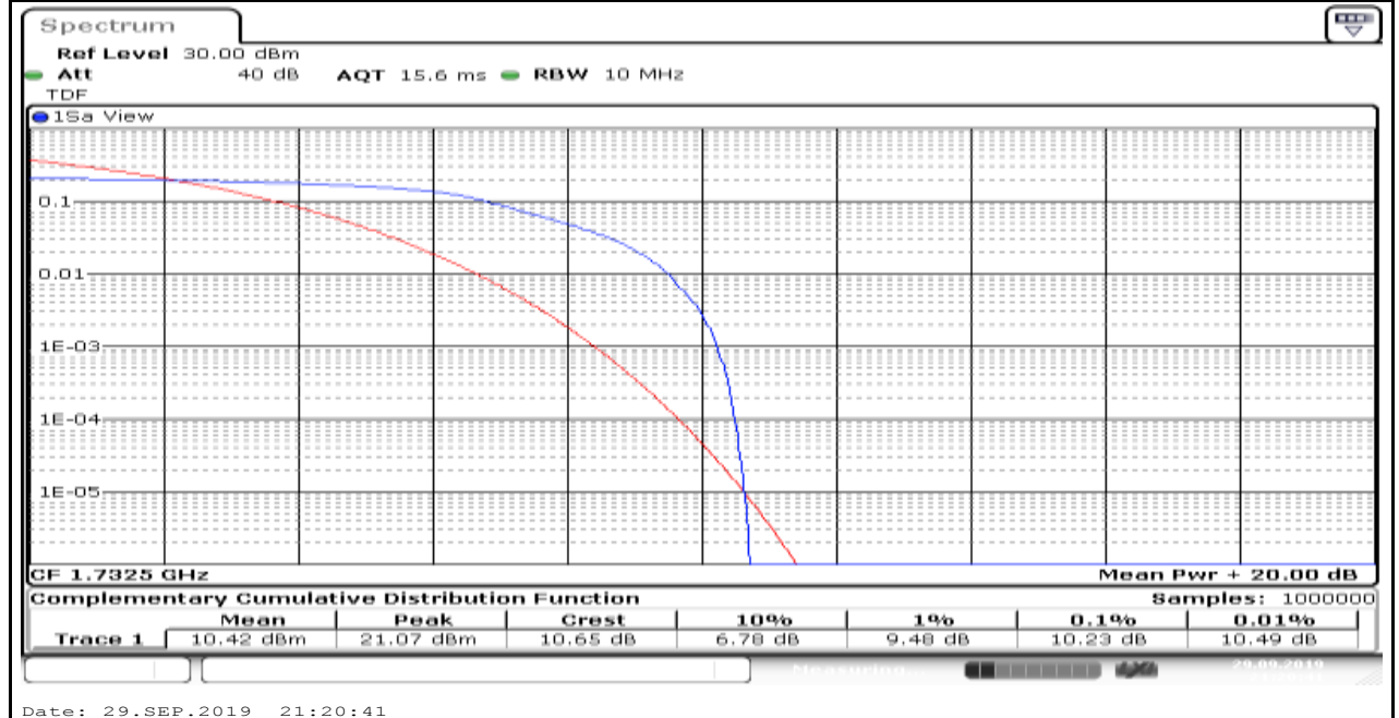
Band4_1.4MHz_16QAM_20175_6
