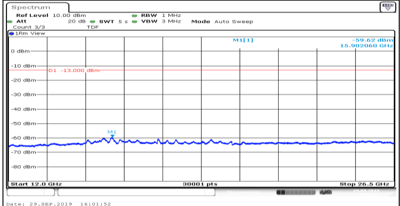
Band2_1.4MHz_16QAM_18900_6
