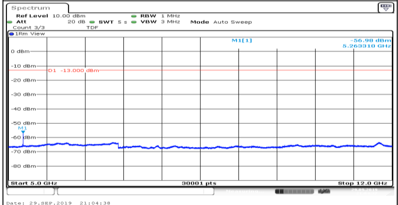
Band4_1.4MHz_QPSK_20393_5
