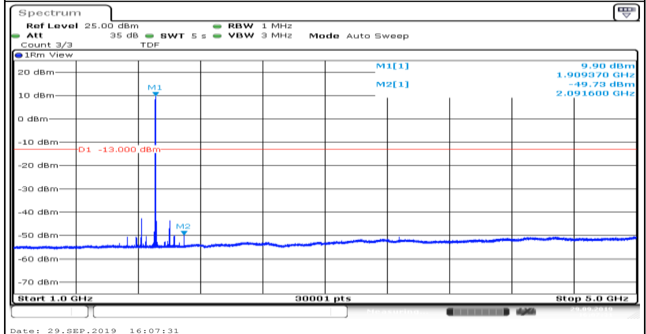
Band2_1.4MHz_16QAM_19193_6
