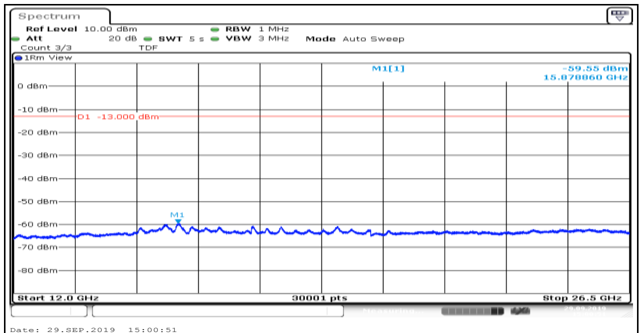
Band2_1.4MHz_QPSK_18607_6
