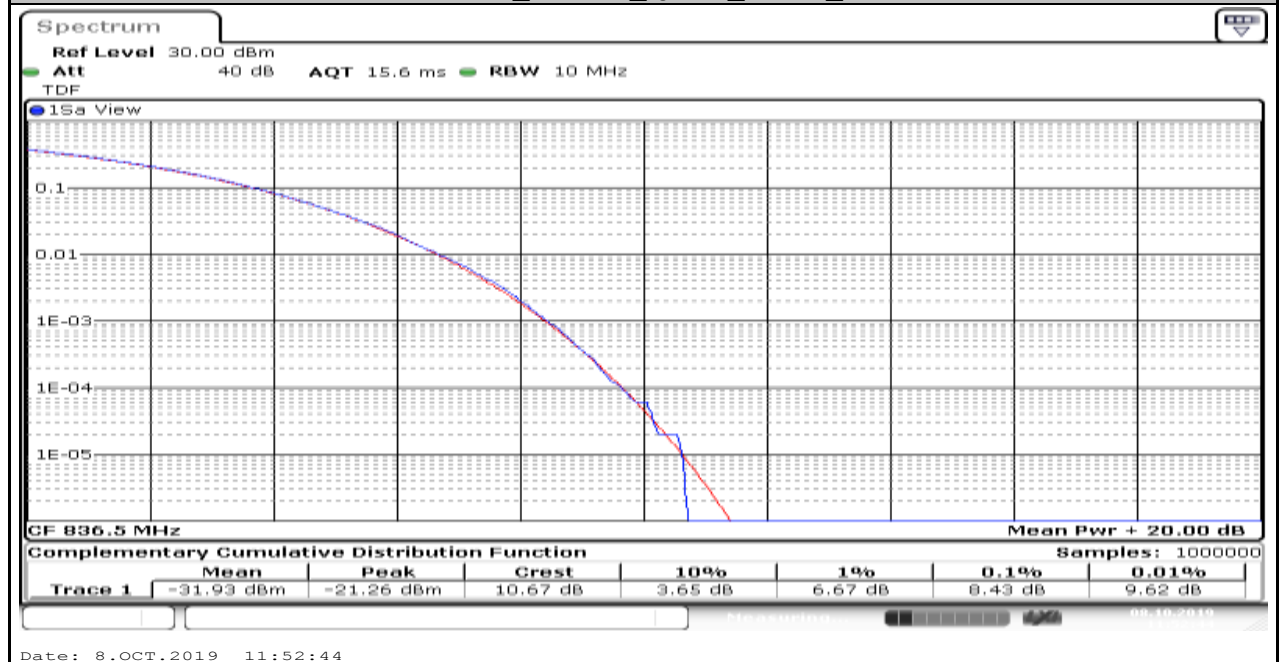
Band5_5MHz_16QAM_20525_6
