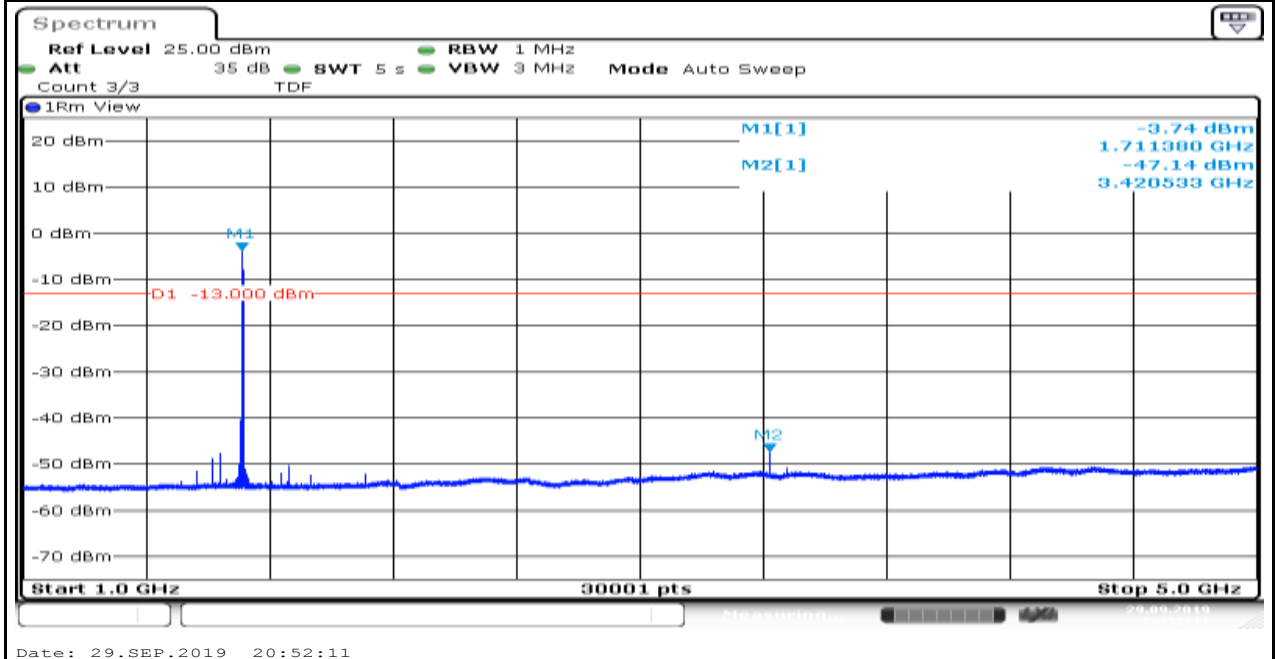
Band4_1.4MHz_16QAM_19957_6
