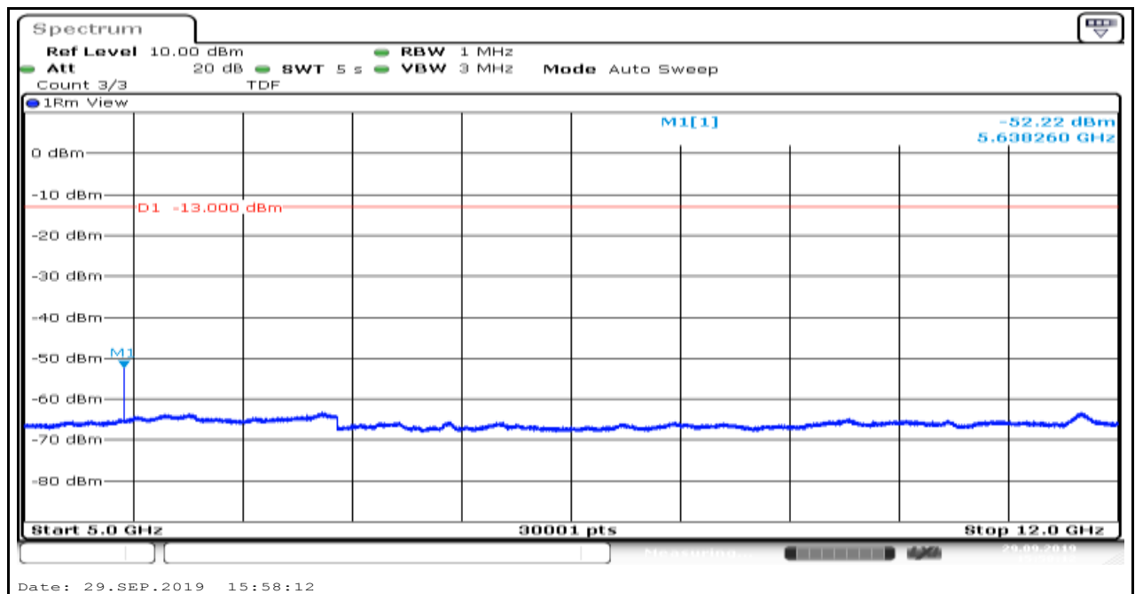
Band2_1.4MHz_16QAM_18900_1
