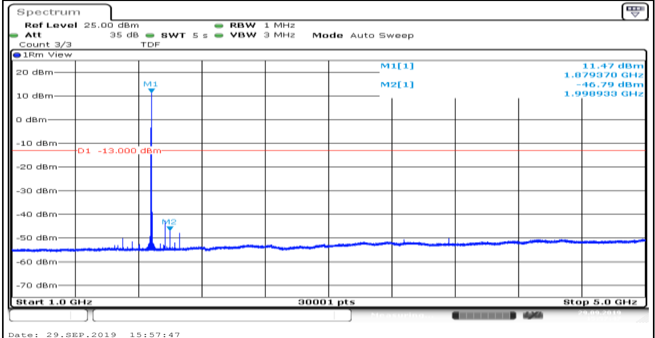
Band2_1.4MHz_16QAM_18900_1
