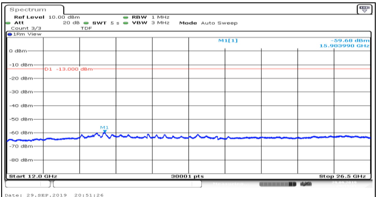
Band4_1.4MHz_QPSK_19957_6
