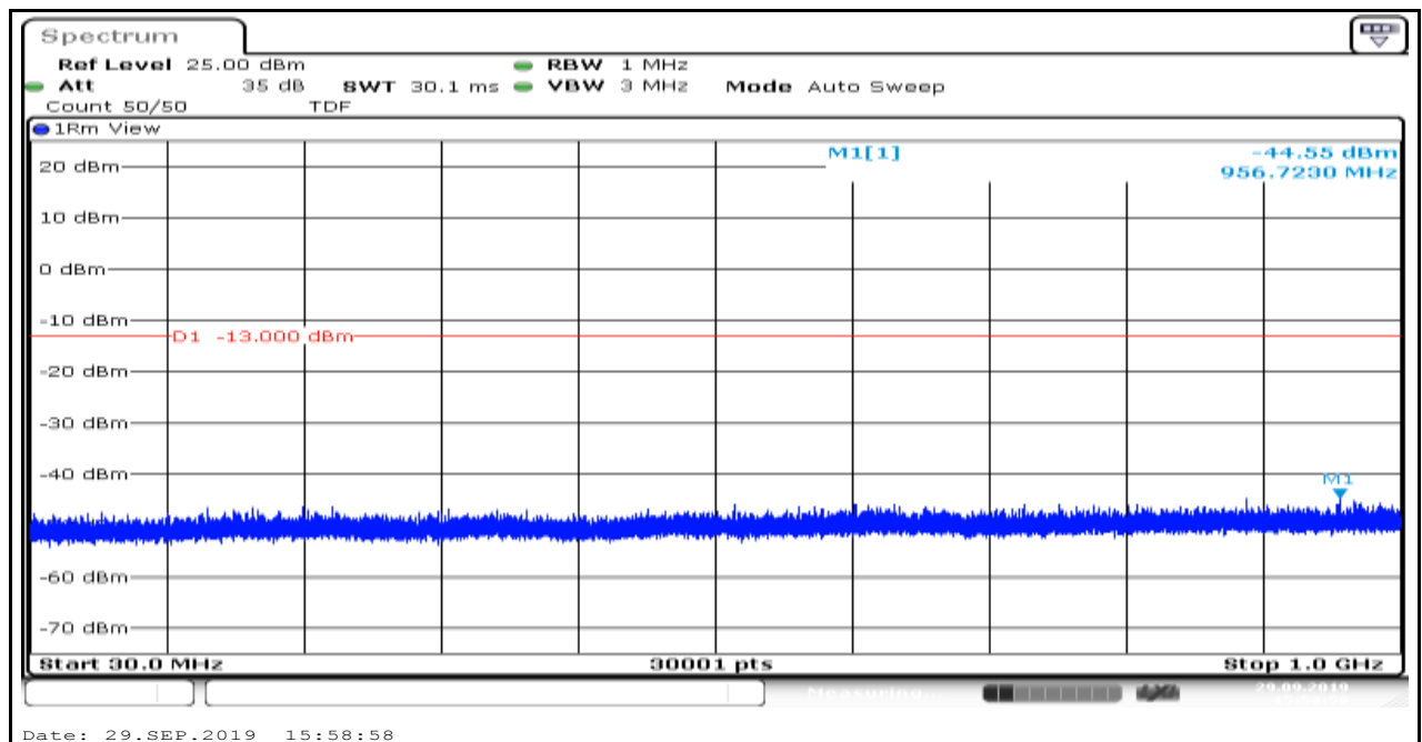
Band2_1.4MHz_QPSK_18900_6
