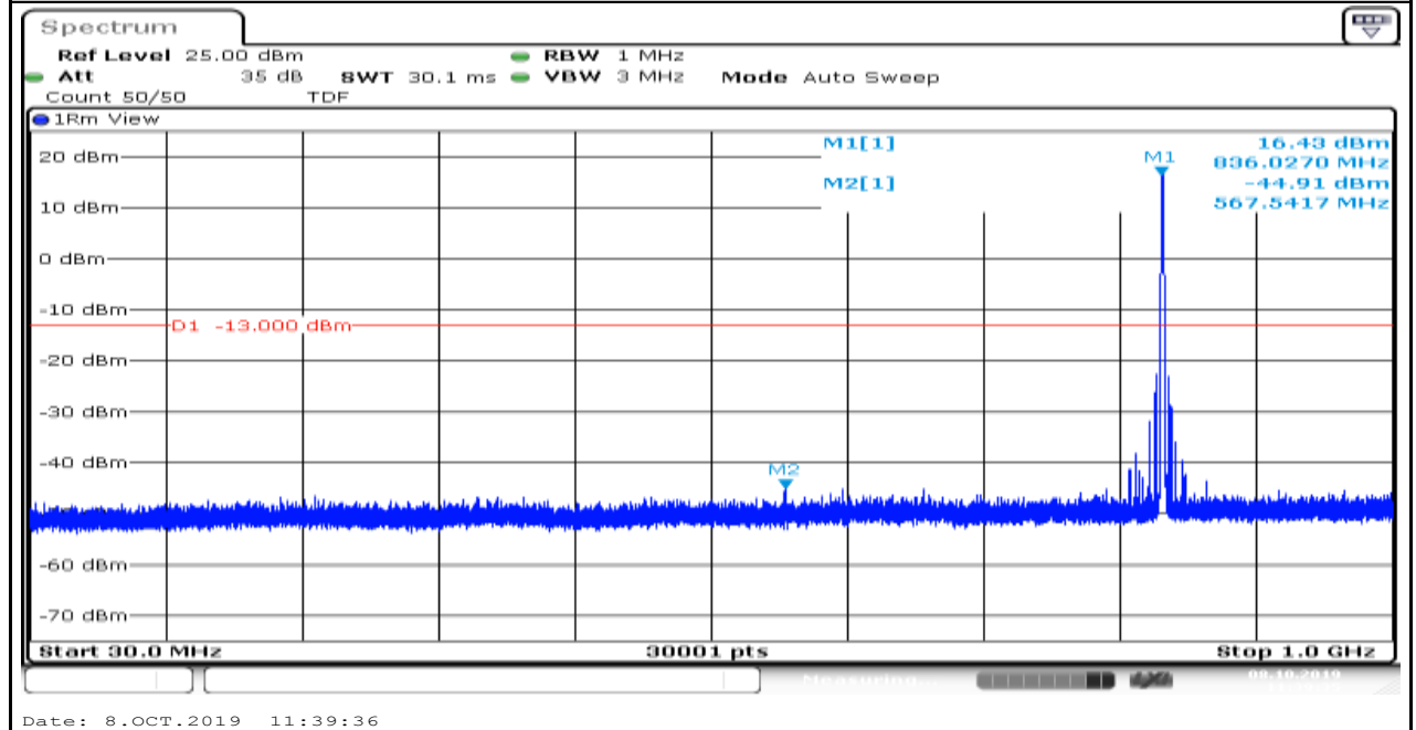
Band5_1.4MHz_QPSK_20525_6
