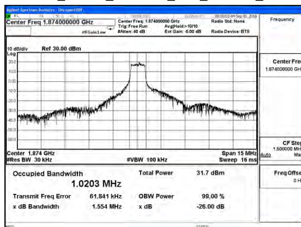
Cat M1_Band 2_CH18900_15M_16-QAM_5RB1
