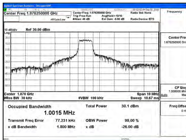
Cat M1_Band 2_CH18900_10M_16-QAM_5RB1
