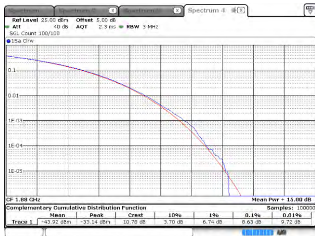
Cat M1_Band 2_CH18900_20M_QPSK_1RB0
