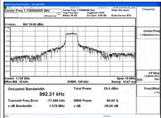
Cat M1_Band 4_CH20175_10M_16-QAM_5RB1
