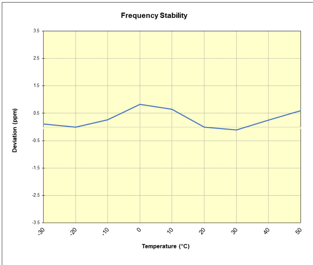
Plot 7-37. LTE Band 8 NB-IoT Frequency Stability Chart
