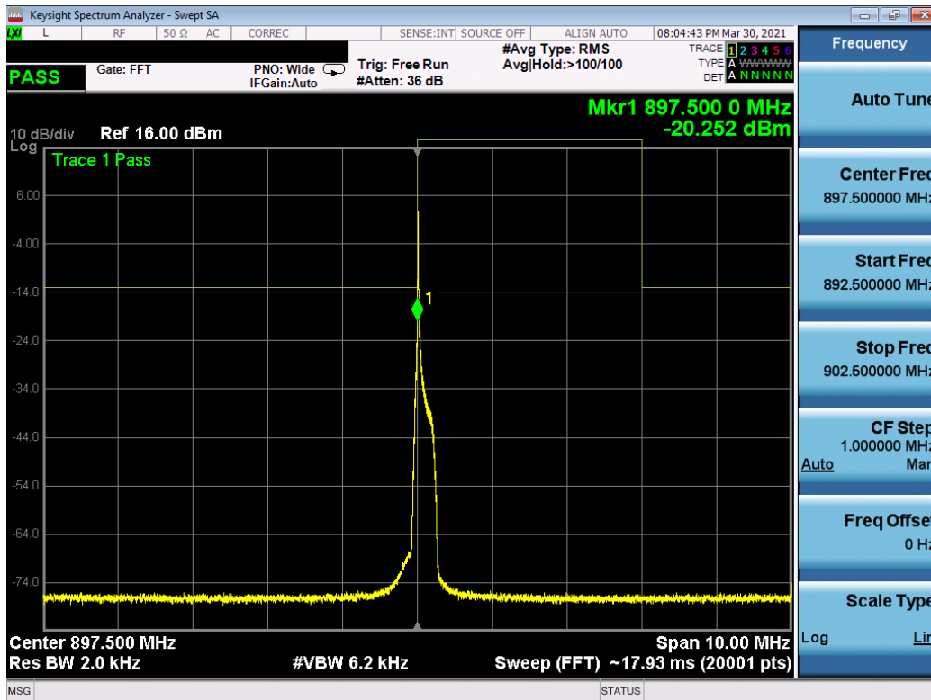
Plot 7-5. Lower Band Edge Plot (3.75kHz SCS, BPSK, 1SC, SC Offset 6, 2kHz RBW) _CH21626
