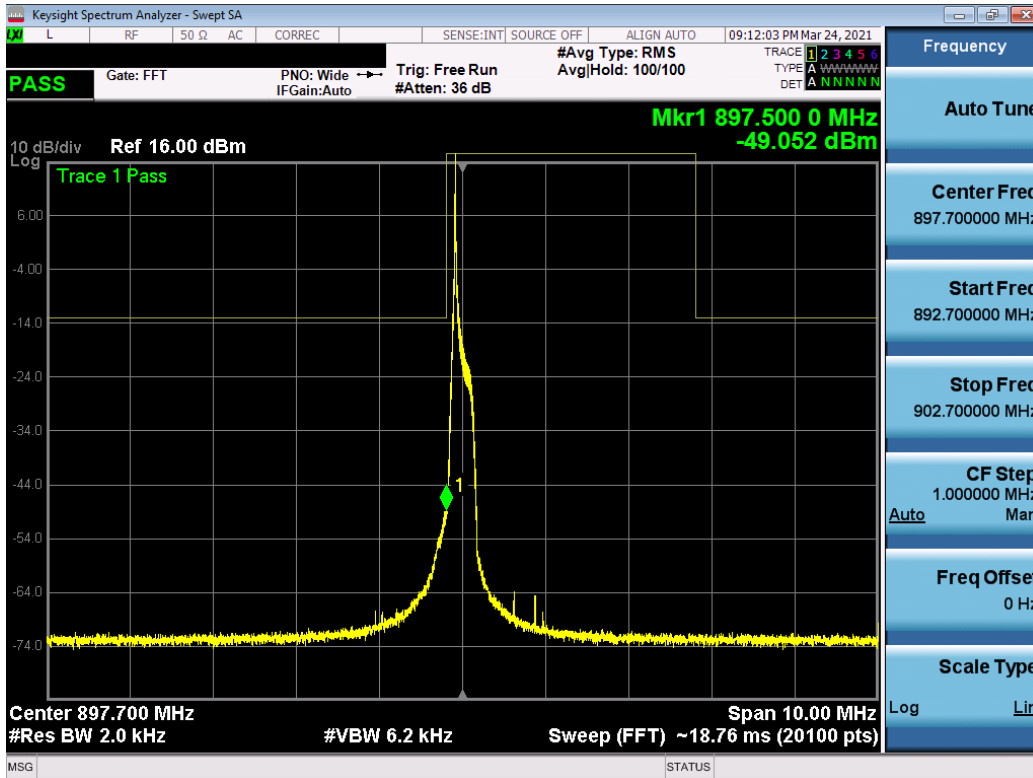
Plot 7-6. Lower Band Edge Plot (3.75kHz SCS, BPSK, 1SC, SC Offset 6, 2kHz RBW) _CH21627
