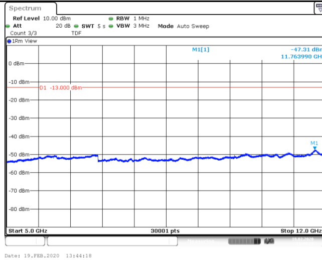
Band26_Stand-Alone_NaN_BPSK_26691_1@11_15kHz_30_1000_30~1000MHz@-34.71dBm_-13_PASS_
