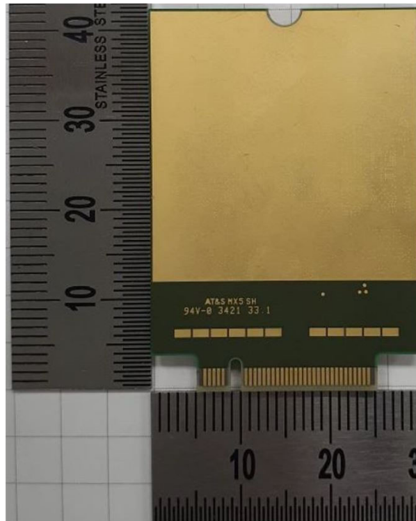
Back View of EUT_LN920A12-WW
