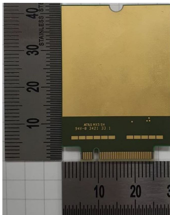
Back View of EUT_ LN920A6-WW
