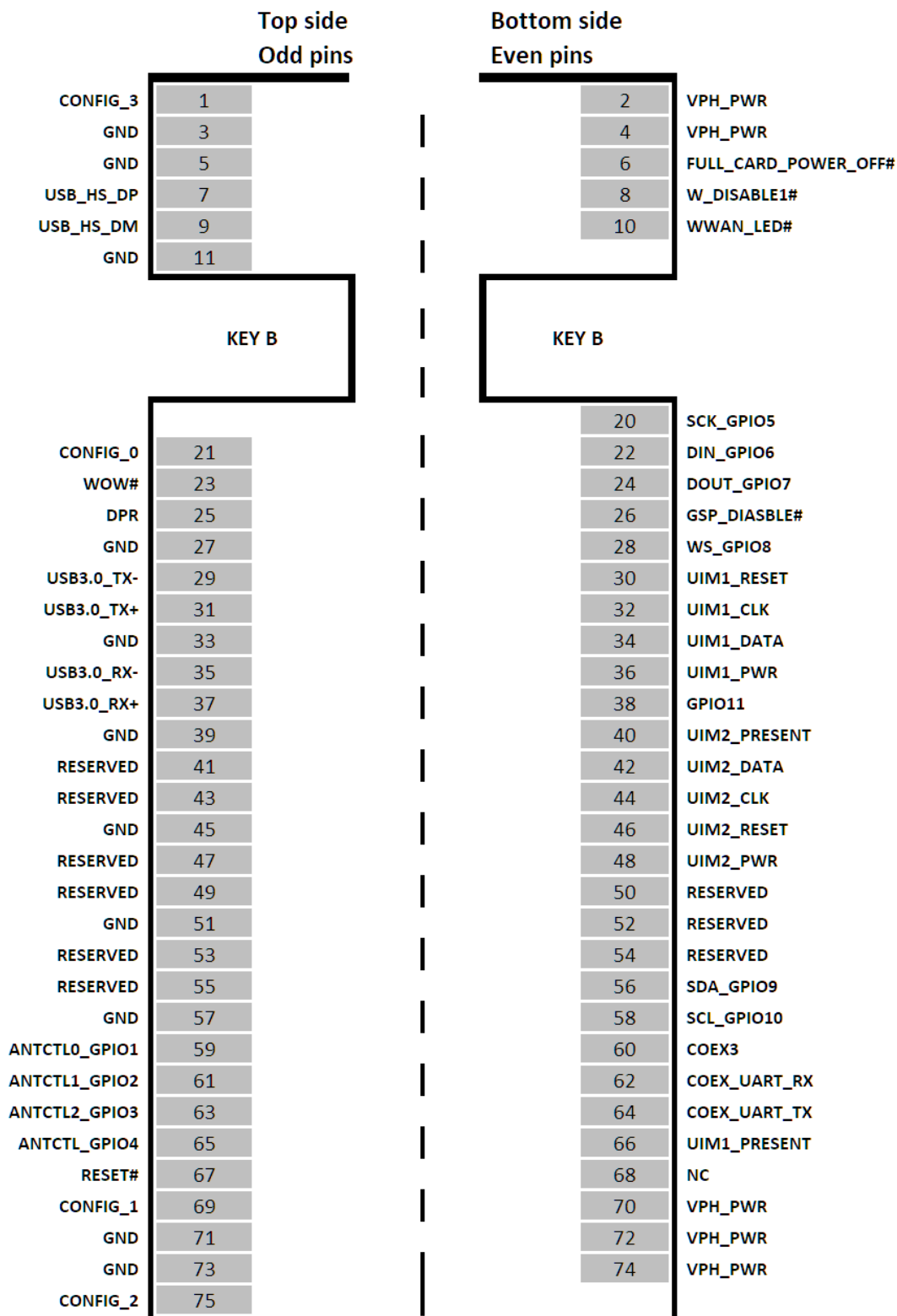
Figure 2: LN920 Pin-out
