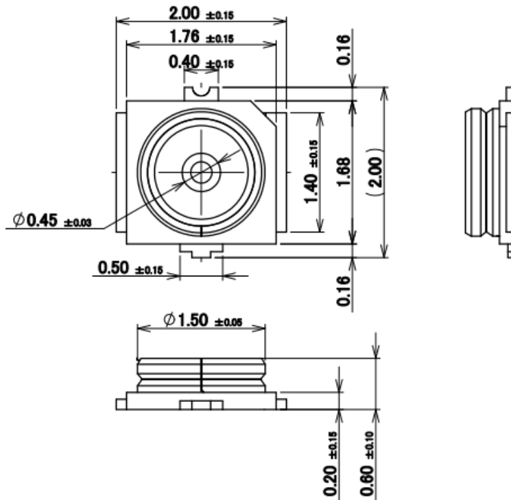
Figure 4: MHF-4 RF connector
